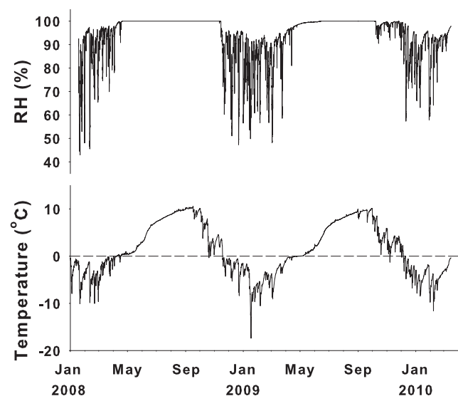
Figure 5 Per cent relative humidity (RH) and ambient air temperature measured hourly in the ice mine talus cave over a two-year period of time.
