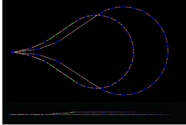
Figure 3a: Top and side views of a G4beamline model of the RLA I arcs#1 (1.2 GeV) and #3 (2.4 GeV).
