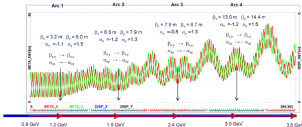
Figure 2b. Beta beating in the RLA I linac for all passes.
