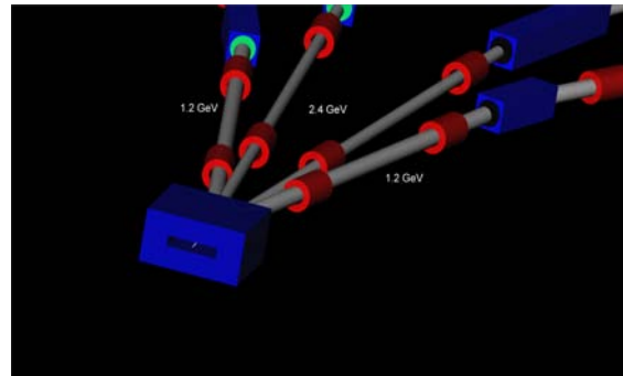
Figure 4. G4beamline model of RLA I switchyard for arc#1 and #3.
