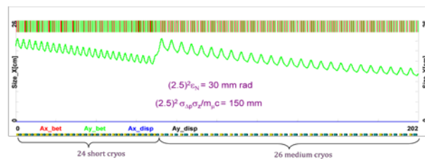
Figure 1c: OptiM model of the prelinac.
