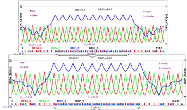
Figure 3b: OptiM model of RLA I arc #1 and #3.
