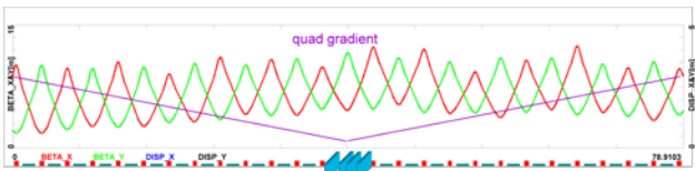
Figure 2a. Increasing quadrupole strength with distance to center of linac and 1 st whole pass beta functions.
