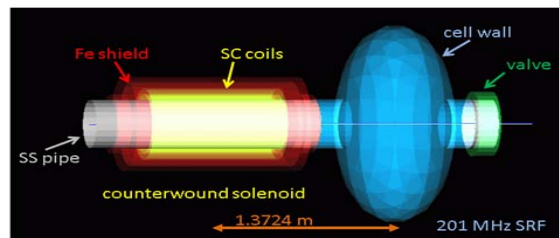
Figure 1a: G4beamline model of a 3m prelinac cryomodule.
