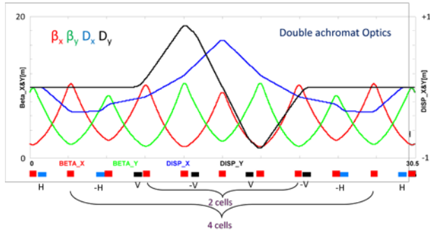
Figure 2b: OptiM model of the prelinac to RLA I chicane.
