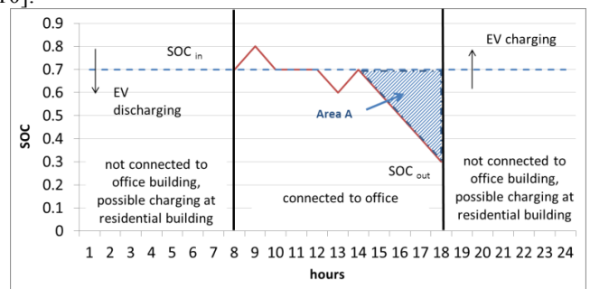
Fig. 3. Hypothetical charging/discharging at a commercial (office) building. SOC in means mobile storage state of charge at the time when the EV connects to the building, SOC out means state of charge at the time when the EV disconnects from the building.
