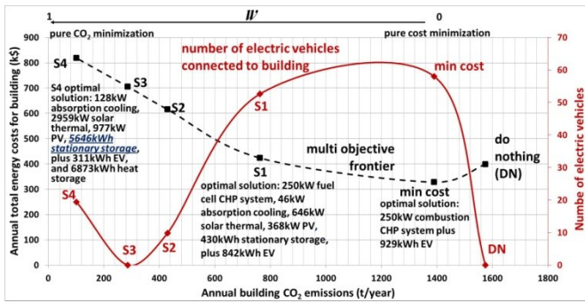
Fig. 5. Multi-objective frontier for the healthcare facility in FCZ13 (SDG&E) and connected S2 EVs.
