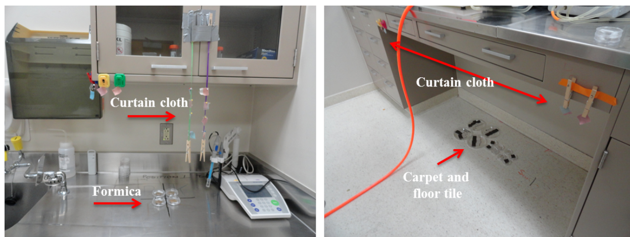
Figure 4.7. Arrangement of the Coupons in the Test Room
