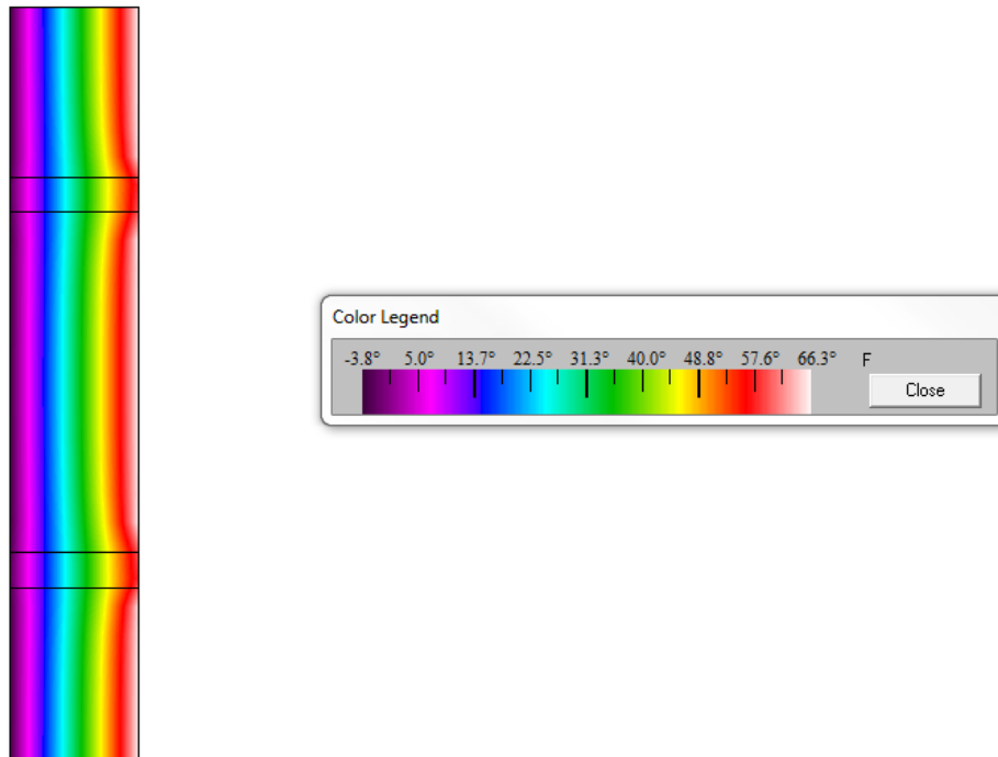
Figure 4. Modeled thermal resistance of PU foam sprayed into studs 2 × 6; 16 in. o.c. The effective thermal resistance of 5.5 in. PU foam is R-25 (excluding air film resistances). To reach target R-35, it was assumed that the studs are installed on the exterior and standing off 2 in. away from the exterior sheeting. The 2 in. gap is filled with PU spray foam and collectively with the 5.5 in. stud spaces provides the required target R-value. Therefore, approximately 7.5 in. PU foam is required to reach target R-35.
