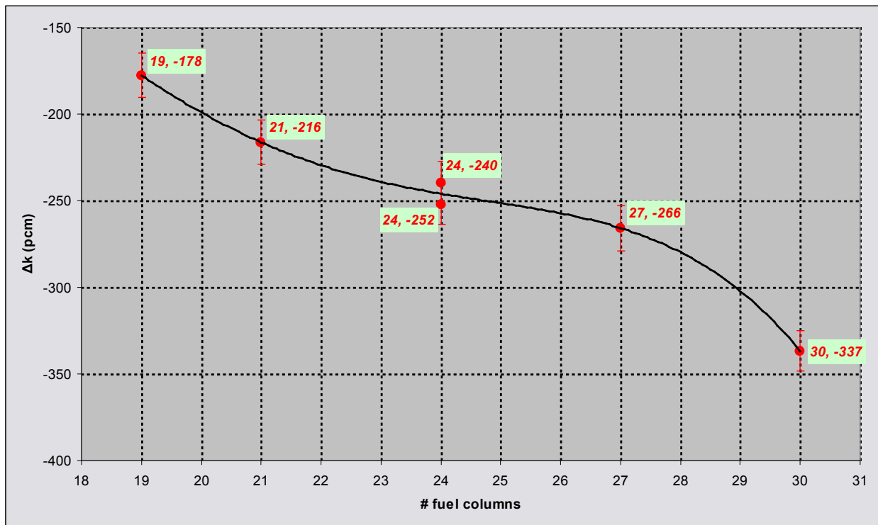
Fig. 3.18. Difference in k_{\text{eff}} calculated with the SCALE MG and CE models.
