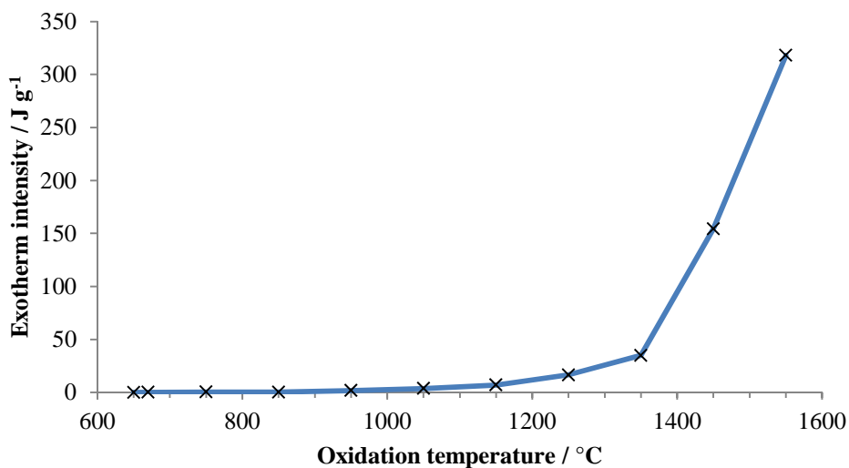
Figure 4. Measured DSC peak intensity upon first exposure of Al foil to air versus temperature of exposure.
