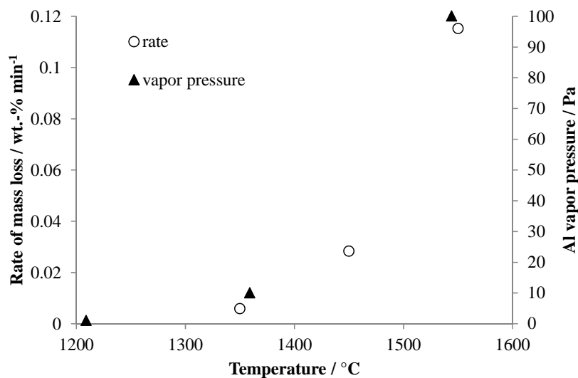
Figure 6. Rates of mass loss during Al evaporation taken from Figure 5 compared to the vapor pressure of Al at similar temperatures. The Al vapor pressure data was taken from http://www.knowledgedoor.com/2/elements_handbook/vapor_pressure.html .
