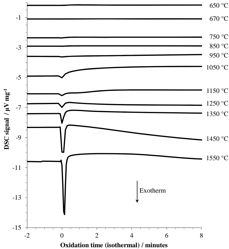
Figure 3. DSC results for Al foil heated under argon to the indicated temperature, then exposed to air (at t = 0 ).
