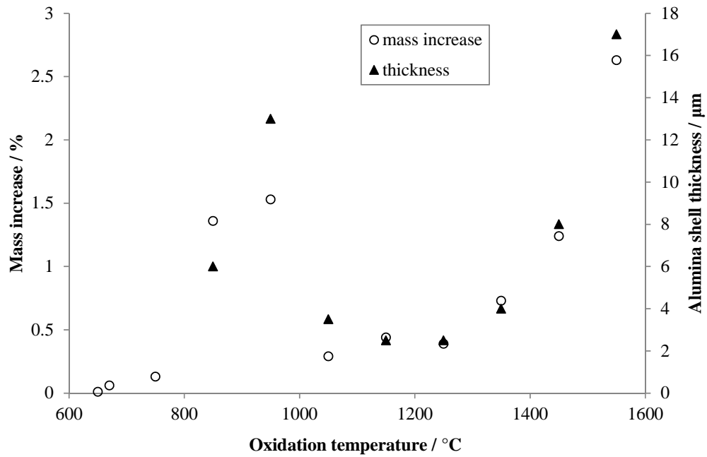
Figure 8. Thicknesses of the alumina shells estimated from the images shown in Figure 7 (filled triangles), and total mass gain during oxidation for each specimen recorded by TGA (open circles).
