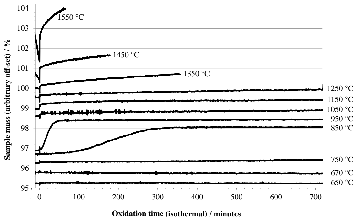
Figure 2. TGA results for Al foil heated under argon to the indicated temperature, then exposed to air (at t = 0 ).
