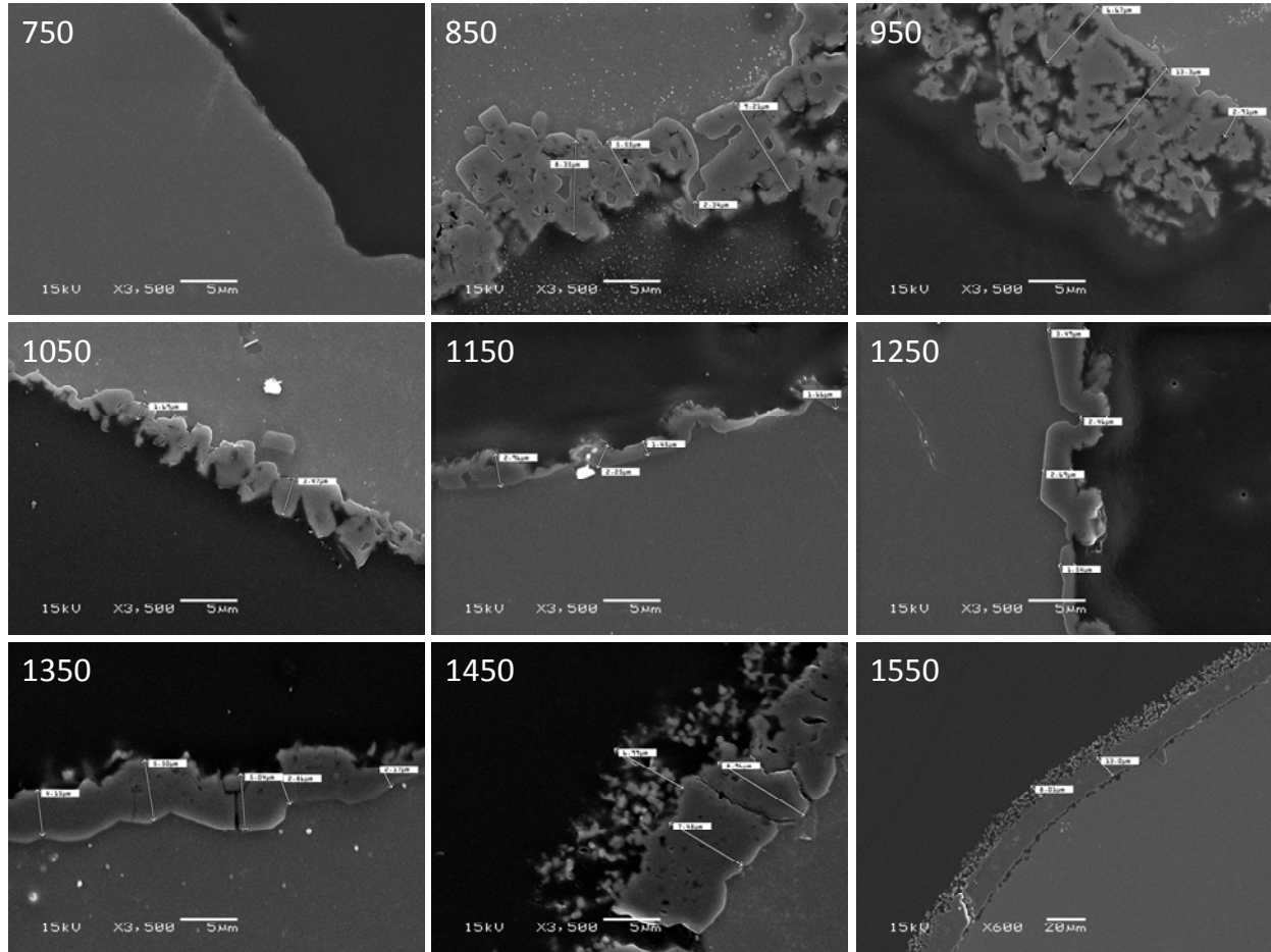
Figure 7. SEM images of cross sections of Al foil specimens after oxidation in air at the indicated temperature (in °C). Note that all images are shown at the same magnification (scale bar = 5 µm), except for that of the specimen oxidized at 1550 °C (scale bar = 20 µm).
