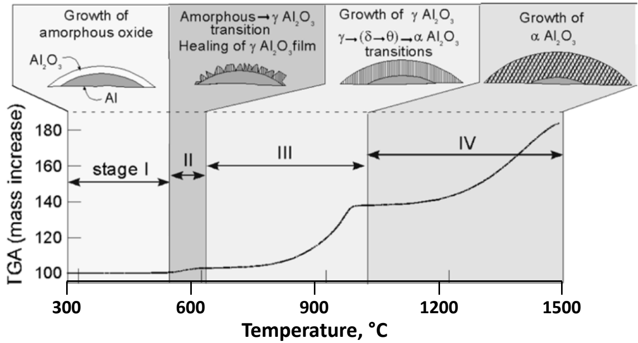
Figure 1. Schematic representation of transitions occurring in alumina layer on aluminum metal, and the temperature ranges in which they occur, superimposed on a typical TGA plot. Figure adapted from reference 7.
