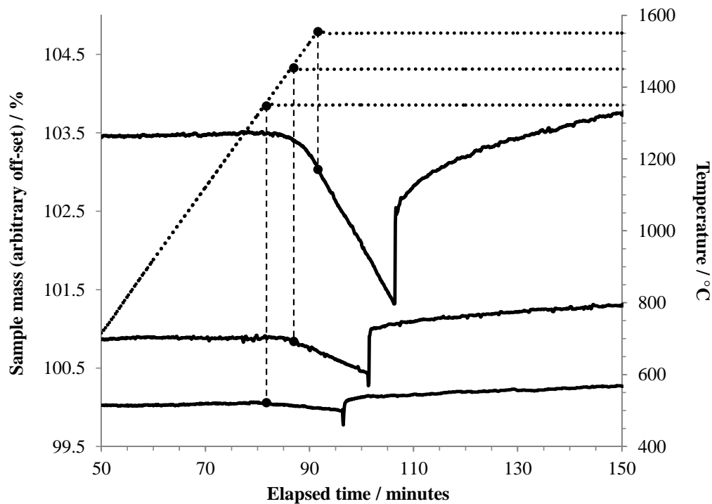
Figure 5. TGA results for Al foil heated to 1350 °C or higher under argon, held at that temperature for 15 minutes, then exposed to air. The vertical dashed lines tie the respective TGA curves to the point on the temperature curve (dotted line) where the isothermal hold began. In this plot, the beginning of the experiment is taken as t = 0 .
