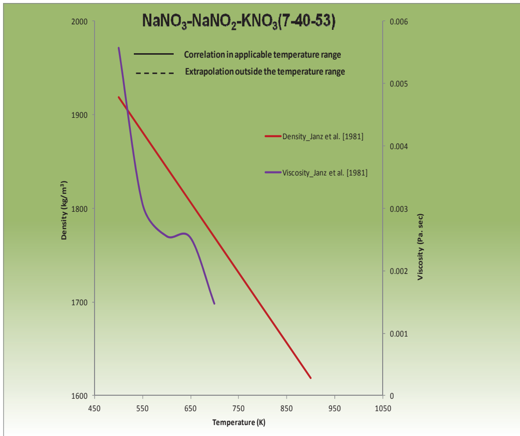
Figure 2.10. Plots of density and viscosity correlations for nitrate salts.
