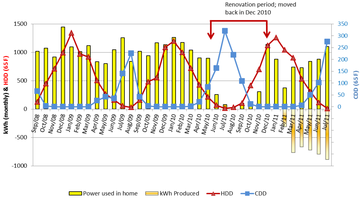
Figure 38. Graph of electricity use and PV generation of the Quincy Bungalow
