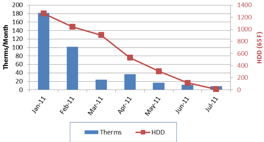
Figure 39. Graph of natural gas use following the Quincy Bungalow DER
