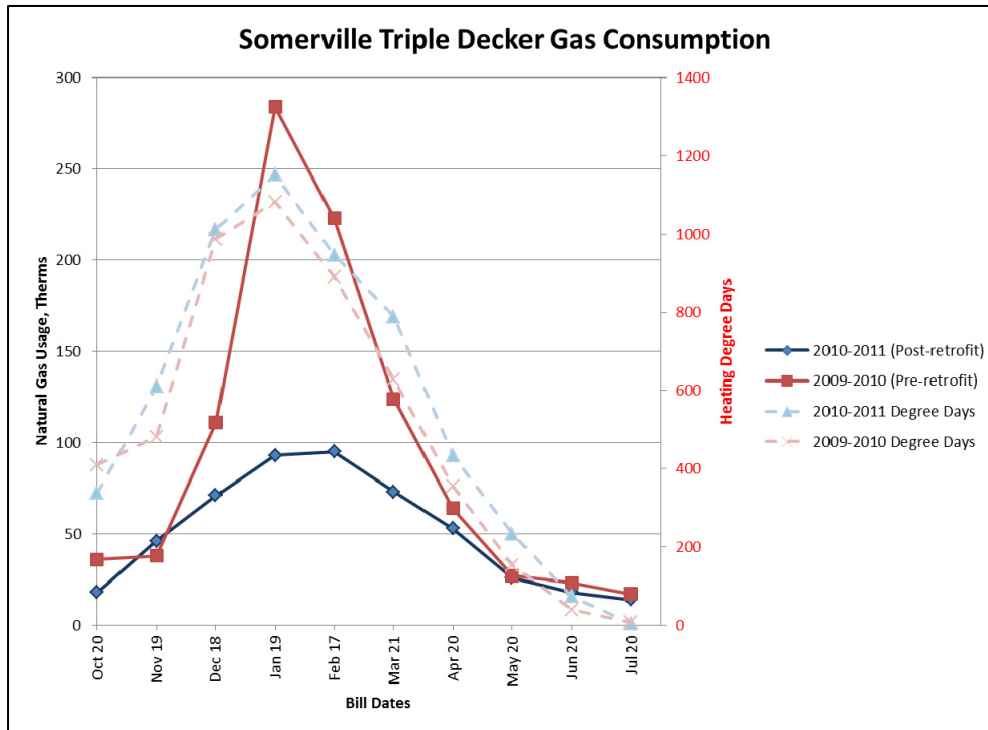
Figure 32. Somerville Triple Decker Gas consumption
