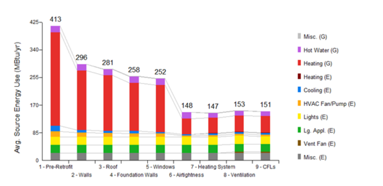
Figure 30. Parametric energy modeling of the Somerville Triple Decker
