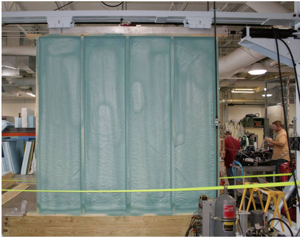
Figure 25. Structural testing wall 2 installed in apparatus
