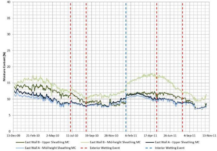
Figure 34. East Wall B (direct applied stucco) and east Wall A (insulating sheathing) middle and upper OSB sheathing measured MC
