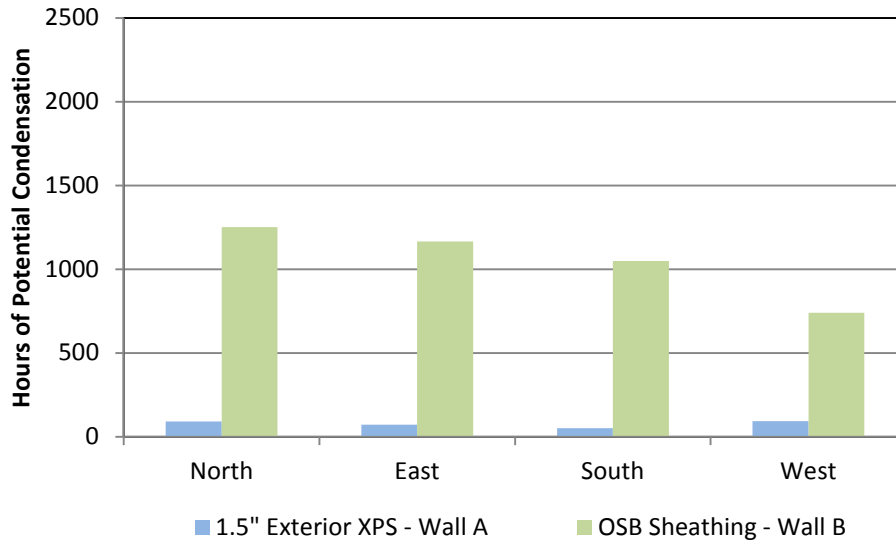
Figure 42. Comparison of the hours of potential condensation between Wall B and Wall A from December 18, 2009, to May 30, 2010, using measured interior dew point and sheathing temperature
