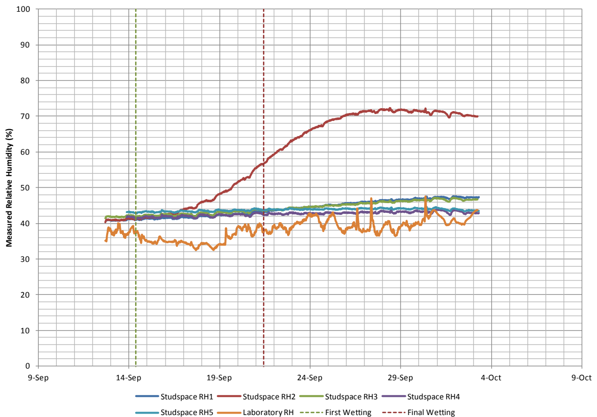
Figure 22. Measured RH in the five stud spaces
