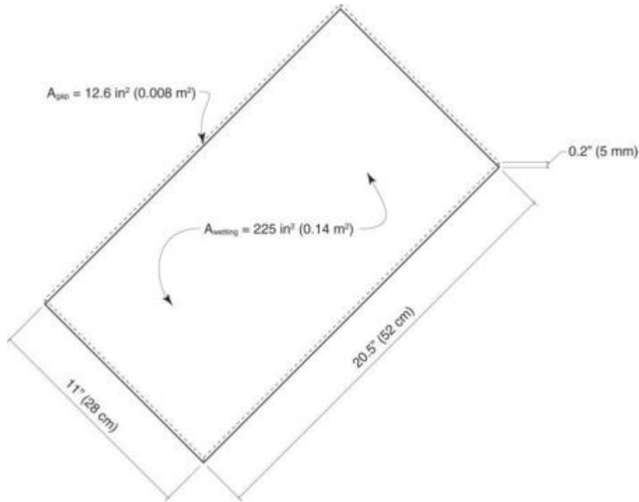
Figure 21. Comparison of surface areas for diffusion from wetting system
