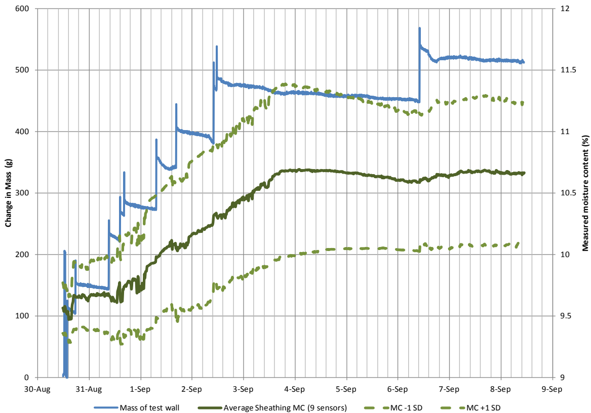
Figure 14. Repeated drainage gap wetting analysis, corrugated housewrap
