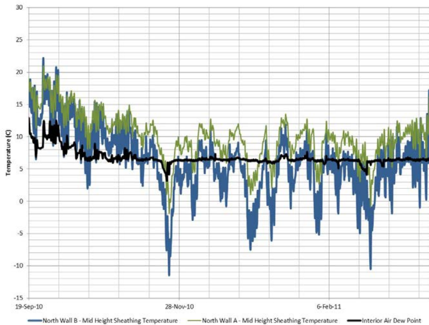
Figure 45. Comparison of condensation potential between north walls A and B, September to March 2010
