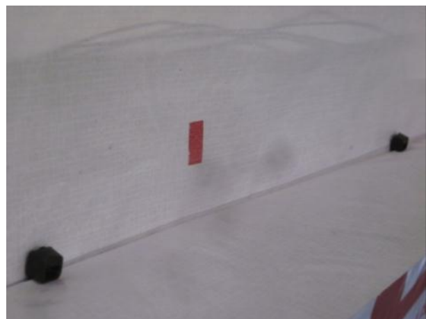
Figure 11. Spacers installed in top of drainage gap
