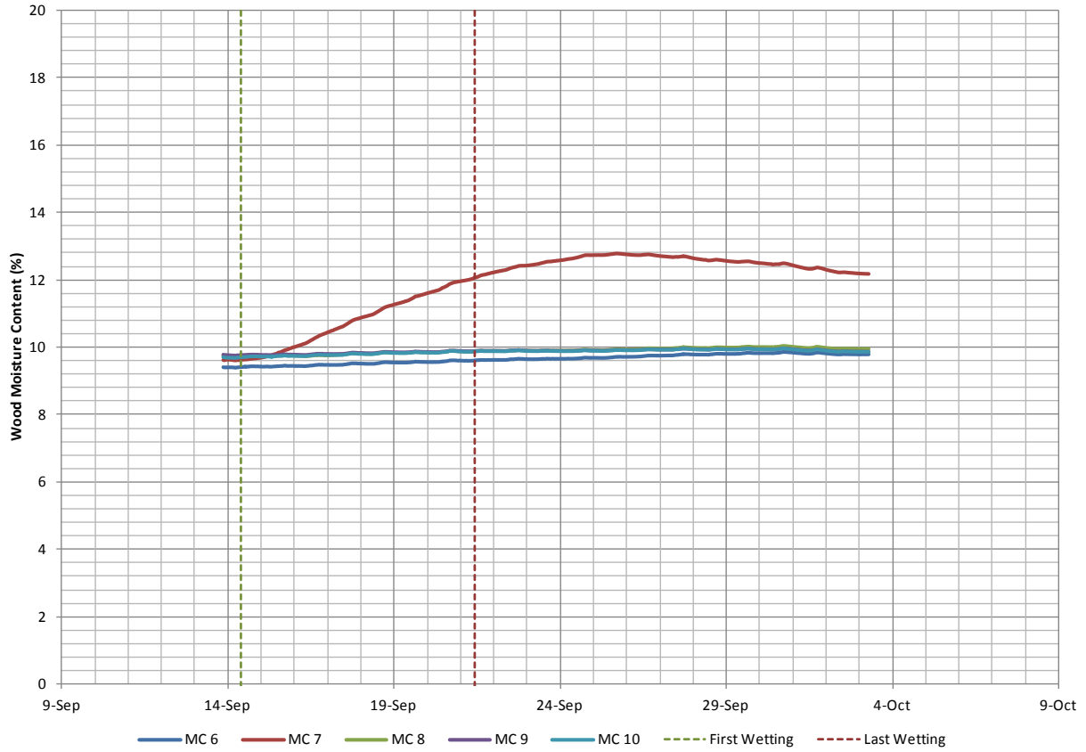
Figure 23. Measured MC sensors in all five stud spaces at the mid height of the wall
