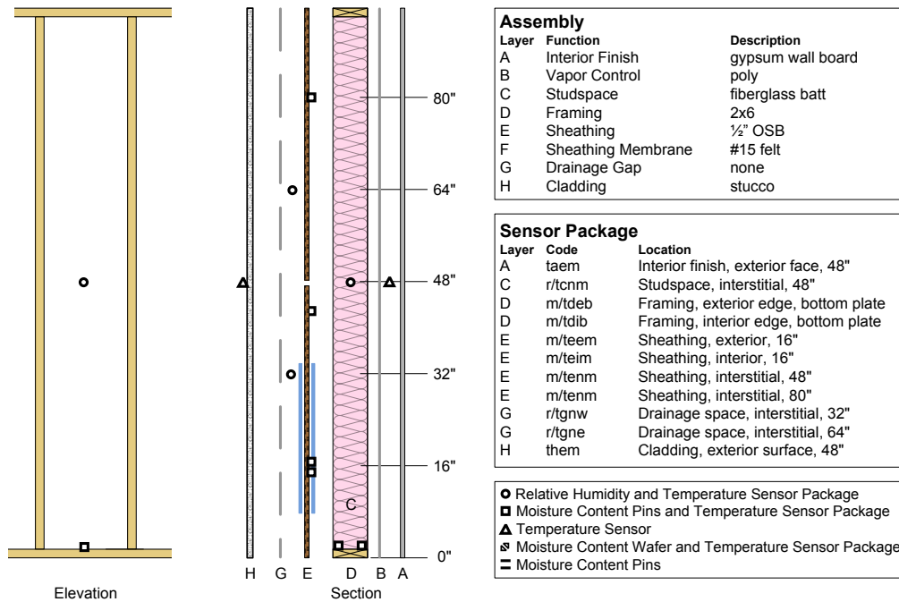
Figure 30. Typical wall construction and sensor configuration
