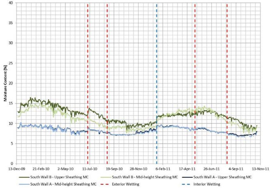
Figure 36. South Wall B (direct applied stucco) and south Wall A (exterior insulation) middle and upper OSB sheathing measured MC
