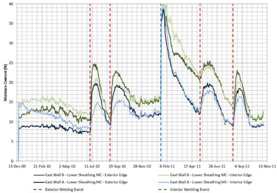
Figure 33. East Wall B (direct applied stucco) and east Wall A (insulating sheathing) lower OSB sheathing measured MC
