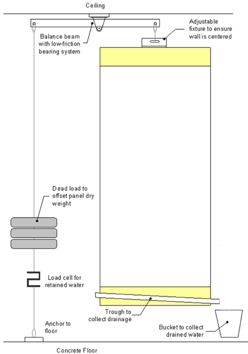
Figure 3. Wall balance schematic
