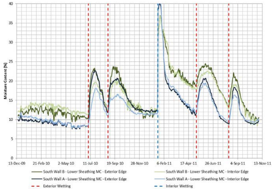
Figure 35. South Wall B (direct applied stucco) and south Wall A (exterior insulation) lower OSB sheathing measured MC
