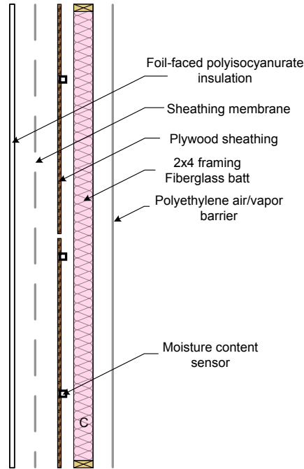
Figure 7. Typical test wall schematic
