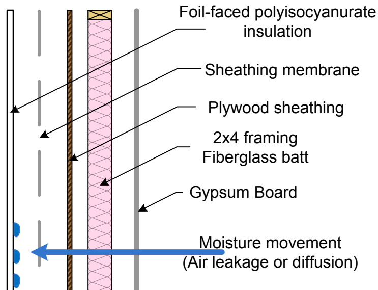
Figure 1. Moisture movement and condensation on interior surface of exterior insulation
