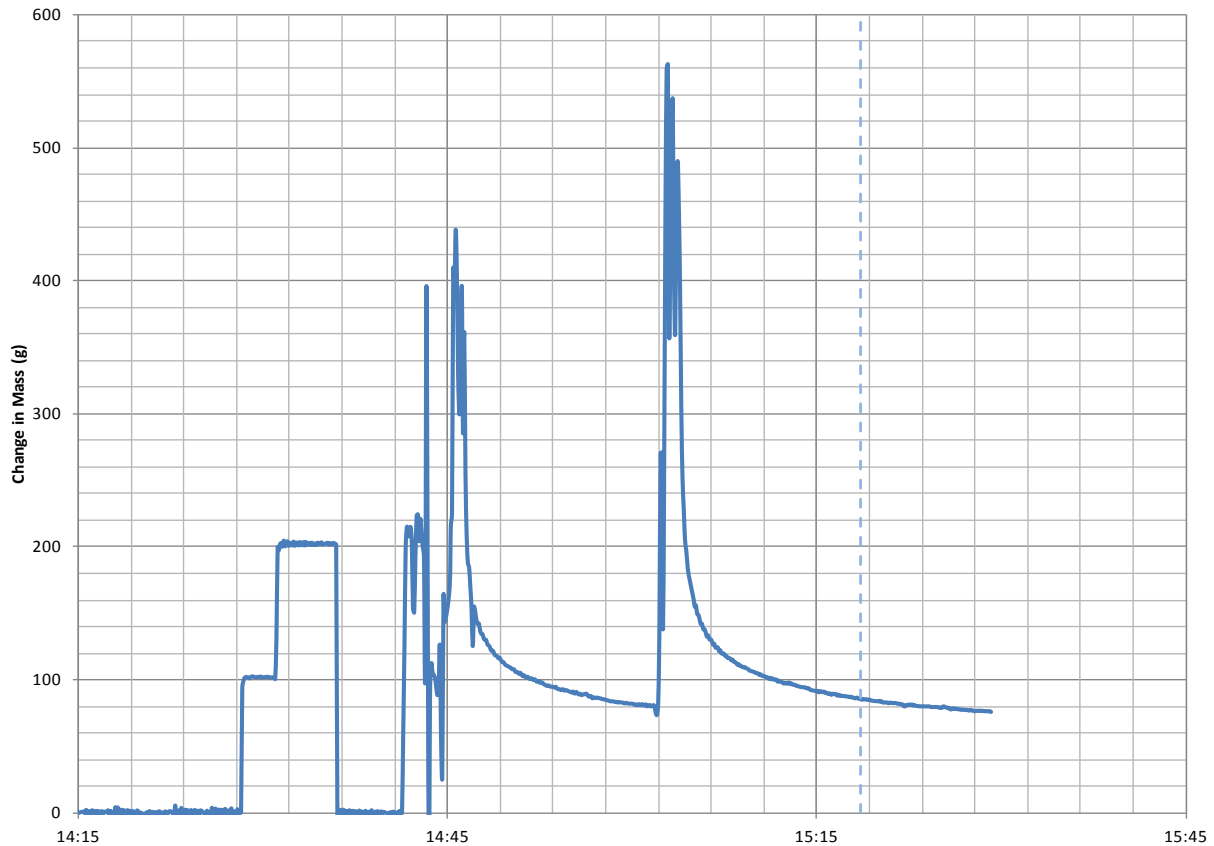
Figure 12. Smooth plastic housewrap drainage test
