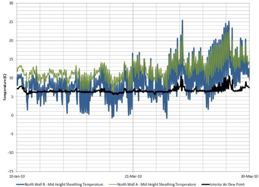
Figure 44. Comparison of condensation potential between north walls A and B, January to May 2010
