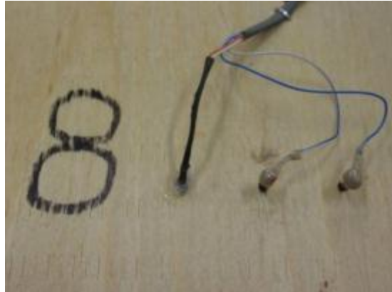
Figure 6. Installed wood MC sensor and thermistor
