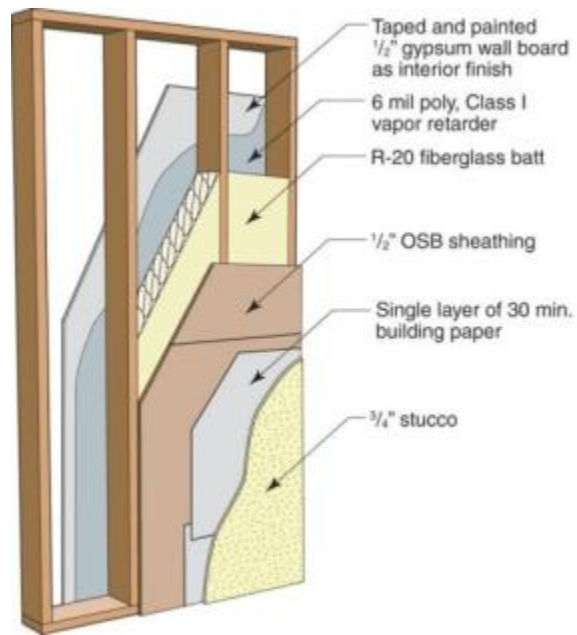
Figure 26. Direct applied stucco wall on all four orientations (Wall B)
