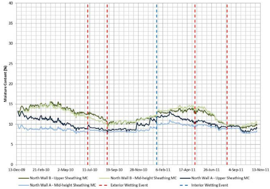
Figure 32. Middle and upper OSB sheathing measured MC comparison between north Wall B (direct applied stucco), and north Wall A (exterior insulation)
