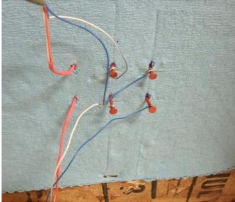
Figure 28. MC pins installed in plywood sheathing through the wetting system
