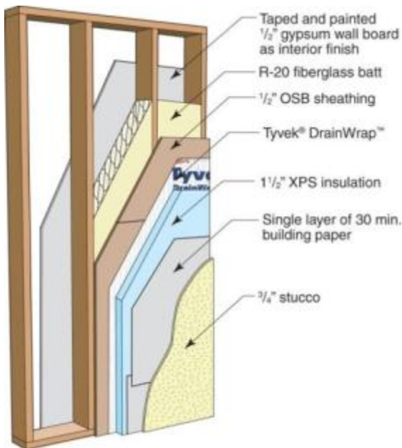
Figure 25. Exterior insulated wall on all four orientations (Wall A)
