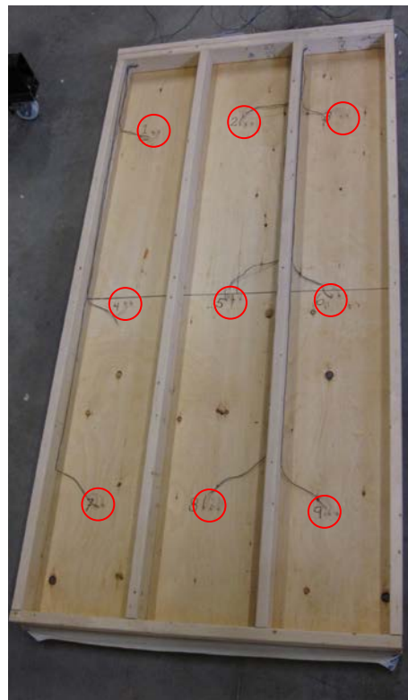
Figure 5. Location of wood MC sensors
