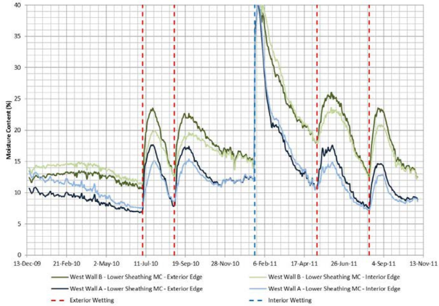
Figure 37. West Wall B and south Wall A lower OSB sheathing measured MC comparing exterior insulation
