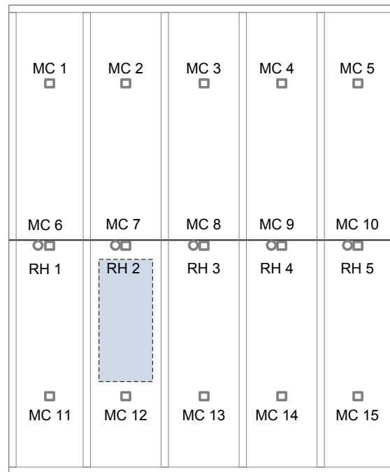
Figure 17. Layout for sheathing MC sensors and stud space RH sensors as shown from the “interior”
