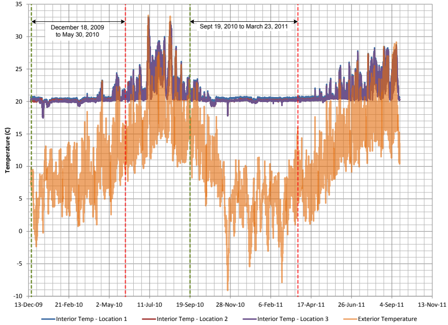
Figure 40. Measured interior and ambient temperatures
