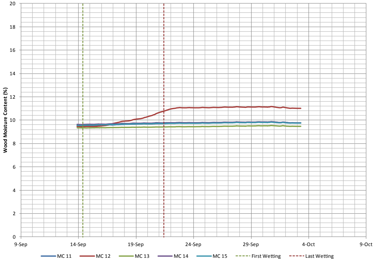
Figure 24. Measured MC sensors in all five stud spaces 16 in. from the bottom of the wall
