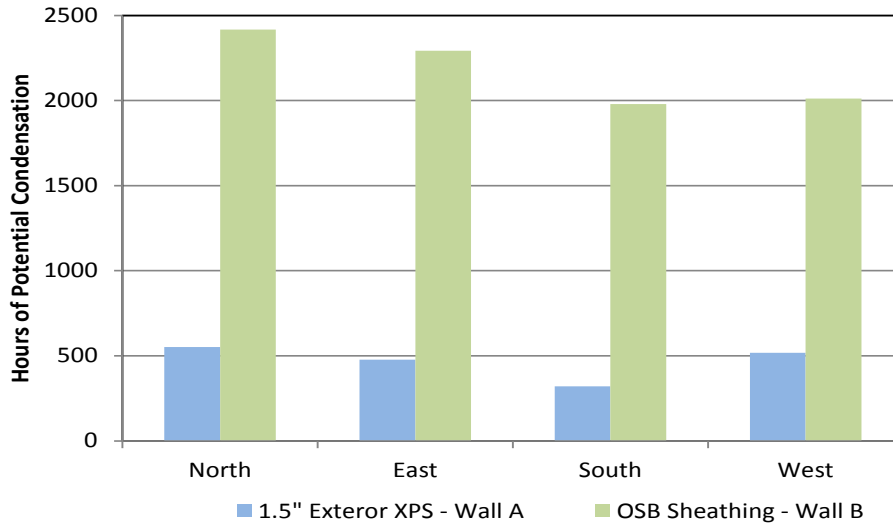
Figure 43. Comparison of the hours of potential condensation between Wall B and Wall A from September 19, 2010, to March 23, 2011, using measured interior dew point and sheathing temperature
