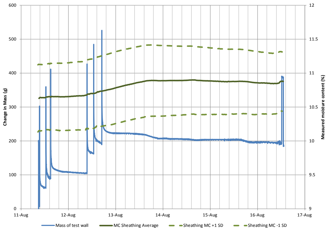
Figure 13. Repeated drainage gap wetting analysis, smooth housewrap
