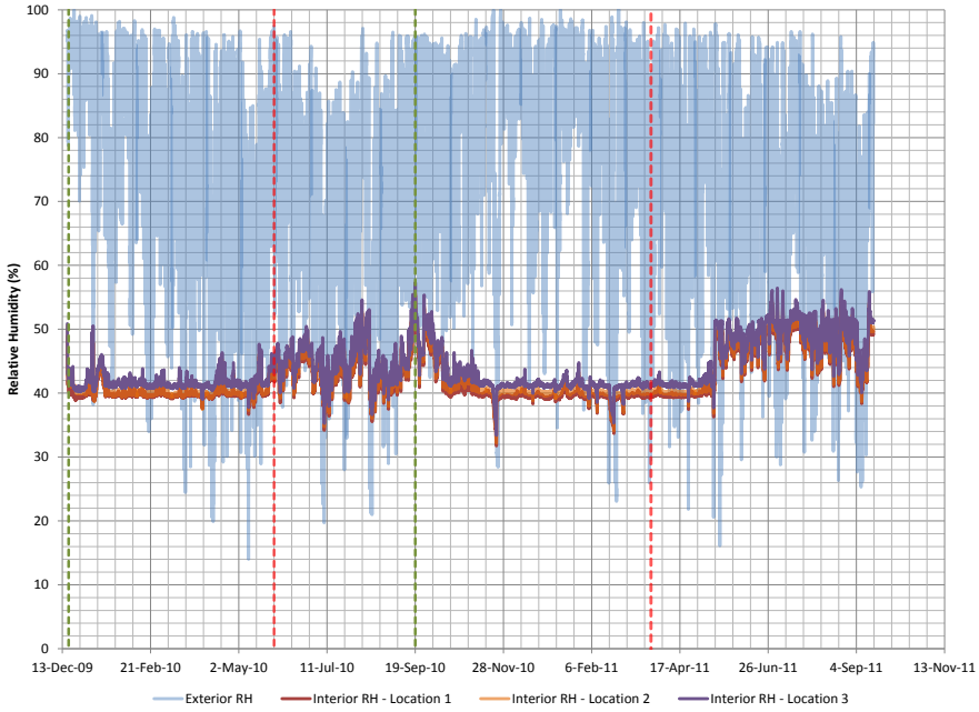
Figure 41. Measured interior and ambient RH
