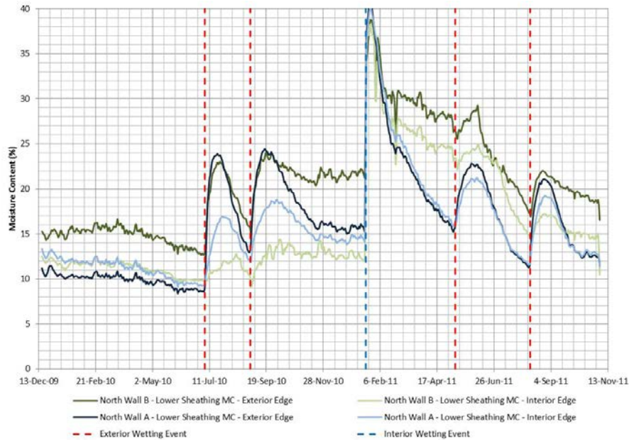
Figure 31. Lower OSB sheathing measured MC comparison between north Wall B (direct applied stucco) and north Wall A (exterior insulation)
