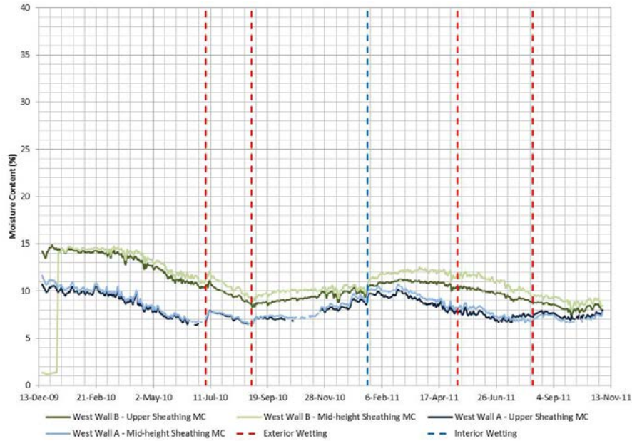
Figure 38. West Wall B and south Wall A middle and upper OSB sheathing measured MC comparing exterior insulation
