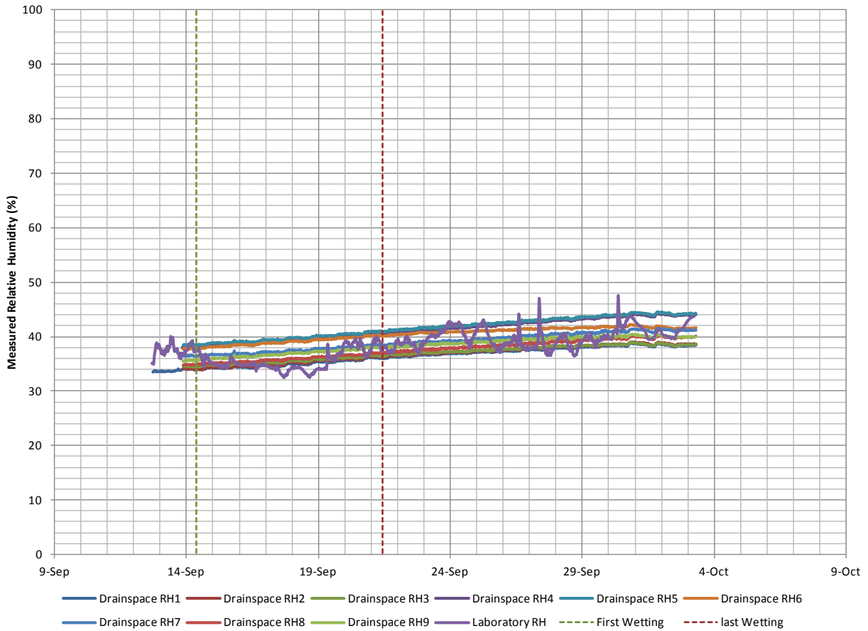
Figure 20. Measured RH at nine locations in the drainage space
