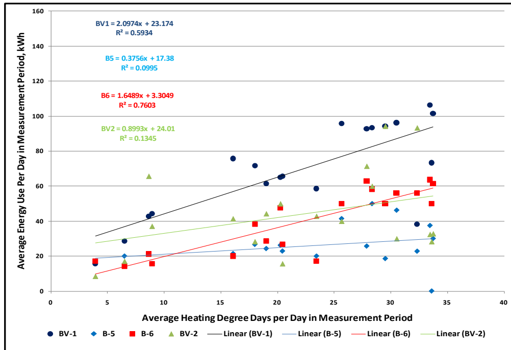
Figure 24. BV-1, B-5, B-6 and BV-2 average daily usage and HDD for the heating period.
