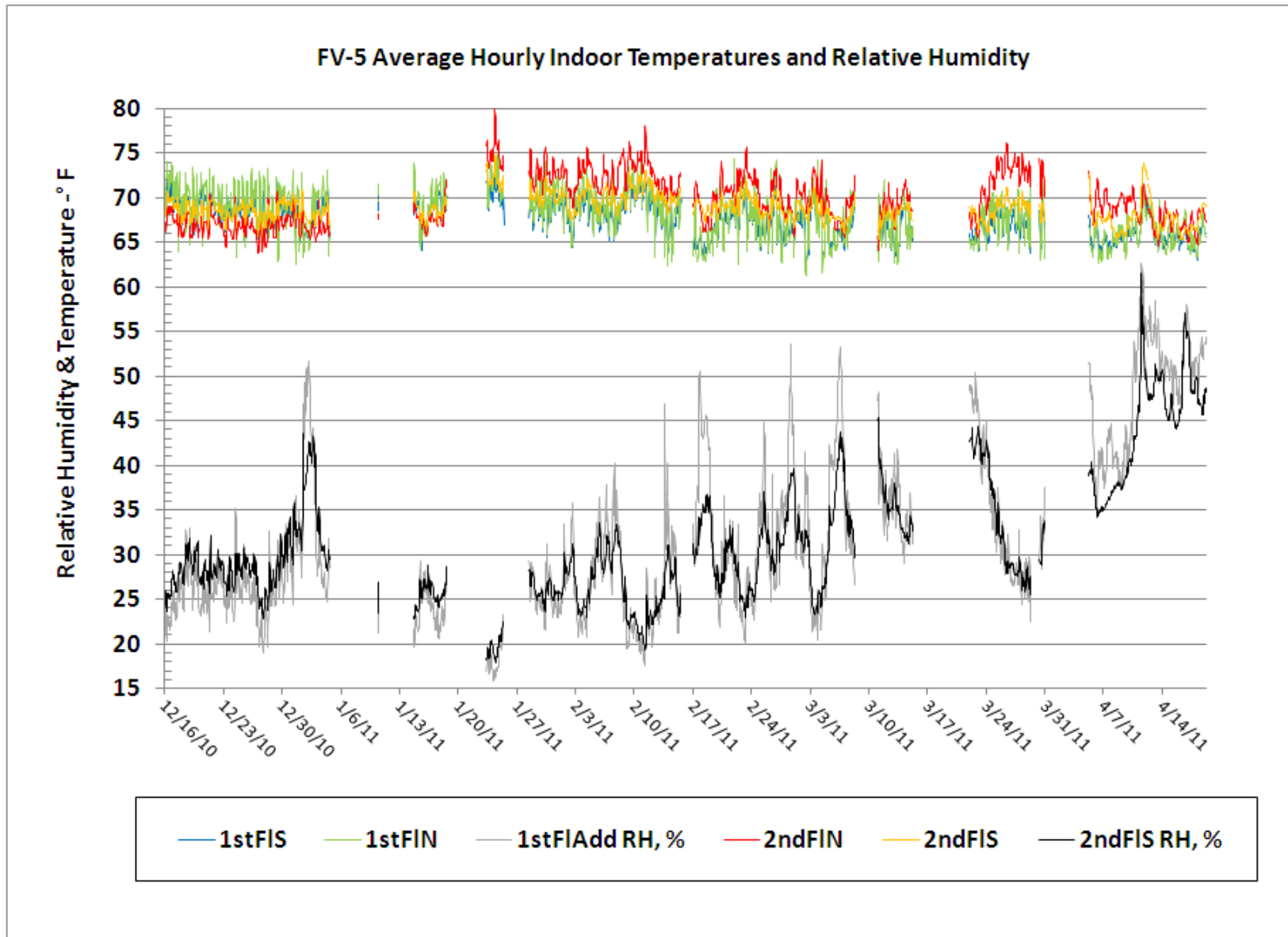
Figure 83. FV-5 Average Hourly Temperature – December 2010 to April 2011.
