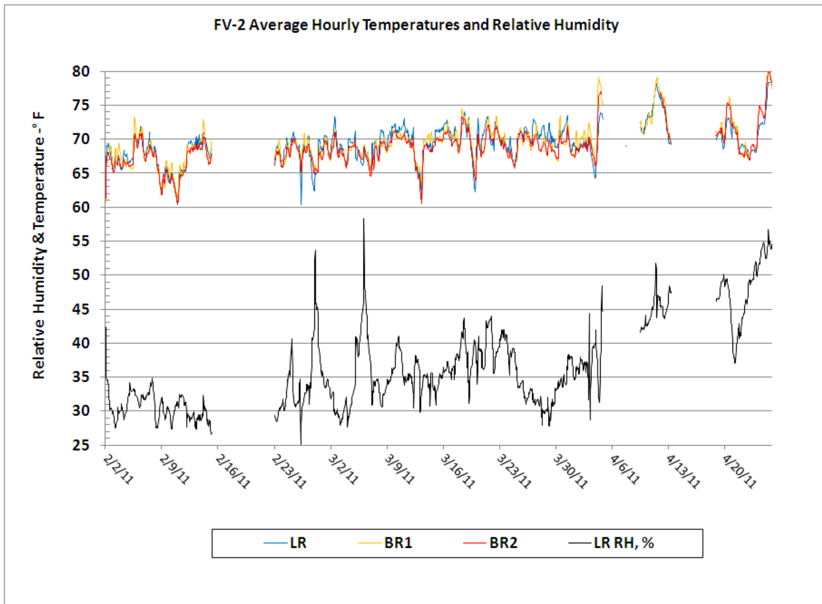
Figure 80. FV-2 Average Hourly Temperature – February 2011 to April 2011.
