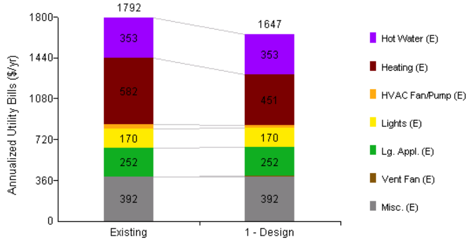
Figure 53. Modeled energy use FB-2.
