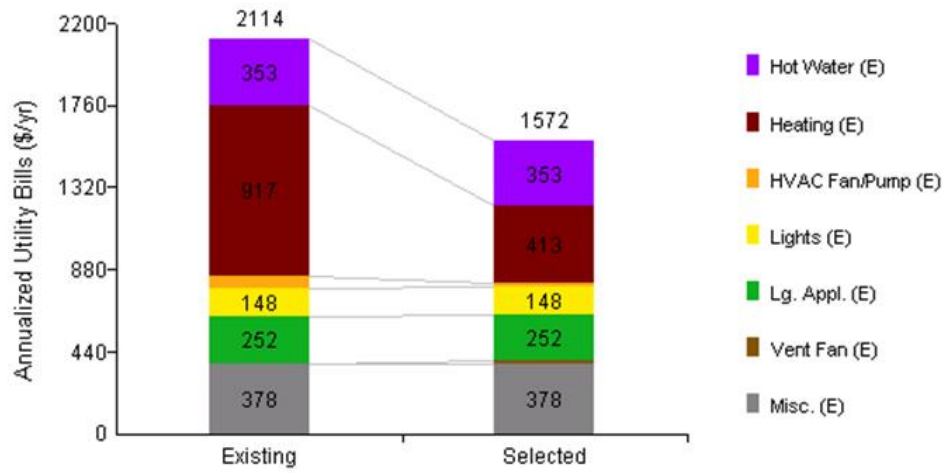
Figure 47. Modeled energy use B-2.
