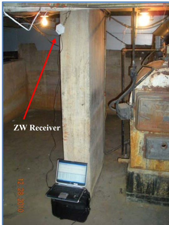
Figure 7. Onset receiver (data download in progress).
