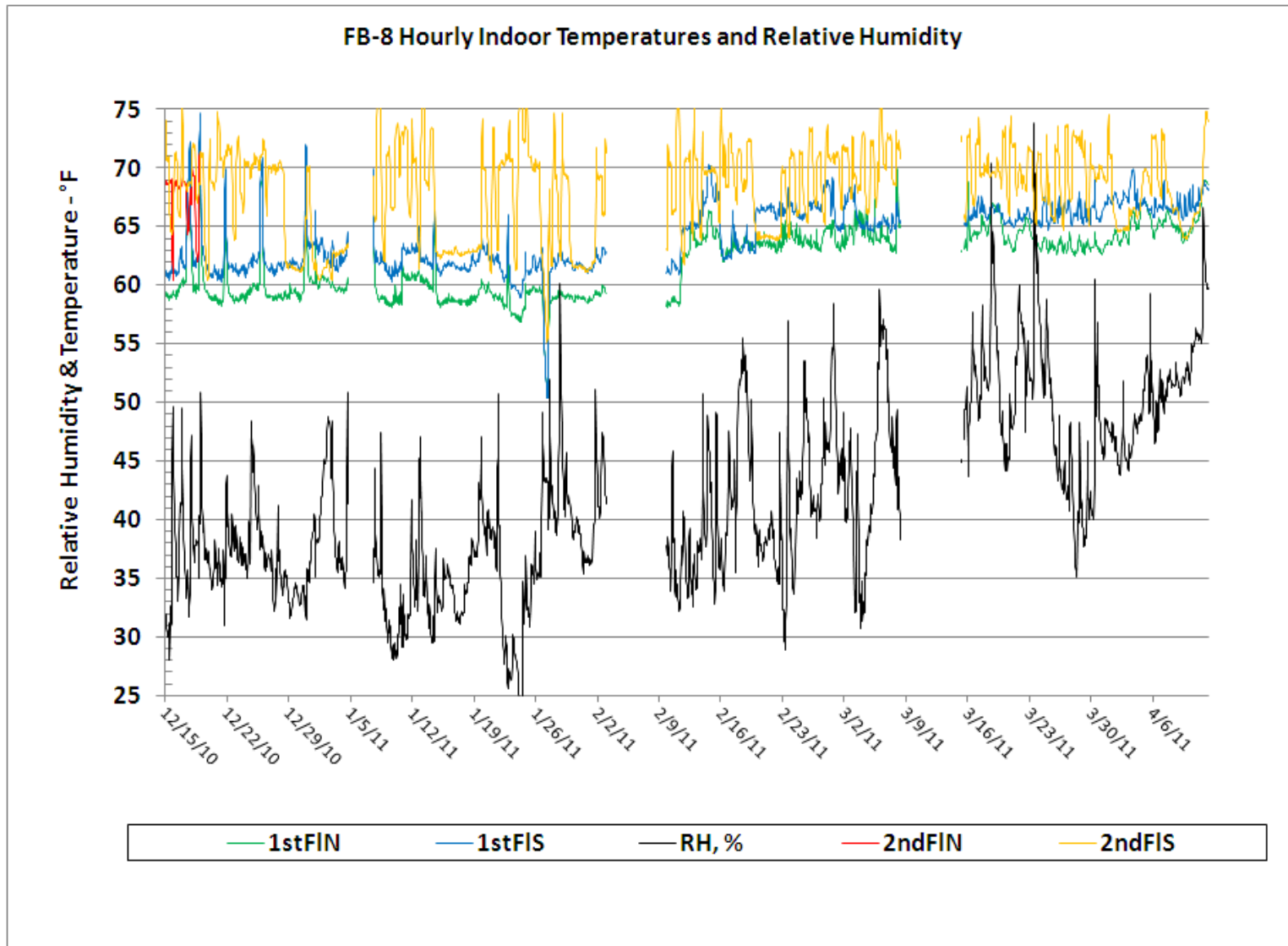
Figure 78. FB-8 Average Hourly Temperature – December 2010 to April 2011.
