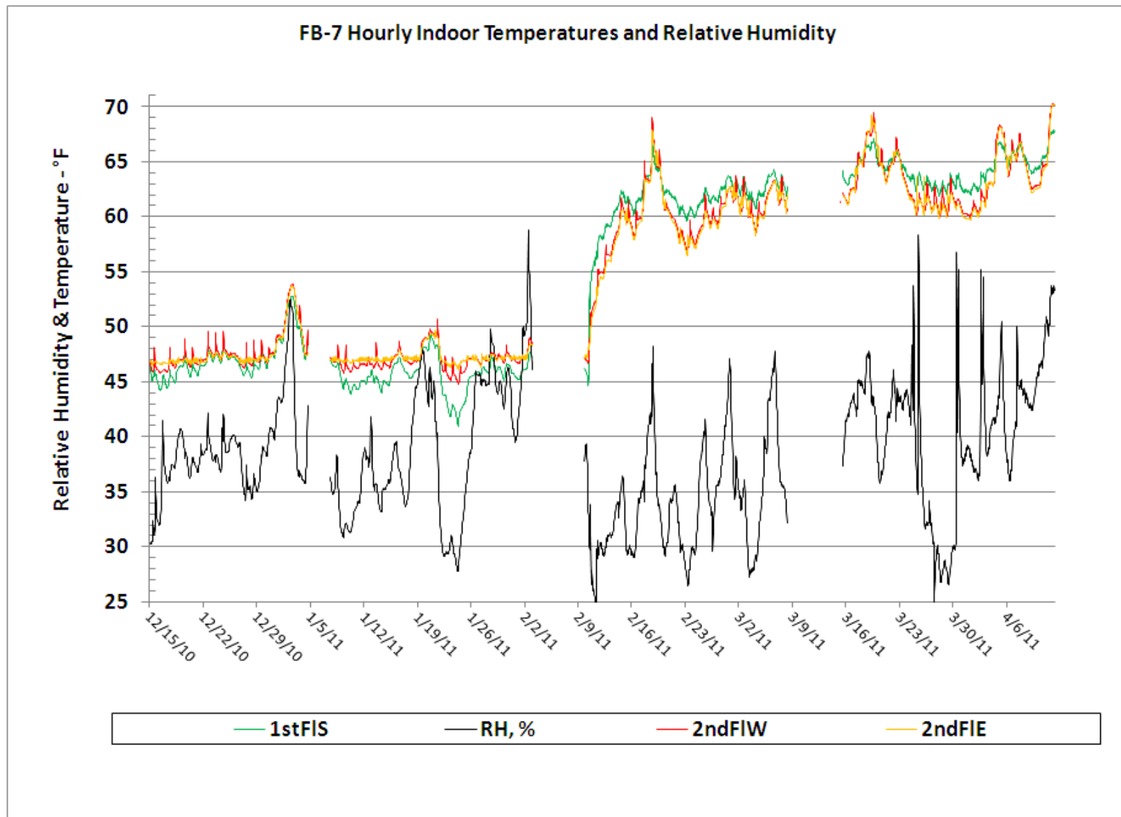
Figure 77. FB-7 Average Hourly Temperature – December 2010 to April 2011.
