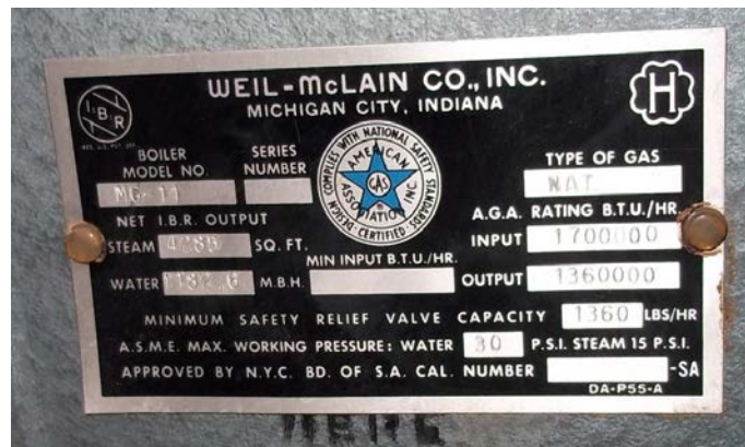
Figure 10. Sample boiler plate for a natural gas boiler that contains information about boiler specifications
