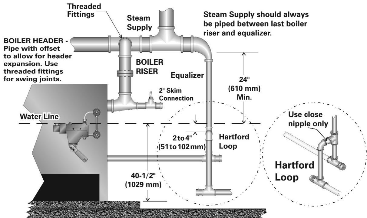
Figure 7. Specifications for how to pipe a Series 211A™ natural gas steam boiler by Peerless® Boilers
