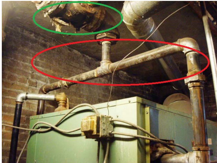
Figure 6. The header piping is smaller than the boiler manufacturer's specifications.
