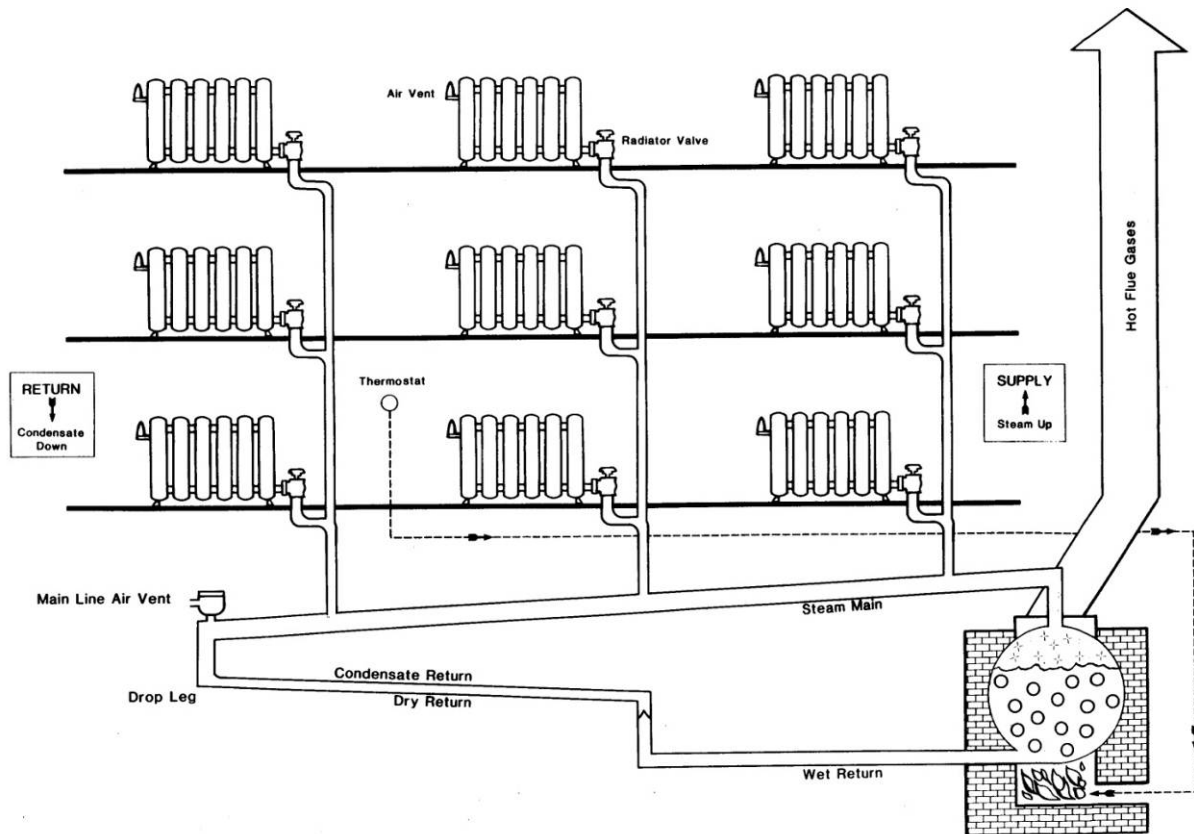
Figure 3. Schematic of one-pipe gravity return steam system (adapted and used with permission from Peterson 1985)
