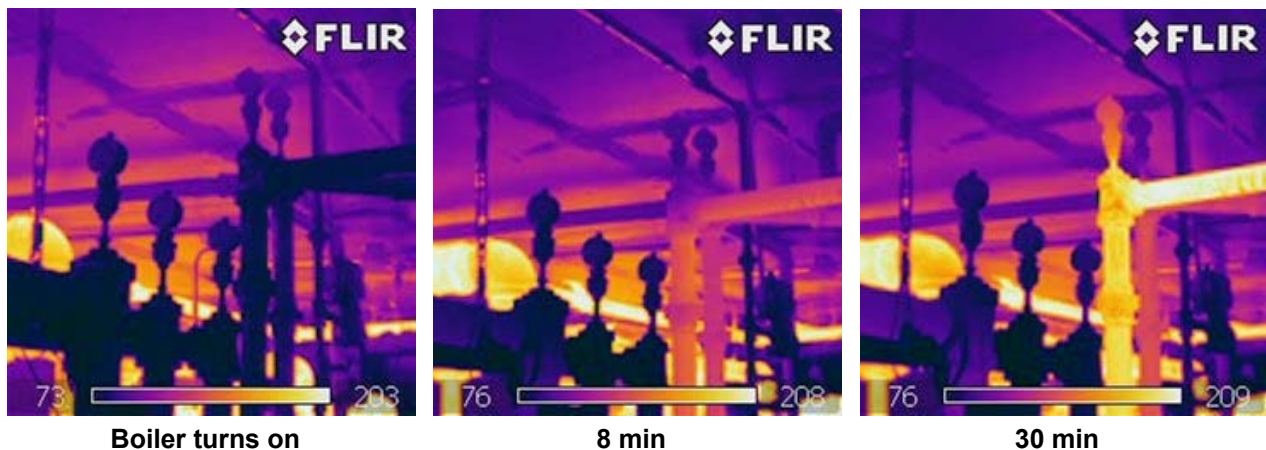
Figure 4. At the beginning of a boiler firing cycle, the main lines are filled with air and quite cool, meaning that the steam must heat a large mass of piping and push air out of the air vents. As time passes, the main lines fill with steam and become hot. In an unbalanced system, some of the steam lines may never heat up during the boiler cycle.
