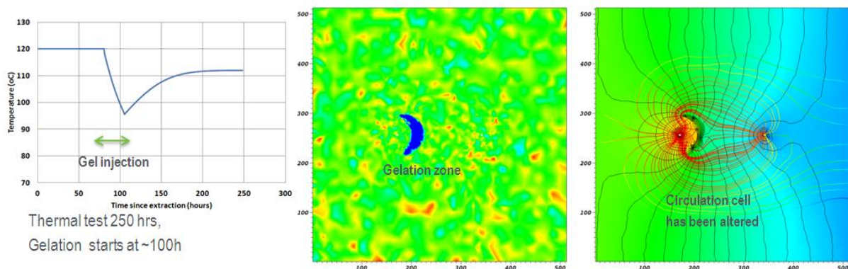
FIGURE 21. TWO DIMENSIONAL DOUBLET FLOW AND TRANSPORT SIMULATIONS OF GEL IN A SINGLE ROUGH FRACTURE. LEFT: THERMAL TEST PROTOCOL AND TEMPERATURE RESPONSES AS FUNCTION OF TIME. CENTER: APERTURE RANDOM FIELD WITH CRESCENT-LIKE DIVERTER E.G. GELLED SILICA. RIGHT: FLOW NETWORK SHOWING THE IMPACT OF GELLED SILICA ON STREAMLINES AND FLOW CELLS.
