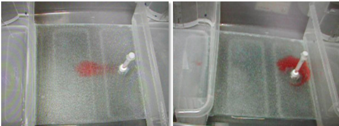
FIGURE 14. TRANSPARENT FLOW CELL EXPERIMENTAL SETUP SHOWING GEL EMPLACEMENT
