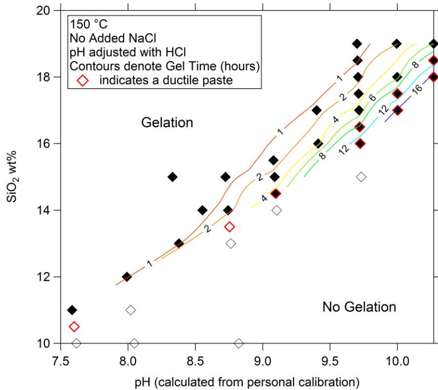
FIGURE 13. CONTOUR PLOT OF MODELED GEL TIMES AT 150 °C AS A FUNCTION OF SILICA CONCENTRATION AND PH
