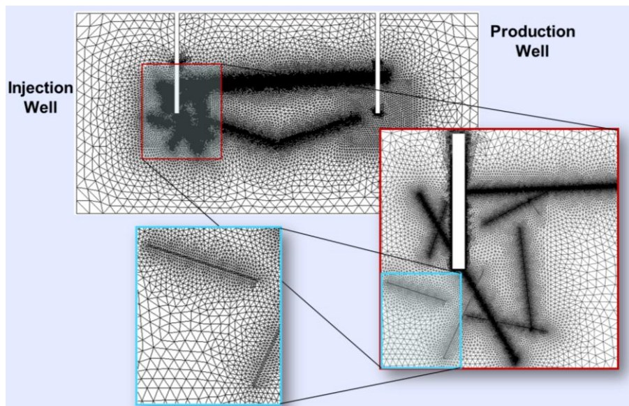
FIGURE 30. SCHEMATIC OF A VERTICAL CROSS-SECTION THROUGH A 3D GEOTHERMAL RESERVOIR. FIGURE SHOWS THE OPERATIONAL WELLS. ADAPTIVE MESH REFINEMENT WAS USED TO REPRESENT THE FRACTURES WITH HIGH FIDELITY AND ILLUSTRATED THROUGH SEVERAL ZOOM-OUTS.
