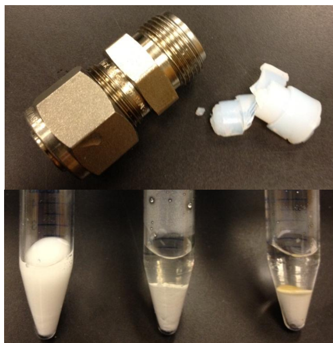
FIGURE 8. GEL (RIGHT) PRODUCED IN A 300 °C OVEN. WATER WAS PREVENTED FROM ESCAPING BY SEALING THE COLLOIDAL SOLUTION IN A SWAGELOK CAPSULE (LEFT). THE SHAPE OF THE GEL REFLECTS THE INTERNAL GEOMETRY OF THE CAPSULE.
