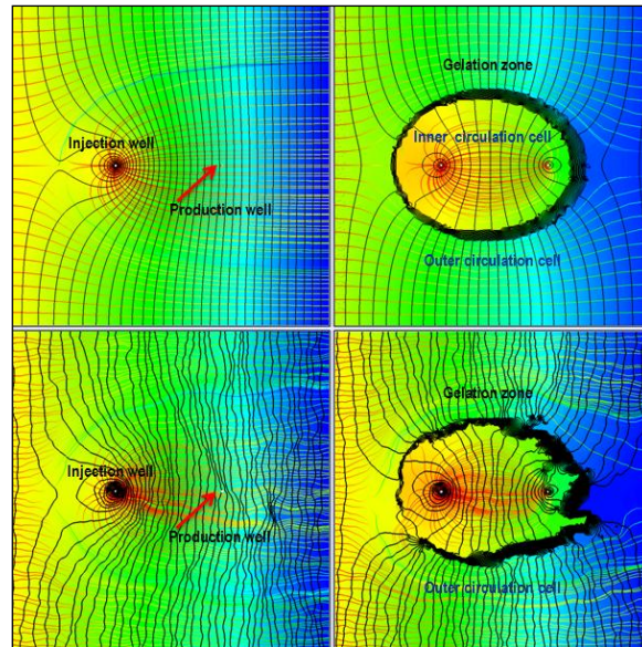
FIGURE 26. INITIAL (LEFT) AND FINAL (RIGHT) SNAPSHOTS OF TWO DIMENSIONAL DOUBLET FLOW AND TRANSPORT SIMULATIONS OF GEL IN A SINGLE SMOOTH (TOP) ROUGH FRACTURE (BOTTOM). EACH FRAME DEPICTS THE GEL LOCATION AND THE FLOWNET. IN THE LEFT FRAMES THE PRODUCTION WELL IS OFF, WHILE IN THE RIGHT FRAMES THE PRODUCTION WELL IS ON.
