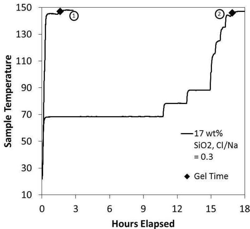
FIGURE 7. GEL TIME AS A FUNCTION OF HEATING PATH.
