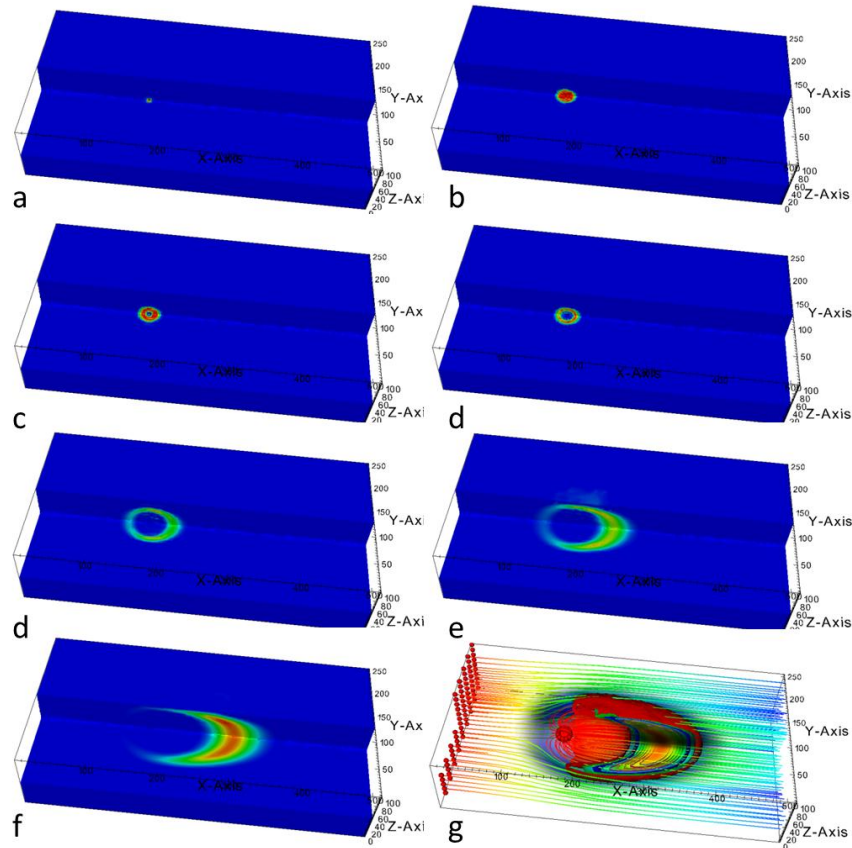
FIGURE 28. ILLUSTRATION OF 3D SEDIMENTARY GEOTHERMAL RESERVOIR. SNAPSHOTS A-F DEPICT THE TIME EVOLUTION OF THE INJECTED SILICA WHILE FRAME (G) DEPICTS THE COMPLEX STREAMLINES AROUND THE SILICA GEL.
