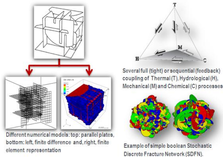
FIGURE 18. SDFN-THMC (EZZEDINE, 2005) OFFERS AN IDEAL NUMERICAL FRAMEWORK TO ADDRESS THE PROBLEM OF DEPLOYING SILICA GEL IN EGS. THE MODEL ALLOWS FOR FLOW, THERMAL, AND MECHANICAL & CHEMICAL SIMULATION IN A 3D STOCHASTIC DISCRETE FRACTURE NETWORK.
