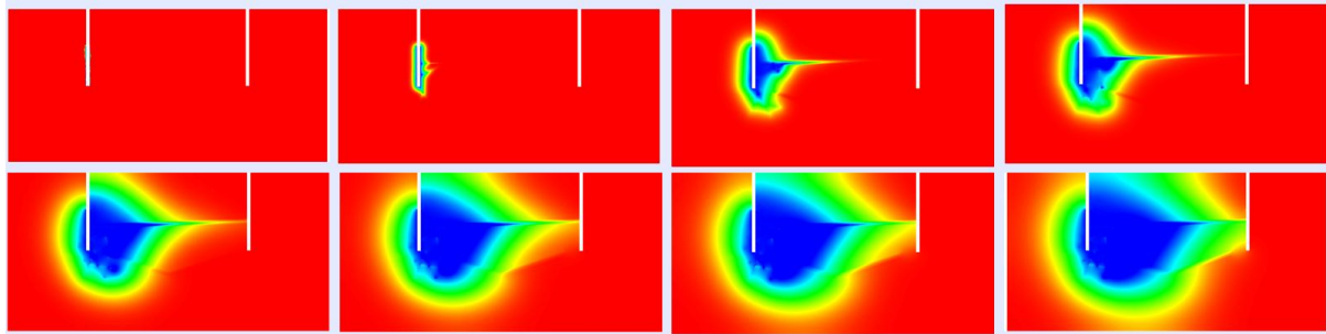
FIGURE 33. SCHEMATIC OF A VERTICAL CROSS-SECTION THROUGH A 3D GEOTHERMAL RESERVOIR AFTER GEL DEPLOYMENT. A TRACER (THERMAL) TEST WAS INJECTED. FIGURE DEPICTS TIME-SNAPSHOTS OF THE TRACER/HEAT TRANSFER THROUGH THE RESERVOIR. TIME FLOWS FROM LEFT TO RIGHT AND TOP TO BOTTOM. BLUE COLOR DEPICTS COLD REGIONS WHILE RED COLOR REPRESENTS HOT REGIONS. ONE CAN SEE THAT THE BOTTOM FRACTURE IS OBSTRUCTED AFTER SILICA GEL HAS BEEN DEPLOYED AND THAT THE COLD REGION INITIALLY OBSERVED BEFORE GEL DEPLOYMENT HAS VANISHED.
