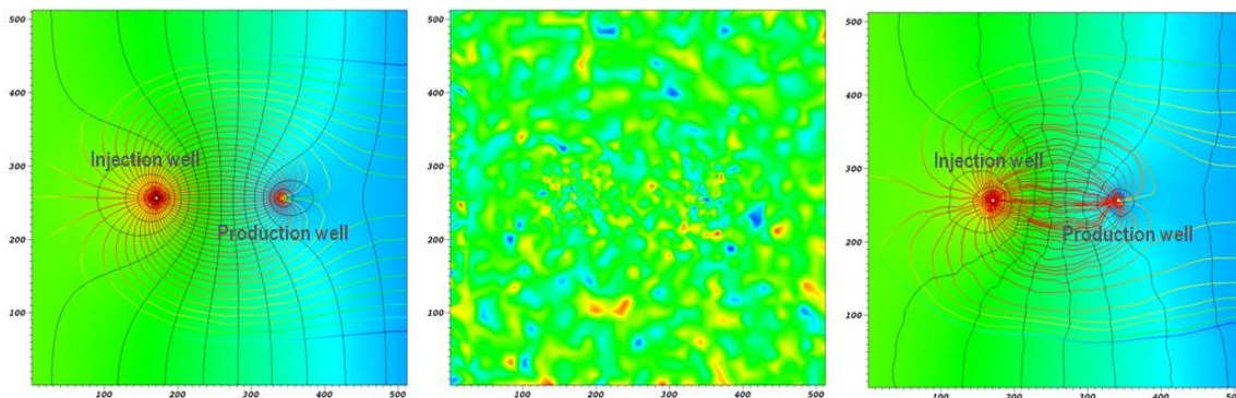
FIGURE 20. TWO DIMENSIONAL DOUBLET FLOW SIMULATIONS IN A SINGLE FRACTURE. LEFT: FLOW NETWORK (PRESSURE AND STREAMLINES) IN A SMOOTH FRACTURE. CENTER: APERTURE RANDOM FIELD, RED DEPICTS LARGE APERTURE WHILE BLUE DEPICTS SMALL APERTURE. RIGHT: FLOW NETWORK IN A ROUGH FRACTURE.
