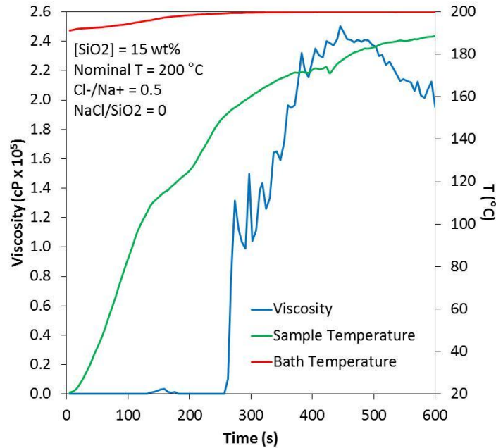
FIGURE 6. VISCOSITY, OIL BATH TEMPERATURE AND SAMPLE TEMPERATURE AS A FUNCTION OF TIME, AT A NOMINAL EXPERIMENTAL TEMPERATURE OF 200 °C.
