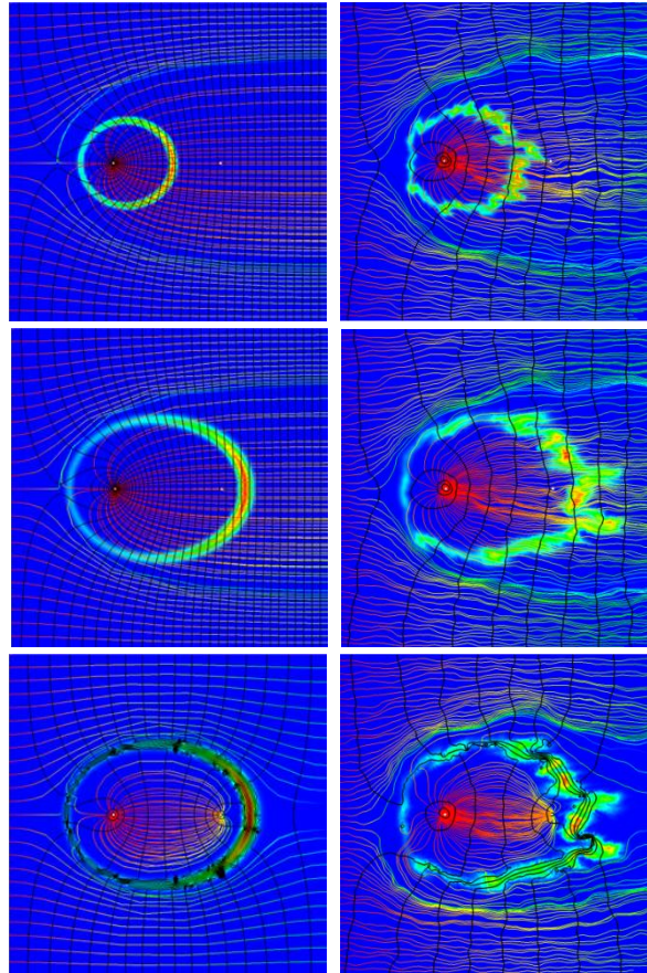
FIGURE 25. SNAPSHOTS OF TWO DIMENSIONAL DOUBLET FLOW AND TRANSPORT SIMULATIONS OF GEL IN A SINGLE SMOOTH (LEFT) ROUGH FRACTURE (RIGHT). TIME FLOWS FROM TOP TO BOTTOM. EACH FRAME DEPICTS THE GEL LOCATION AND THE FLOWNET. IN THE 4 TOP FRAMES THE PRODUCTION WELL IS OFF, WHILE IN THE LAST ROW THE PRODUCTION WELL IS ON.
