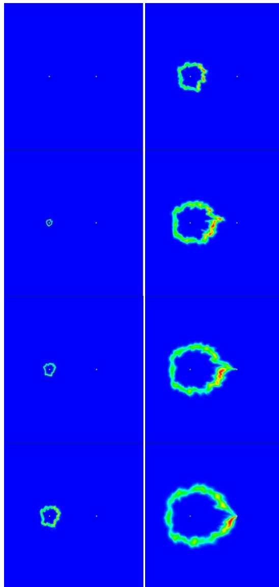
FIGURE 23. SNAPSHOTS OF TWO DIMENSIONAL DOUBLET FLOW AND TRANSPORT SIMULATIONS OF GEL IN A SINGLE ROUGH FRACTURE. TIME FLOWS FROM TOP TO BOTTOM AND LEFT TO RIGHT. TOP LEFT PICTURE DEPICTS THE HYDROLOGICAL CONDITIONS. PAINTED COLORS ARE NOT AT THE SAME SCALE; THESE PICTURES ARE FOR ILLUSTRATION PURPOSES.
