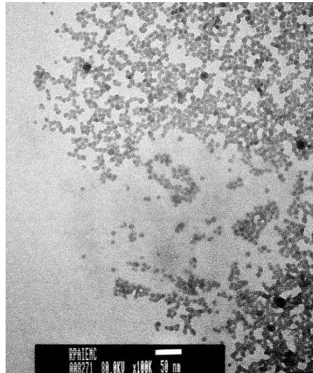
FIGURE 1. SILICA GEL PRODUCED FROM THE MAMMOTH LAKES GEOTHERMAL FLUID. THE GEL IS MADE UP OF A NETWORK OF 10 NM SILICA COLLOIDS (BOURCIER, 2009).
