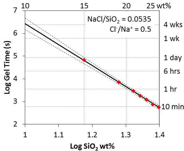
FIGURE 2. LOG GEL TIME VERSUS SILICA CONCENTRATION. DASHED LINES REPRESENT 95% CONFIDENCE INTERVALS
