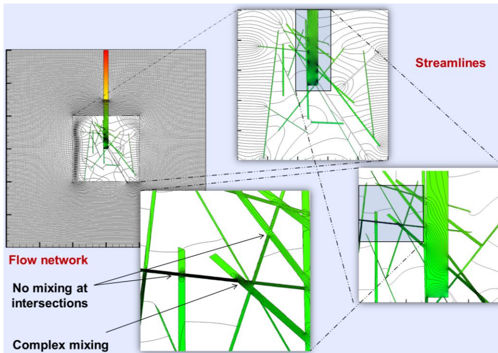
FIGURE 31. SCHEMATIC OF A VERTICAL CROSS-SECTION THROUGH A 3D GEOTHERMAL RESERVOIR NEAR THE INJECTION WELL. FIGURE DEPICTS STREAMLINES WITH THE DOMAIN. ADAPTIVE MESH REFINEMENT WAS USED TO REPRESENT THE FRACTURES AND THE STREAMLINES WITH HIGH FIDELITY AND ILLUSTRATED THROUGH SEVERAL ZOOM-OUTS. STREAMLINES ARE ESSENTIAL FOR TRACKING THE SILICA GEL DEPLOYMENT AND TO ASSESS THE IMPACT OF MIXING WITHIN FRACTURES ON THE GELATION TIME.
