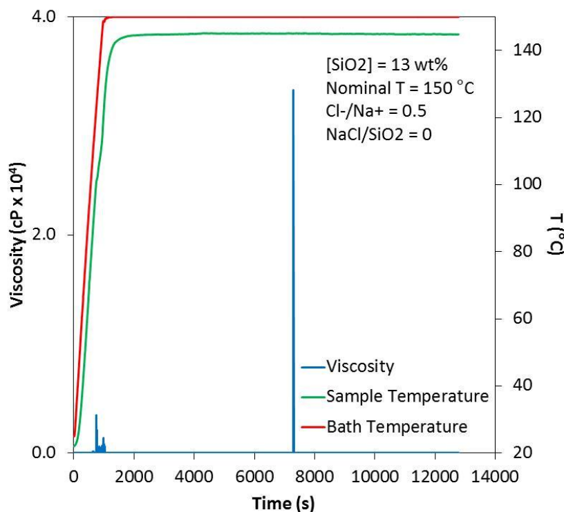
FIGURE 10. VISCOSITY, OIL BATH TEMPERATURE AND SAMPLE TEMPERATURE MEASUREMENTS AS A FUNCTION OF TIME.
