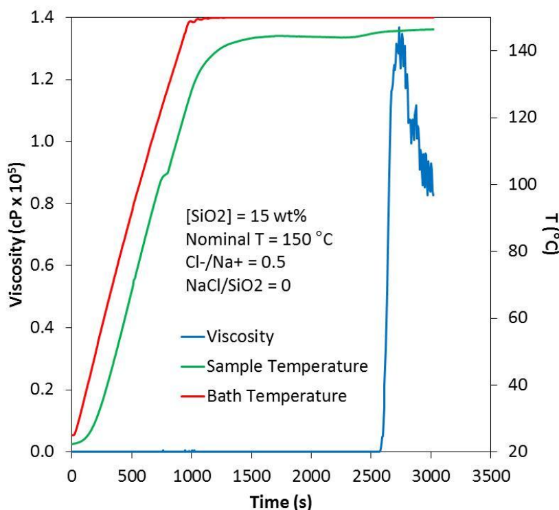
FIGURE 5. VISCOSITY, OIL BATH TEMPERATURE AND SAMPLE TEMPERATURE MEASUREMENTS AS A FUNCTION OF TIME.
