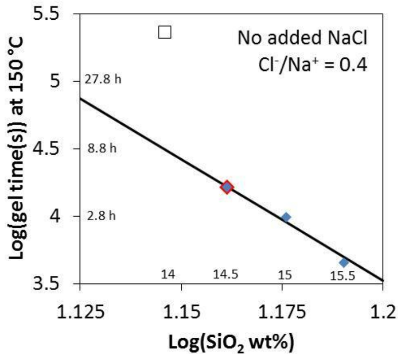
FIGURE 11. GELATION TIME AS A FUNCTION OF SILICA CONCENTRATION AT 150 °C
