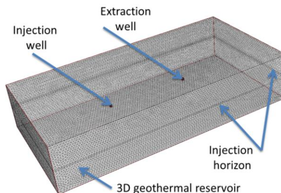
FIGURE 27. ILLUSTRATION OF 3D SEDIMENTARY GEOTHERMAL RESERVOIR. THIS FIGURE SHOWS BOTH INJECTION AND PRODUCTION WELLS INTERSECTING THE INJECTION/EXTRACTION HORIZON.
