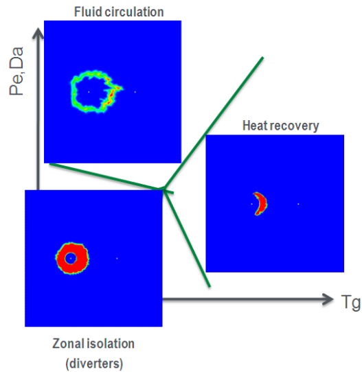
FIGURE 24. ILLUSTRATION OF DIFFERENT OUTCOMES OF GEL DEPLOYMENT AS A FUNCTION OF THE KEY PHYSICO-CHEMICAL PARAMETERS THAT GOVERN FLOW, HEAT, GEL TRANSPORT AND GELATION TIME.
