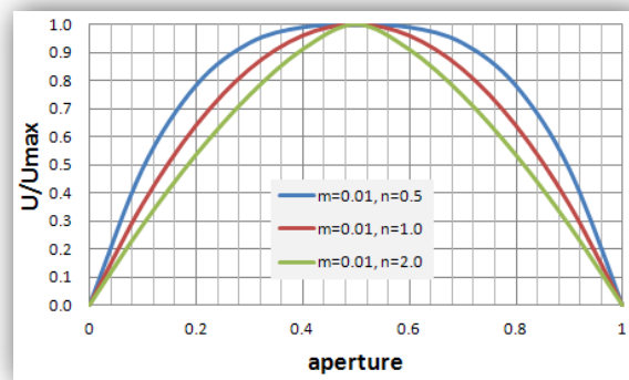
FIGURE 19. NORMALIZED VELOCITY PROFILE OF FLUID WITHIN FRACTURE APERTURE. PARAMETERS M AND N ARE CHARACTERISTICS OF THE FLUID AND THE PROFILE. RED PROFILE, PARABOLIC, IS THE NEWTONIAN, THE OTHER TWO (BLUE AND GREEN) ARE NON-NEWTONIAN.
