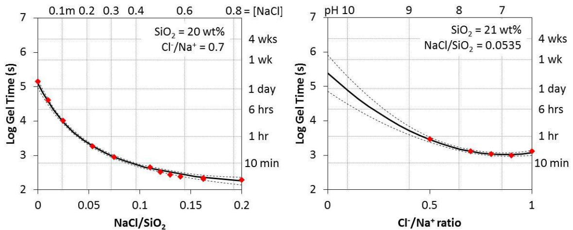
FIGURE 3. LOG GEL TIME VERSUS SALT/SILICA RATIO AND LOG GEL TIME VERSUS \text{Cl}^-/\text{Na}^+ (UN) RATIO. DASHED LINES REPRESENT 95% CONFIDENCE INTERVALS
