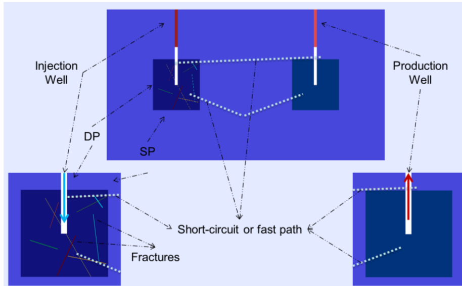
FIGURE 29. SCHEMATIC OF A VERTICAL CROSS-SECTION THROUGH A 3D GEOTHERMAL RESERVOIR. FIGURE SHOWS THE OPERATIONAL WELLS WHICH ARE EMBEDDED IN A DOUBLE POROSITY MEDIUM (DP), THE BACKGROUND RESERVOIR IS CONSIDERED AS A SINGLE POROUS MEDIUM (SP). SEVERAL FRACTURES ARE ALSO EMBEDDED WITH THE RESERVOIR; TWO OF THEM INTERSECT BOTH WELLS. THE BOTTOM FRACTURE, UNSEEN BY BOTH WELLS, PLAYS THE ROLE OF HIGH CONDUCTIVE FRACTURE AND THUS SHORT-CIRCUITING BOTH “WELLS”.
