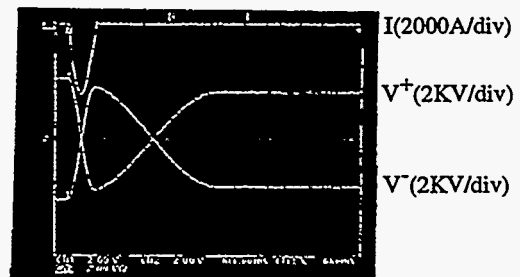
Fig 7 Output current and energy recovery waveforms
