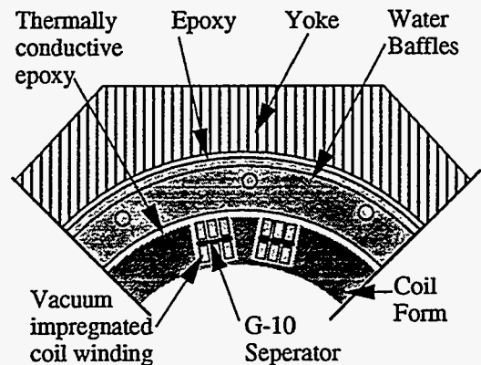
Fig. 1 Cross-sectional view of one quadrant of the Magnet
