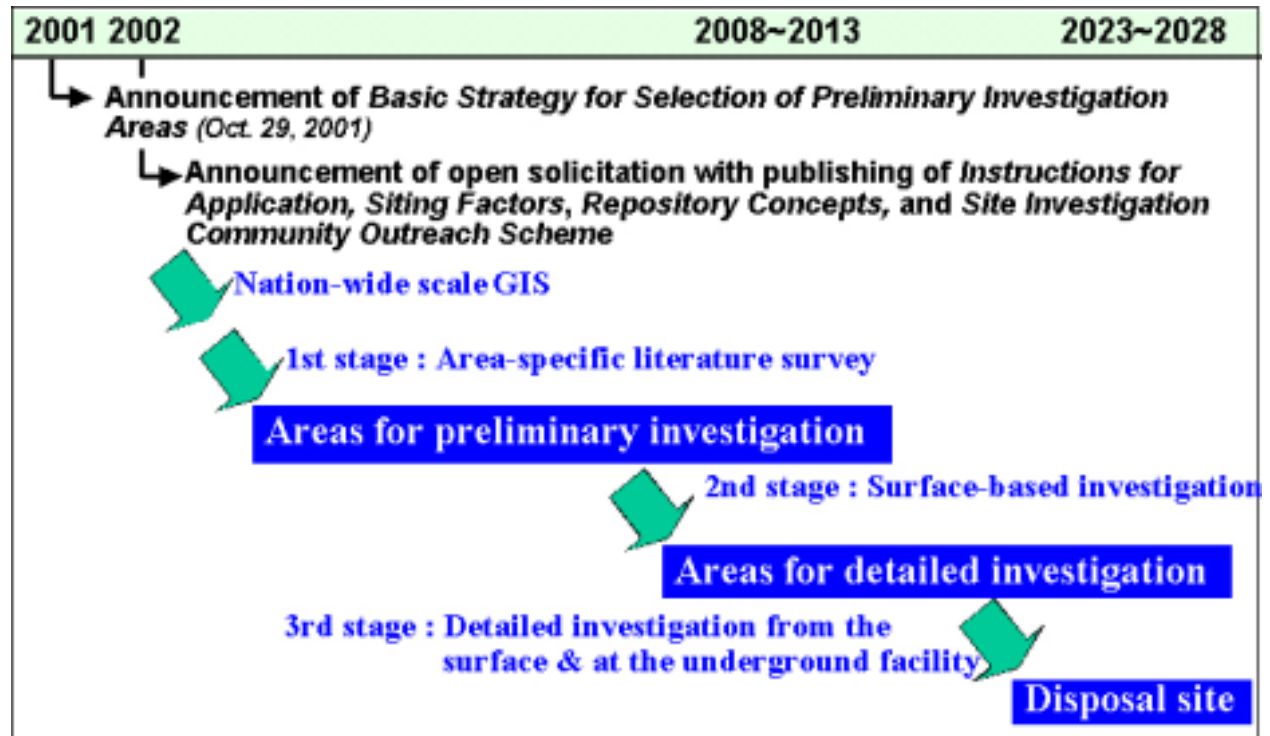
Fig. 2. NUMO's strategy for stepwise site selection process
