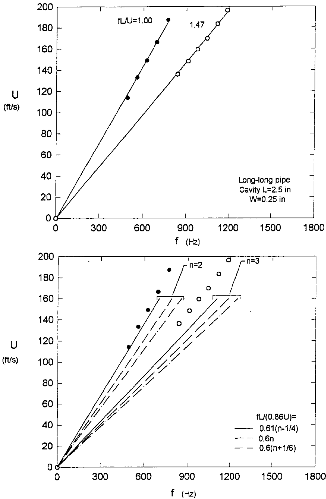
Figure 6c: Plots of values of frequency corresponding to amplitude peaks in Figure 4e. Top plot shows lines corresponding to the best fit of the dimensionless frequency fL/U through each set of data points. Bottom plot shows lines corresponding to three different correlations for fL/U . Velocity U corresponds to the time-mean centerline velocity at the center of the pipe, i.e., U = \bar{u}_m . In the lower plot, the bulk velocity of the pipe flow, 0.86U , is employed as the normalization velocity.
