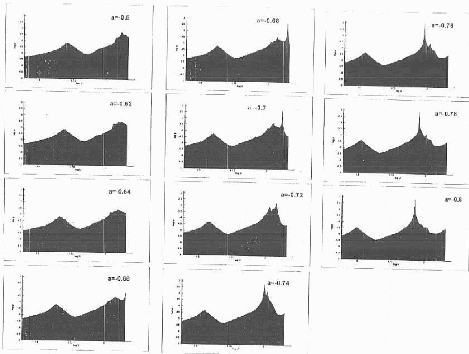
68 Figure 13b: Vertical cuts through the plot of Figure 13a. All cuts are along a line of constant Strouhal number fL/U , but at different values of a lying between the extreme values defined in Figure 13a.
