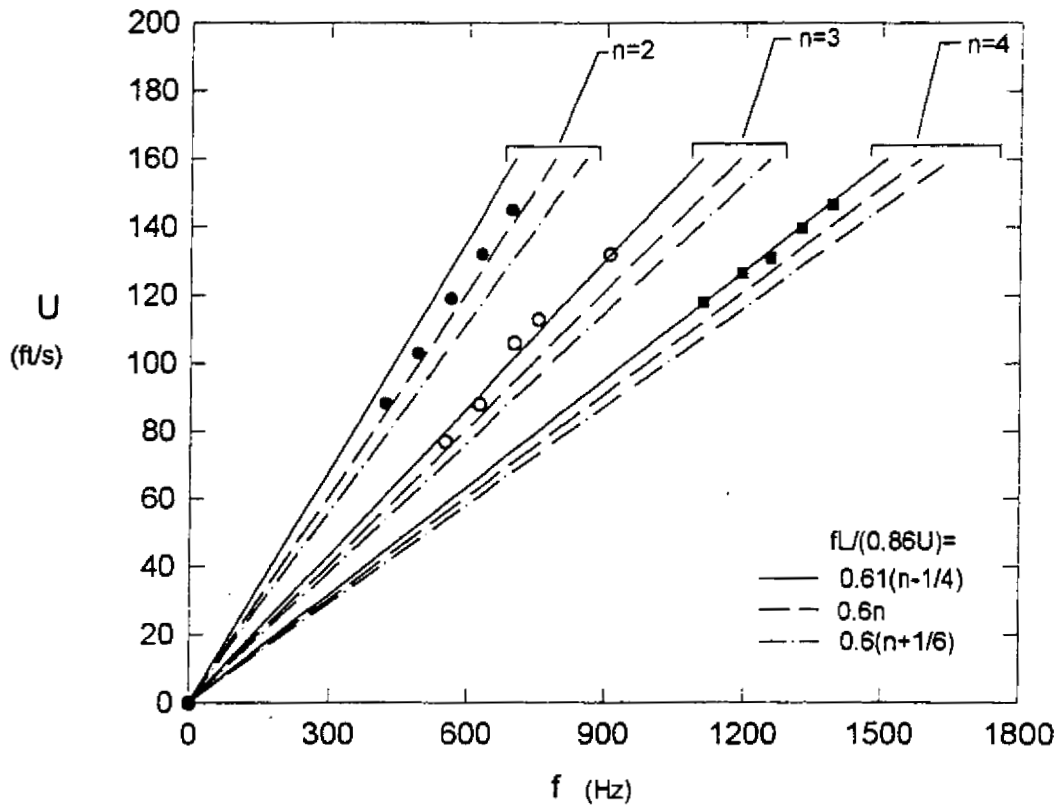
Figure 6b: Plots of values of frequency corresponding to amplitude peaks in Figures 4c and 4d. Top plot shows lines corresponding to the best fit of the dimensionless frequency fL/U through each set of data points. Bottom plot shows lines corresponding to three different correlations for fL/U . Velocity U corresponds to the time-mean centerline velocity at the center of the pipe, i.e., U = \bar{u}_c . In the lower plot, the bulk velocity of the pipe flow, 0.86 U , is employed as the normalization velocity.
