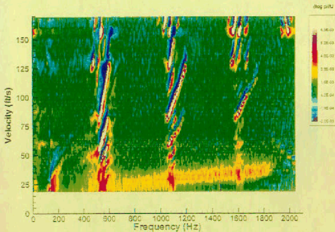
Figure 5b: Plan view of logarithmic pressure amplitude as a function of velocity and frequency (top image), and plan view of magnitude of the derivative of the logarithmic pressure amplitude with respect to velocity, \partial(\log p)/\partial U (bottom image). Cavity length L^* = L/D = 2.5 and depth W^* = W/D = 1.25 , where D is pipe diameter. Short pipes of equal length are located at either end of the cavity.
