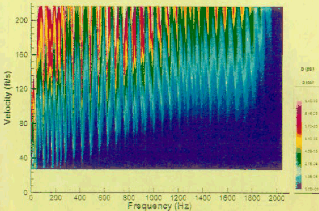
Figure 4f: Isometric view (top image) and plan view (bottom image) of pressure amplitude as a function of frequency and velocity. Cavity length L^* = L/D = 2.5 and depth W^* = W/D = 0.125 , where D is pipe diameter. Long pipes of equal length are located at either end of the cavity.
