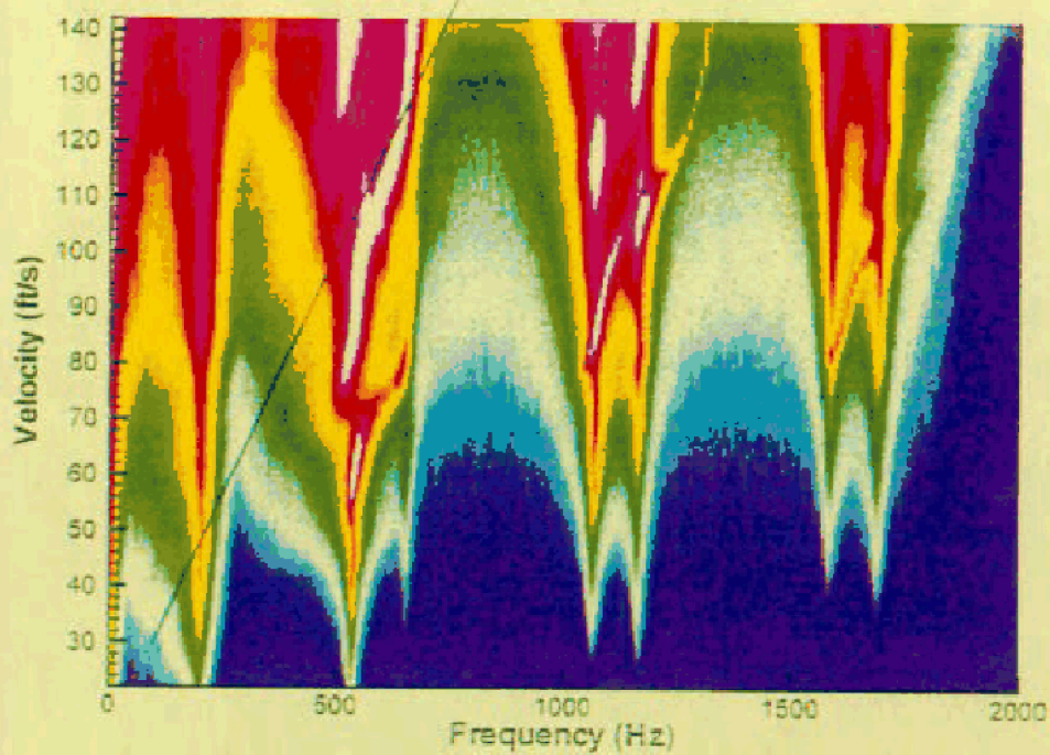
Figure 5c: isometric view (top image) and plan view (bottom image) of pressure amplitude as a function of frequency and velocity. Line shown on plan view represents a fit through peak values of pressure amplitude. Cavity length L^* = L/D = 2.5 and depth W^* = W/D = 0.5 , where D is pipe diameter. Short pipes of equal length are located at either end of the cavity.
