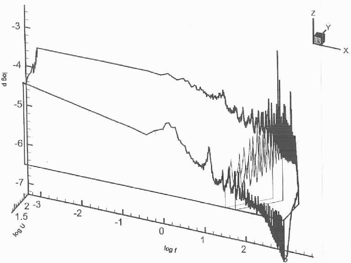
Figure 11b: Three-dimensional representation of vertical cuts defined by extreme values of a in Figure 11a. Bold lines represent spectra. Thin lines are vertical cuts coincident with the constant value of a in Figure 11a. Logarithmic values of parameters are employed.
