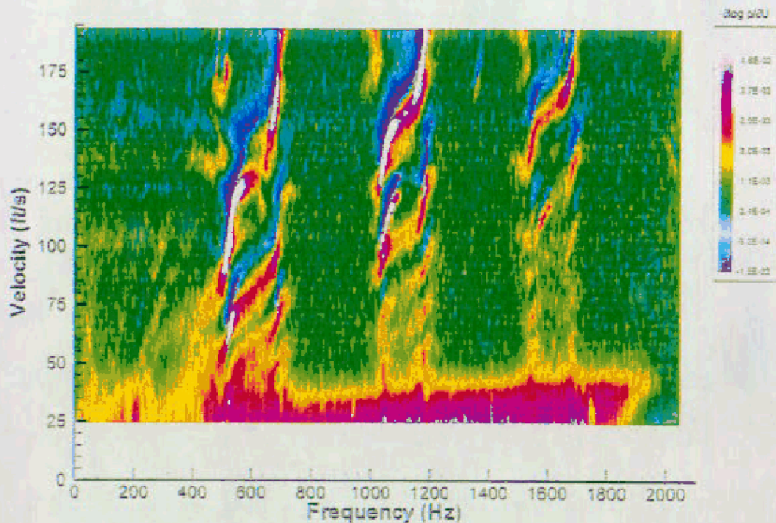
Figure 5f: Plan view of logarithmic pressure amplitude as a function of velocity and frequency (top image), and plan view of magnitude of the derivative of the logarithmic pressure amplitude with respect to velocity, \partial \log p / \partial U (bottom image). Cavity length L = L/D = 2.5 and depth W = W/D = 0.25 , where D is pipe diameter. Short pipes of equal length are located at either end of the cavity.
