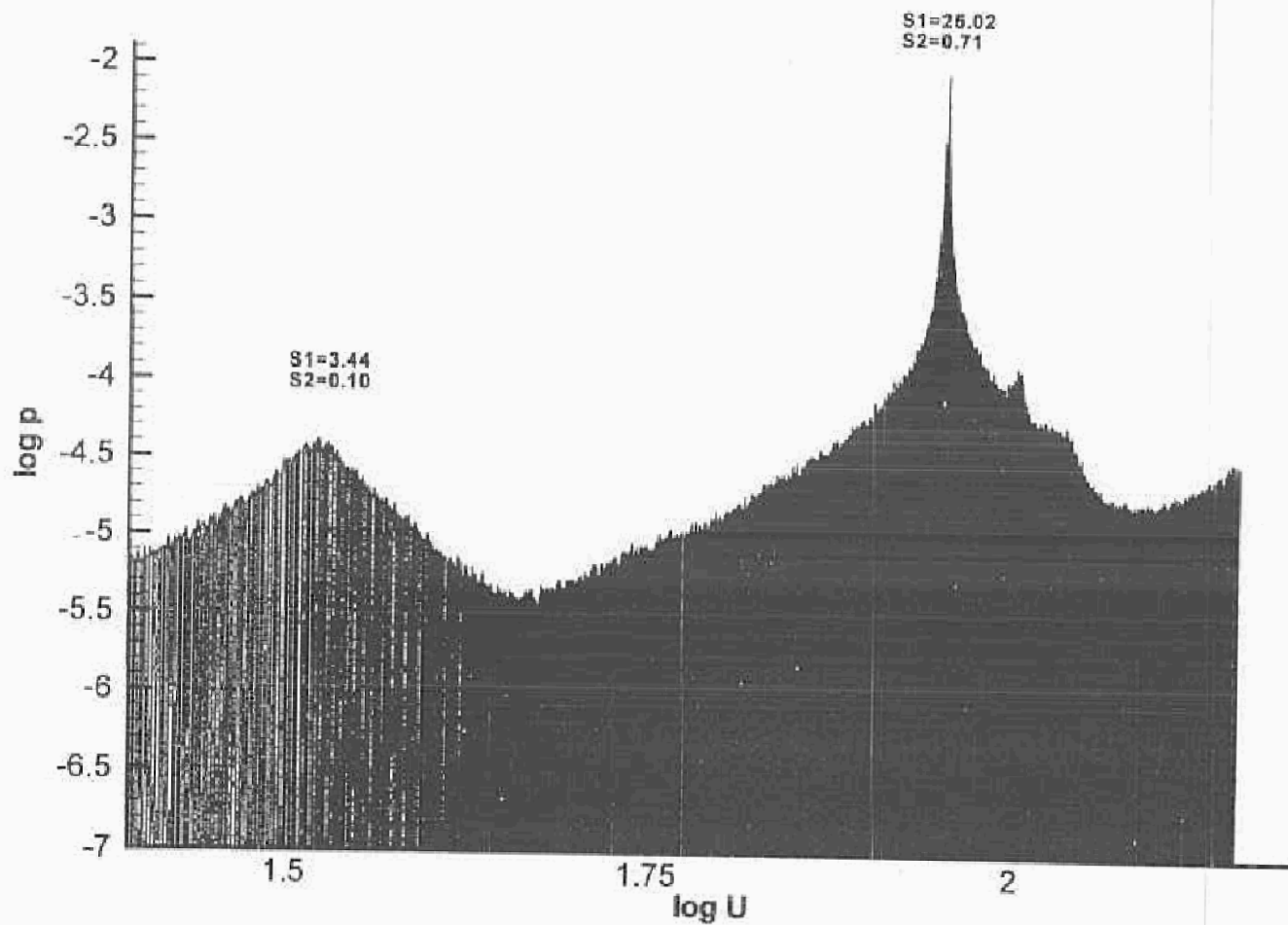
Figure 13c: Zoomed-in view of vertical cut selected from series of Figure 13b. Parameters S_1 and S_2 are sharpness factors analogous to Q-quality factors.
