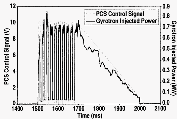
Fig. 3. Gyrotron output power sufficiently follows complex PCS control signals.
