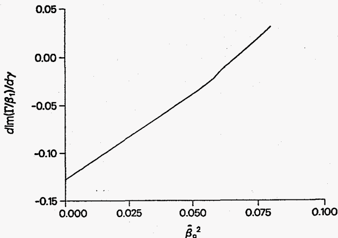
Figure 3: Sensitivity of phase to beam energy for medium gain ( C = 0.1 ), low energy ( \gamma = 2 ) case as a function of the space-charge wavenumber, for a detuning \Delta = -50 \text{ m}^{-1} .
