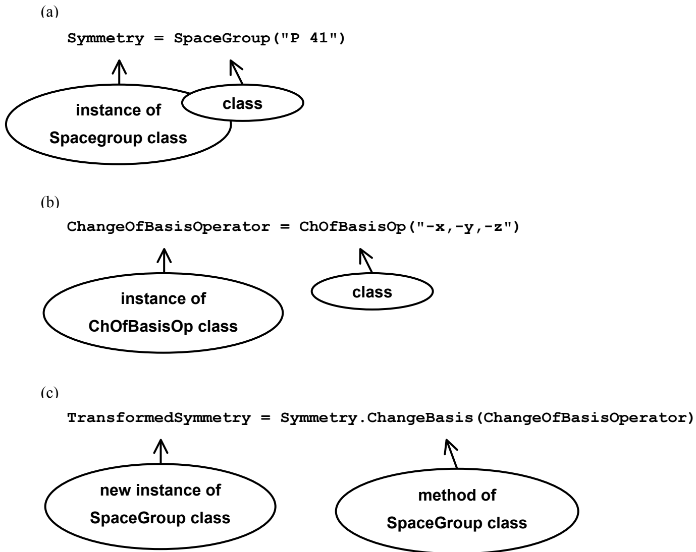
Figure 9: Example (using Python syntax) for expressions in an object-oriented programming language. (a) The Symmetry object is an instance of a class for the handling of space group symmetry ( Spacegroup ). (b) ChangeOfBasisOperator is another object that is an instance of a class for the handling of change-of-basis matrices ( ChOfBasisOp ). (c) ChangeBasis is a method of the space group class that applies the given change-of-basis matrix to transform the symmetry operations stored in the Symmetry object. The result is returned as a new, dynamically allocated instance of the space group class: the object TransformedSymmetry . Both Symmetry and TransformedSymmetry exist simultaneously after the expression is evaluated and can be independently manipulated.
