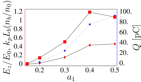
Figure 4.4: (Color) Bunch charge Q in pC (right vertical axis, stars), k_p L_b (n_b/n_0) (left vertical axis, squares) and normalized axial electric field E_z/E_0 (left vertical axis, points) generated by the electron bunch alone versus a_1 with \lambda_0 = 0.8 \mu\text{m} , L_0 = 9\lambda_{p0}/4 , r_0 = \lambda_{p0} = 40 \mu\text{m} , a_0 = 1 , z_t = 240 \mu\text{m} , L_t = \lambda_{p0} , \tau_t = 30\% and ct = 147 k_{p0}^{-1} \simeq 935 \mu\text{m} after injection
