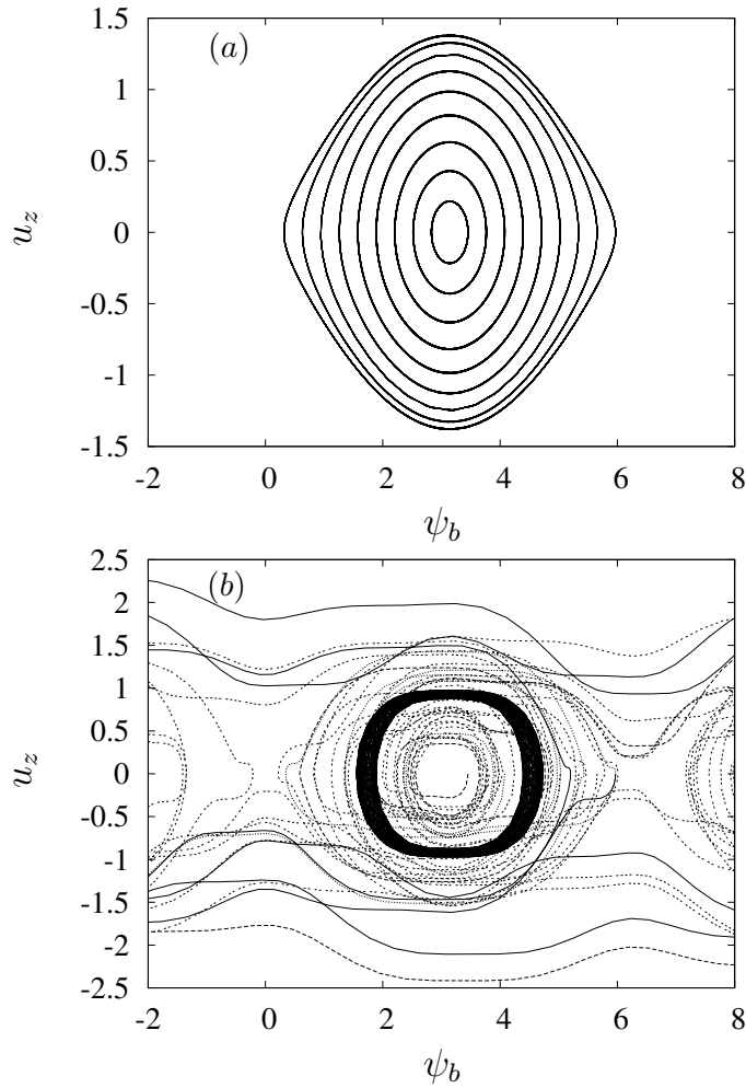
Figure 3.20: Phase space orbits (u_z, \psi_b) of test electrons in two counterpropagating laser pulses with (a) circular polarization and (b) linear polarization. Here both lasers are infinite plane waves with \langle a_0^2 \rangle = \langle a_1^2 \rangle = 0.5 , i.e., equal time-averaged intensities.
