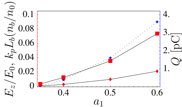
Figure 4.2: (Color) Bunch charge Q in pC (right vertical axis, stars), k_p L_b(n_b/n_0) (left vertical axis, squares) and normalized axial electric field E_z/E_0 (left vertical axis, points) generated by the electron bunch alone (here the laser contribution is not included) versus a_1 with \lambda_0 = 0.8 \mu\text{m} , L_0 = 9\lambda_{p0}/4 , r_0 = \lambda_{p0} = 40 \mu\text{m} , a_0 = 1 , homogeneous plasma, i.e., no density ramp and ct = 47 k_{p0}^{-1} \simeq 300 \mu\text{m} after injection
