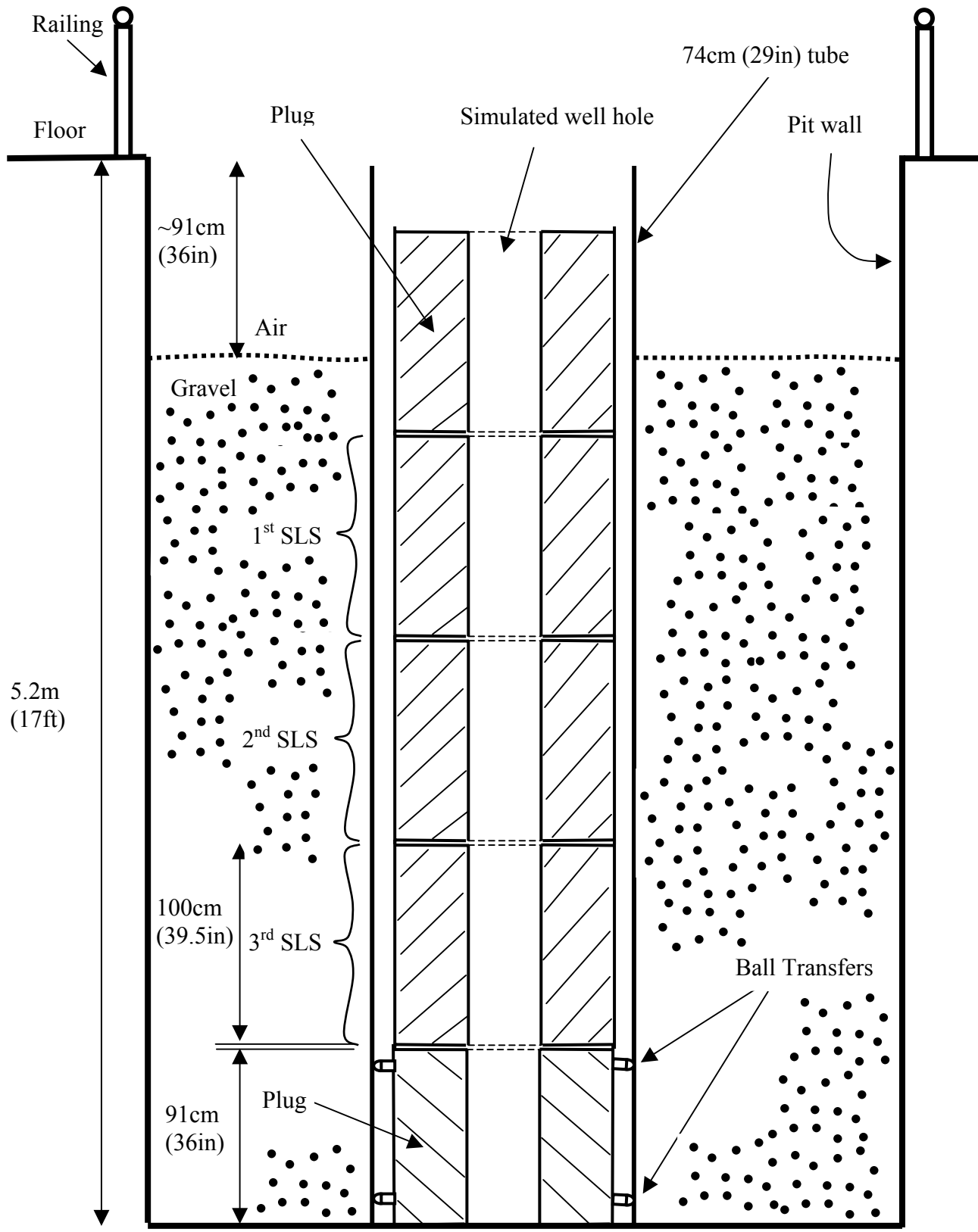
Figure 3: A stack of surrogates is shown placed within the 29in tube in the pit. All surrogates have the same dimensions. Plugs are shown at the top and bottom that are surrogates filled with concrete. Note: This diagram is not to scale.
