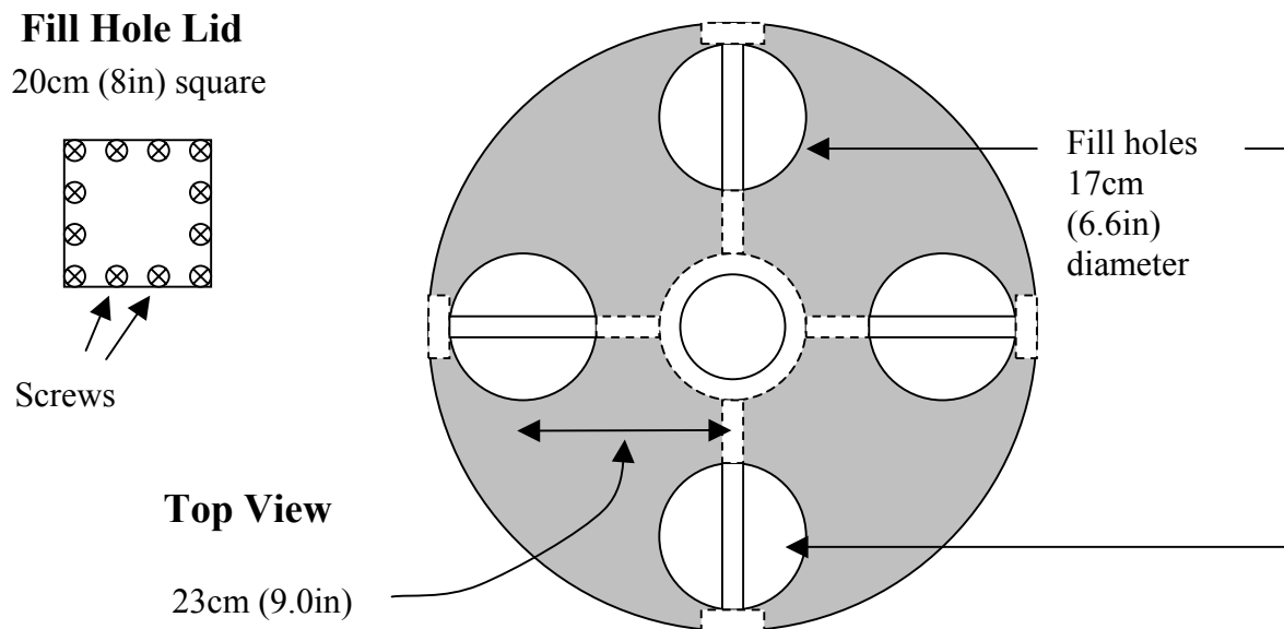
Figure 2: The design of an SLS. Each SLS is constructed from a modified 83gallon drum. Three pieces of penetrometer pipe run down along the longitudinal axis, while samples can be placed into the sample ports around the periphery of the surrogate. The surrogate is filled through the fill holes in the drum lid. The fill holes are to be covered when a surrogate is filled. Note: Not to scale.
