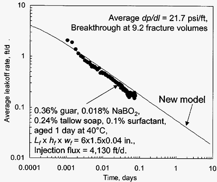
Fig. 14—Leakoff results for a guar-borate gel.
