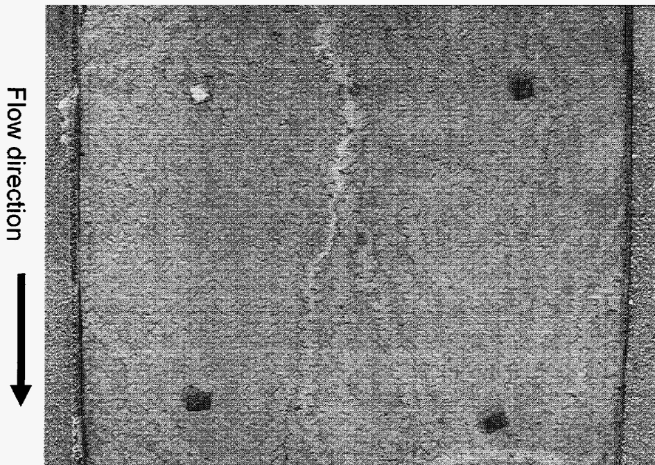
Fig. 15—Wormhole pattern for a guar-borate gel.
