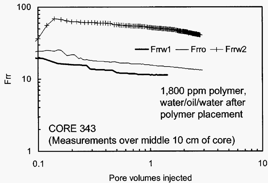
Fig. 54—Residual resistance factors in Core 343.
