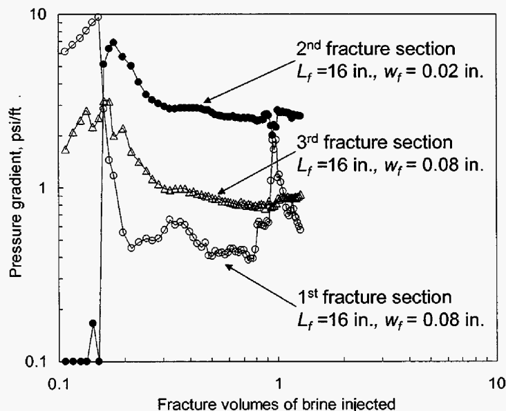
Fig. 31—Pressure gradients during brine injection after gel placement ( 100 \text{ cm}^3/\text{hr} ).
