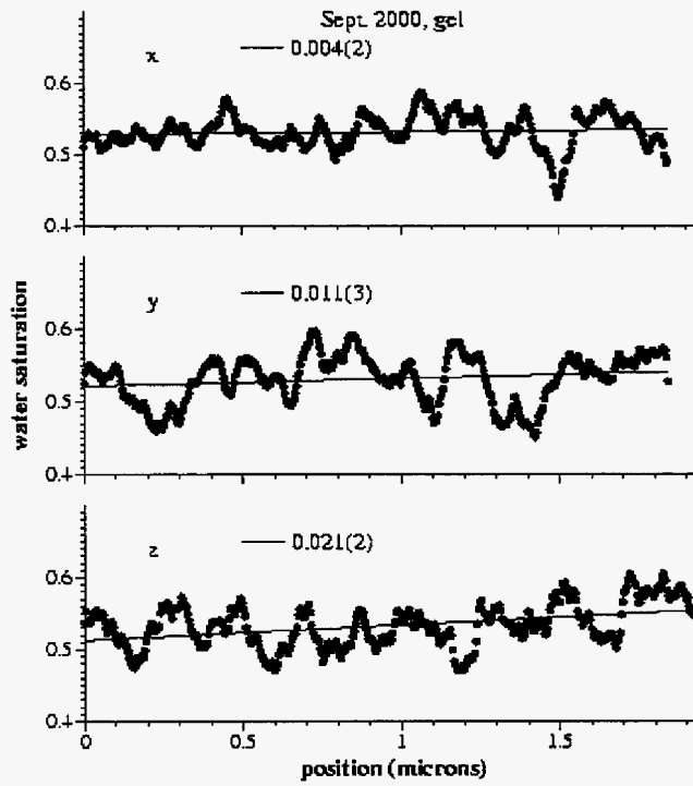
Fig. 81—Saturation gradients in the imaged volume just after gel placement.
