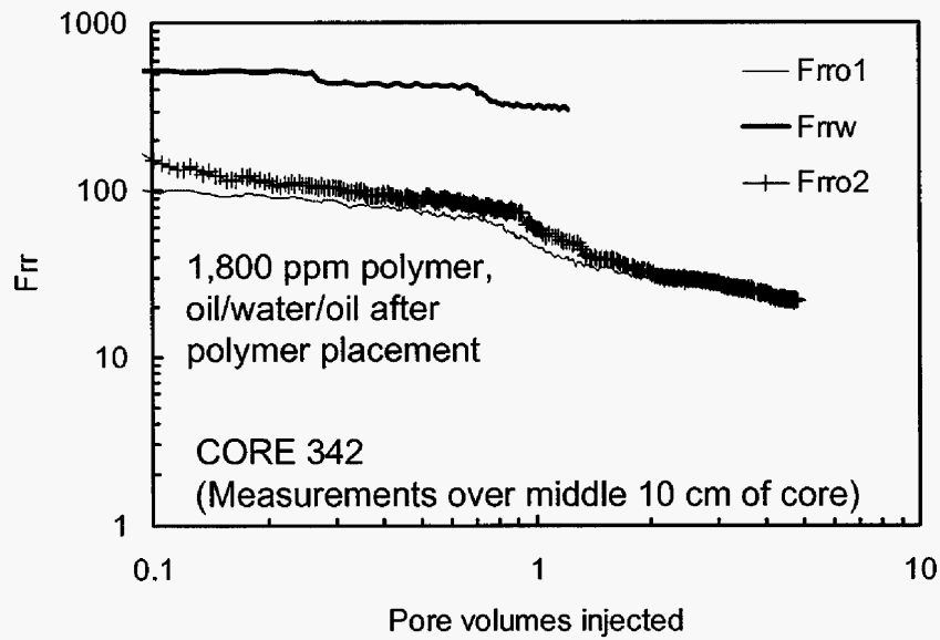
Fig. 53—Residual resistance factors in Core 342.
