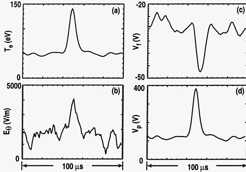
FIG. 5. Conditional average results for (a) T_e , (b) E_{\theta} , (c) V_f , (d) V_p showing that (1) the plasma structures are charged positively, (2) contain and convect substantial amounts of energy and (3) a positive radial electric field exists inside them.
