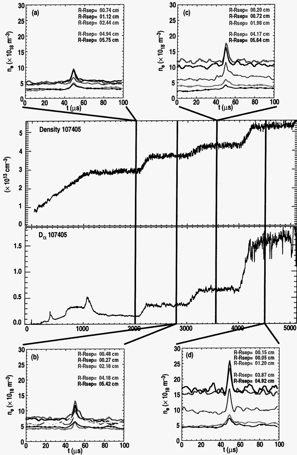
FIG. 8. L-mode discharges where the density was increase stepwise (central frame) allow comparison of IPO density vs discharge/edge density (insets) and a relation of proportionality is found.
