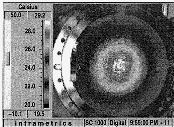
Fig. 1. A CVD diamond window can handle the peak intensity of a Gaussian 1 MW rf beam. This IR image shows the profile of the beam on a target 50 cm from the window.
