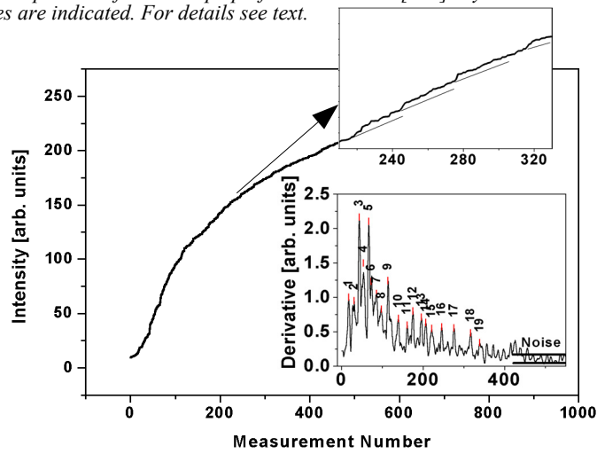
Figure 6: Detection of single gold atoms from Z-contrast images. Intensity maxima are extracted from the HAADF image of figure 2 and sorted according to measurement. The curve exhibits discrete jumps (top inset) that can be amplified by taking the derivative of the curve (bottom inset).
