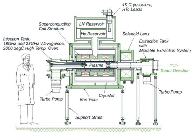
Figure 1: Mechanical layout of the VENUS ion source and cryogenic system.
