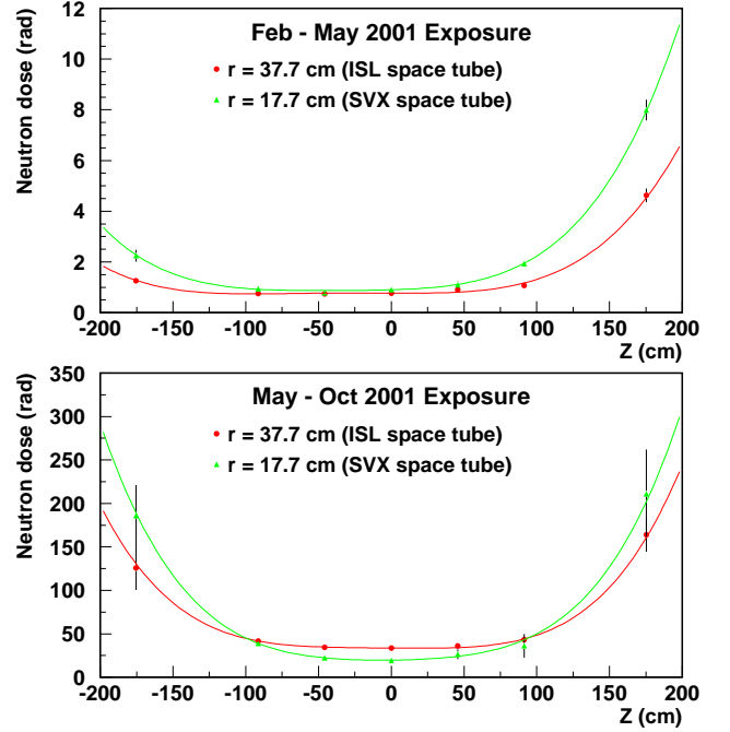
Fig. 8. Neutron radiation dose as a function of z for the two exposure periods. Top: the pattern during the first exposure period, dominated by proton beam losses (proton direction is +z ). Bottom: the dose during the second exposure period, dominated by proton-antiproton collisions around z = 0 .
