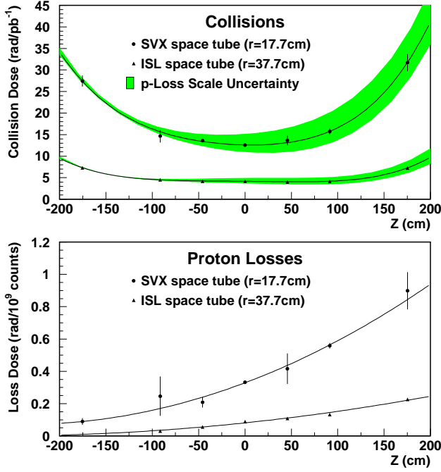
Fig. 7. Ionizing radiation dose, as a function of z , due to p\bar{p} collisions (top), and due to beam losses (bottom). The shaded band represents the systematic uncertainty from the beam loss measurements. For the second exposure period, the ratio of proton losses to collisions was 3.9 \times 10^9 counts / \text{pb}^{-1} .
