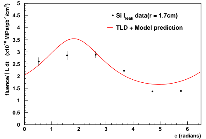
Fig. 10. Fluence (particles per unit area) per \text{pb}^{-1} of delivered luminosity, as a function of the azimuthal angle around the beam line. The points are from the leakage current measurements at the innermost silicon layer. The curve is the prediction of the radiation field model constructed from the TLD measurements.
