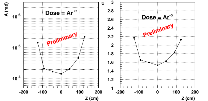
Fig. 9. Fit parameters of the radiation field model in Equation 3; normalization (left) and power law exponent (right) as a function of z .
