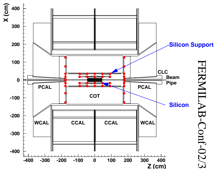
Fig. 1. Elevation view of the Collider Detector at Fermilab, with its detector component closest to the proton-antiproton collisions shown. The circles in the tracking volume denote the locations where we measure the radiation dose.
