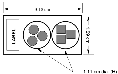
Fig. 4. A 0.79 mm thick FR-4 TLD holder. TLD-700 (round) and TLD-600 (square) dosimeters are kept in place by 76 \mu\text{m} thick kapton tape.
