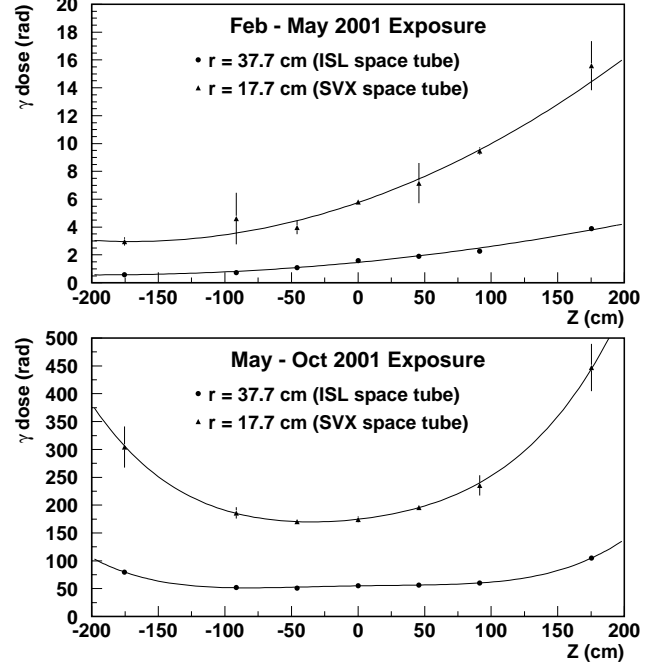
Fig. 6. Ionizing radiation dose as a function of z for the two exposure periods. Top: the pattern during the first exposure period, dominated by proton beam losses (proton direction is +z ). Bottom: the dose during the second exposure period, dominated by proton-antiproton collisions around z = 0 .
