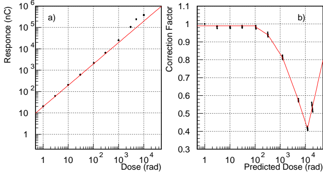
Fig. 5. a) Response of TLD-700 dosimeters to ionizing radiation as a function of received dose; note the super-linear behavior for doses above 100 rad. b) The non-linearity correction factor as a function of the dose estimated from the linear-response assumption.
