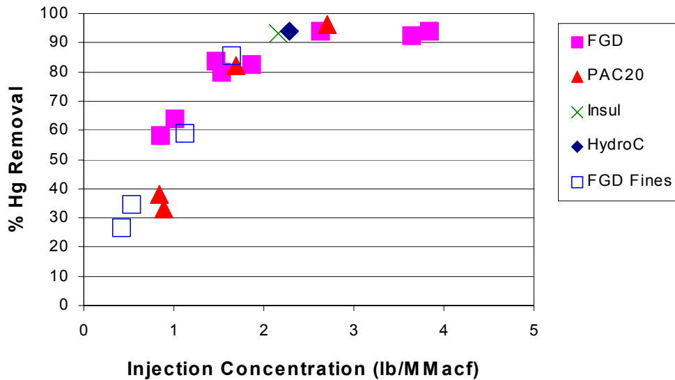
Fig. 3. Mercury Removal Trends Across COHPAC as a Function of PAC Injection Concentrations.
