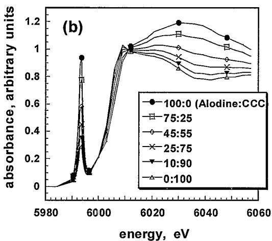
Figure 8. (a) Time-lapse XANES measurements to monitor changes in both electrolyte and a CCC simultaneously during solution exposure for AA 1100. (b) Calculated XANES spectra based on those of the Alodine solution (curve 1 in Figure 8(a)) and of the CCC (curve 6 in Figure 8(a)).
