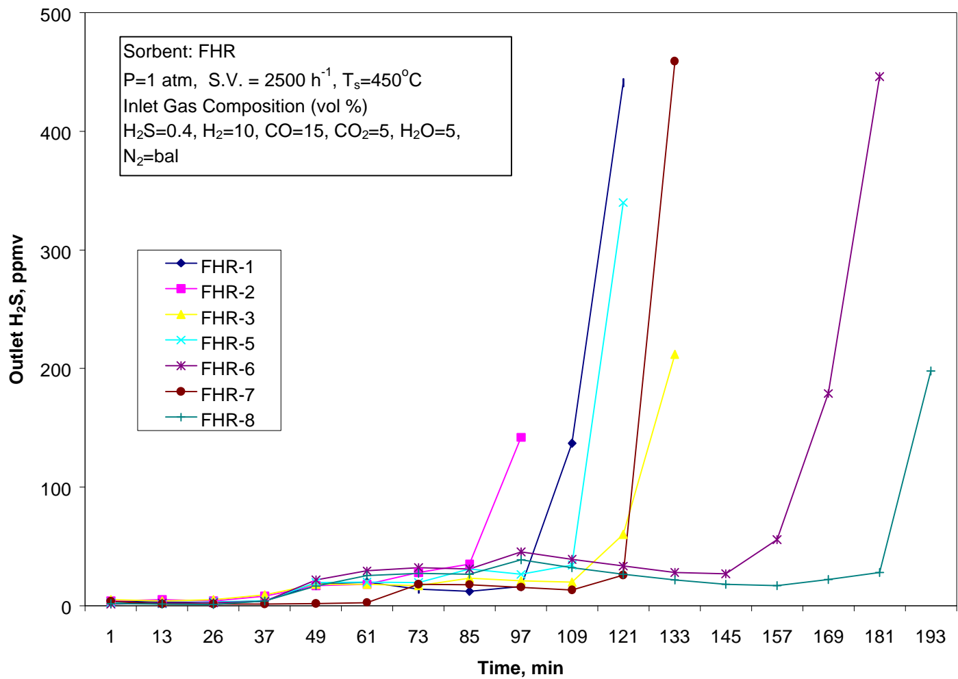
Figure 2. H 2 S Breakthrough Curves in Successive Sulfidation Cycles of FHR Sorbents
