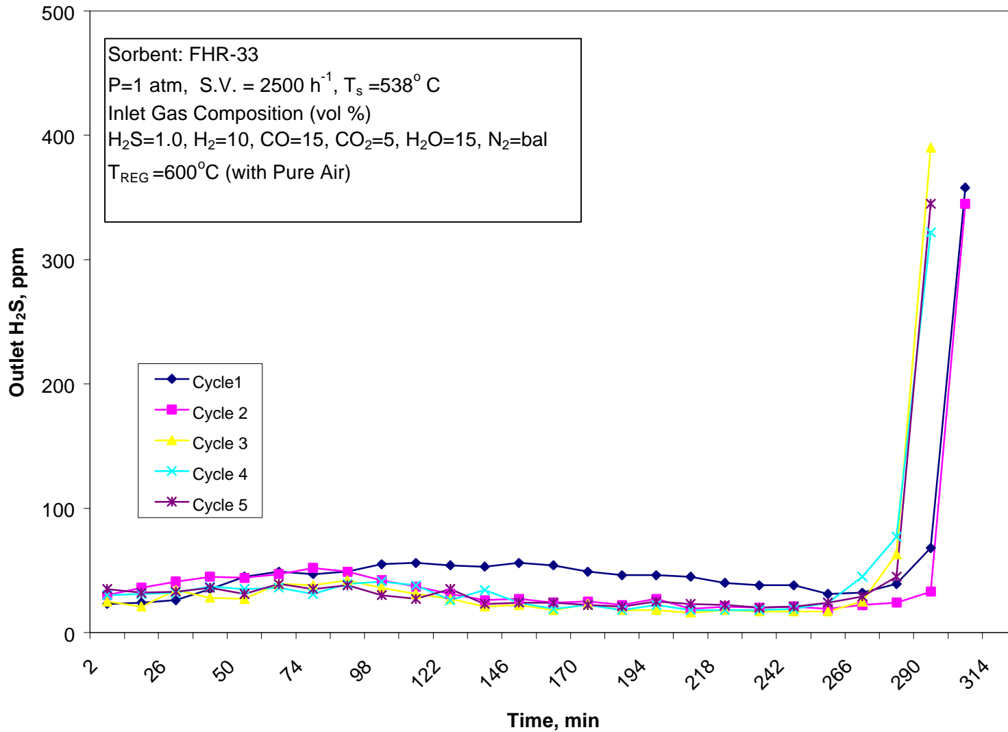
Figure 1. H 2 S Breakthrough Curves in Successive Sulfidation Cycles of Sorbent FHR-33
