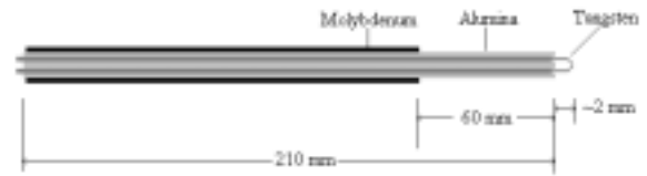
Fig. 3 Floating emissive probe design.
