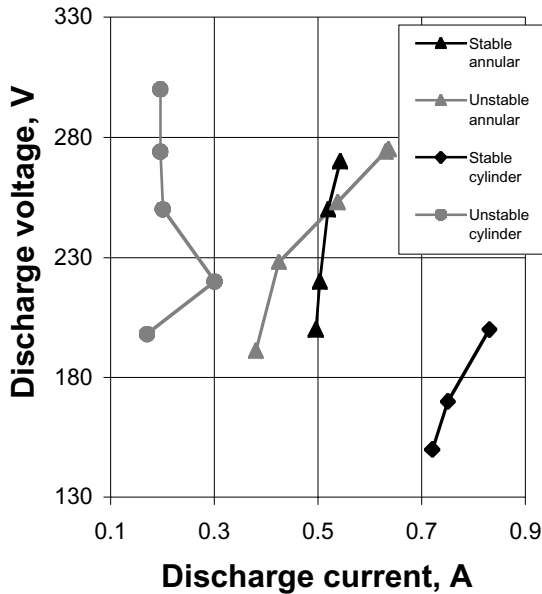
Fig. 14. Discharge voltage versus current characteristics for the 3 cm thruster cylindrical and annular thrusters in stable and unstable regimes at 0.3 mg/ sec. The cathode flow rate is 0.2 mg/s.
