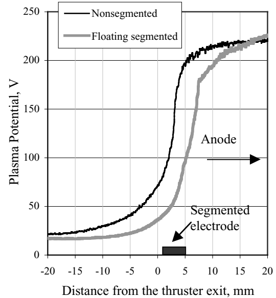
Fig. 6 Plasma potential profiles measured for segmented and non segmented thruster configurations along the channel median.
