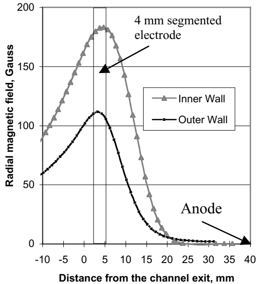
Fig. 2 Magnetic field distribution and placement of the graphite segmented electrode.
