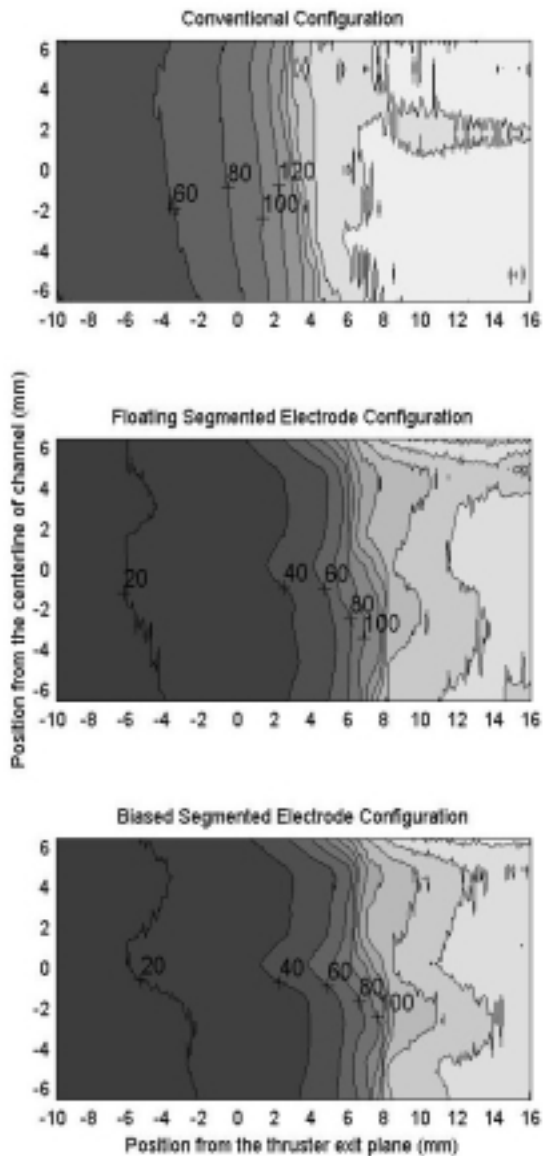
Fig. 7 Plasma potential contours (20 V step) obtained for three thruster configurations, non segmented, segmented floating and segmented biased at discharge voltage of 250 V and mass flow rate of 1.7 mg/s. Note that irregularities at larger potentials and along the channel median (segmented cases) may be caused by probe induced perturbations of the plasma.
