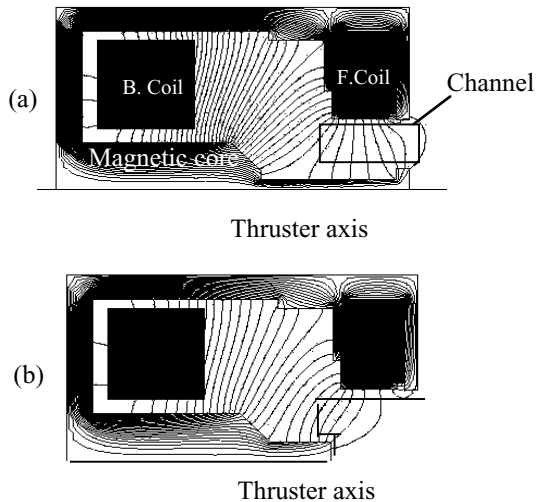
Fig. 9 Magnetic circuit of the annular thruster (a) and cylindrical (b) thruster. The channel OD diameter is 2.6 cm.
