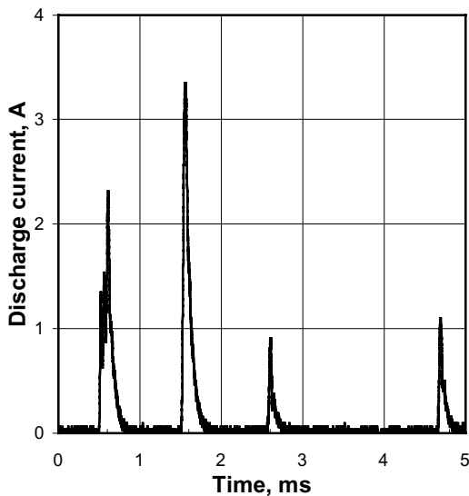
Fig. 11 A typical trace of the discharge current in the unstable regime.
