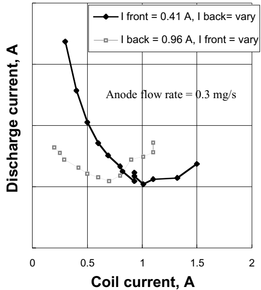
Fig. 12 The effect of the magnetic field on the discharge current for the annular 3 cm thruster.
