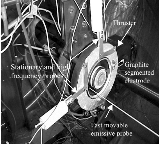
Fig. 1 Segmented electrode Hall thruster and probe setup
