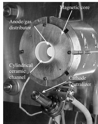
Fig. 8 A 3 cm cylindrical Hall thruster.
