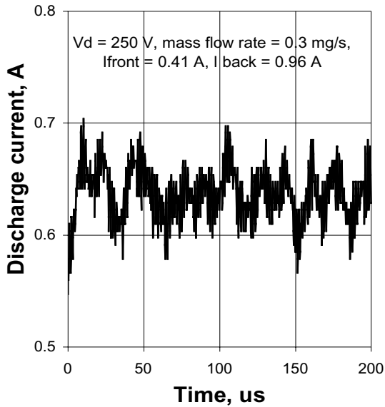
Fig. 13. Discharge current oscillations measured for the annular thruster in the stable regime.
