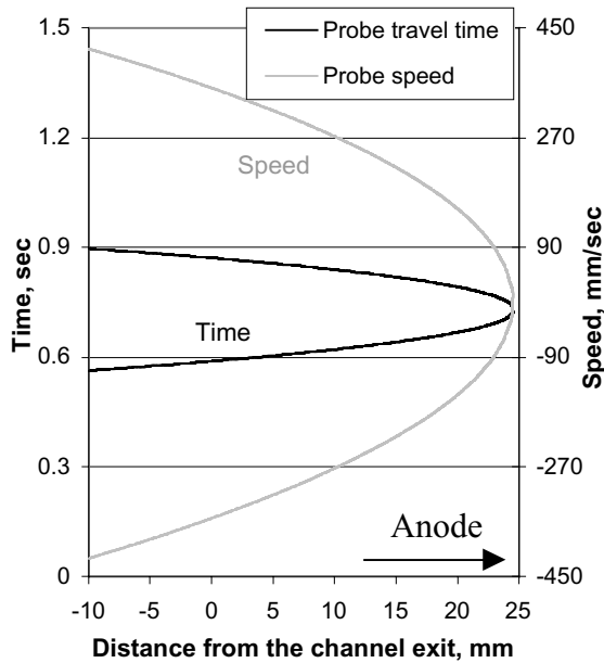
Fig. 4 Dynamic characteristics of the probe positioning system.
