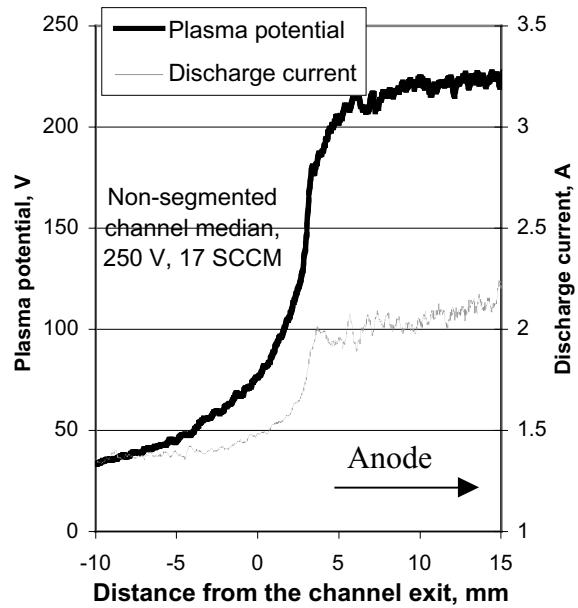
Fig. 5 Plasma potential distribution measured by fast emissive probe relative to the ground and probe induced perturbations of the discharge current.
