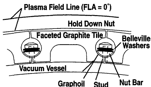
Fig. 2. Horizontal section of centerpost tiles.
