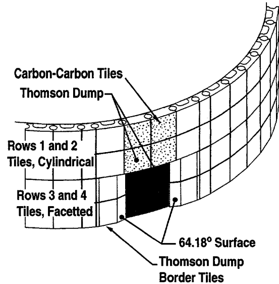
Fig. 4. Isometric view of Thomson dump and centerpost.
