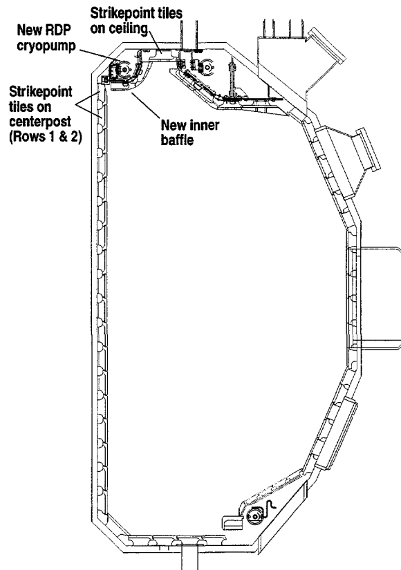
Fig. 1. Vertical cross section of DIII-D.
