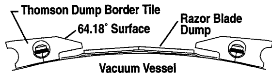
Fig. 5. Horizontal section of Thomson dump on centerpost of vacuum vessel.
