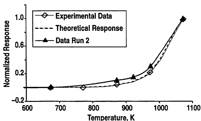
Fig. 3. Normalized results for blackbody response.
