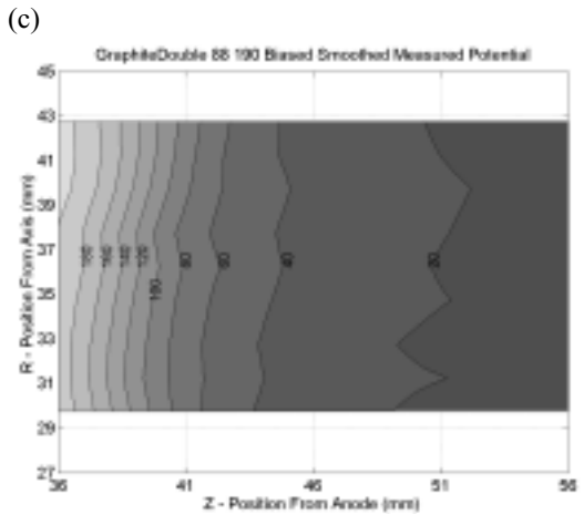
Fig. 5 Plasma potential distribution measure for the single segmented, floating (a) and biased (b) and double segmented with the inner electrode biased (c) configurations. The thruster was operated with the magnetic field distribution shown in Fig. 2a. The channel exit is 46 mm from the anode.
