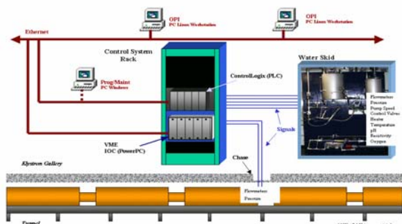
Figure 1: Resonance Control and Cooling System
