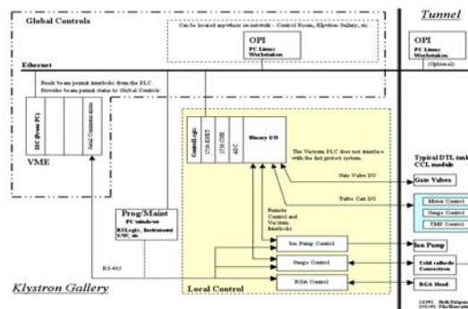
Figure 2: Vacuum System
