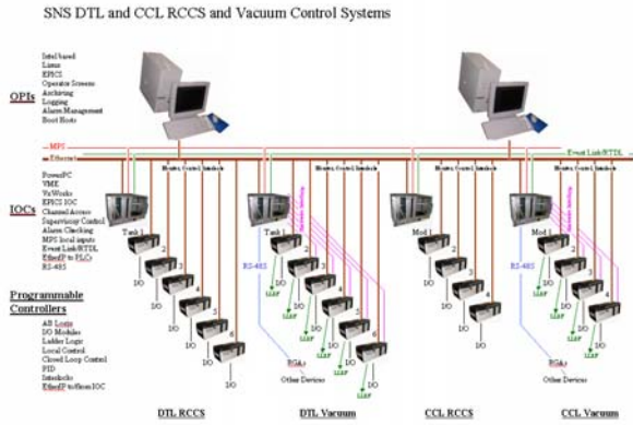
Figure 3: Network diagram of RCCS and Vacuum components
