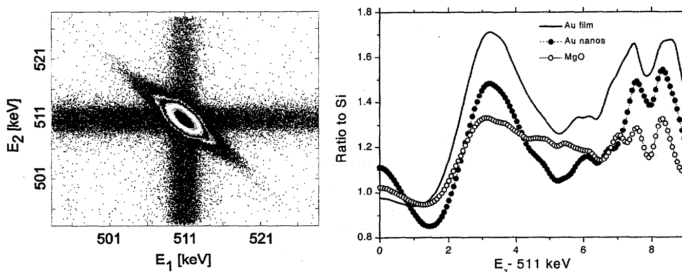
Figure 4 (left) Two-dimensional spectrum of annihilation radiation of positrons injected into a p-Si (100), with 8 \Omega -cm. The diagonal feature indicates the condition of E_1+E_2=1.022 MeV; (right) Normalized annihilation lines as a function of photon energy for Au nanoparticle layer (solid circles), MgO layer (open circles), and Au film (solid line).
