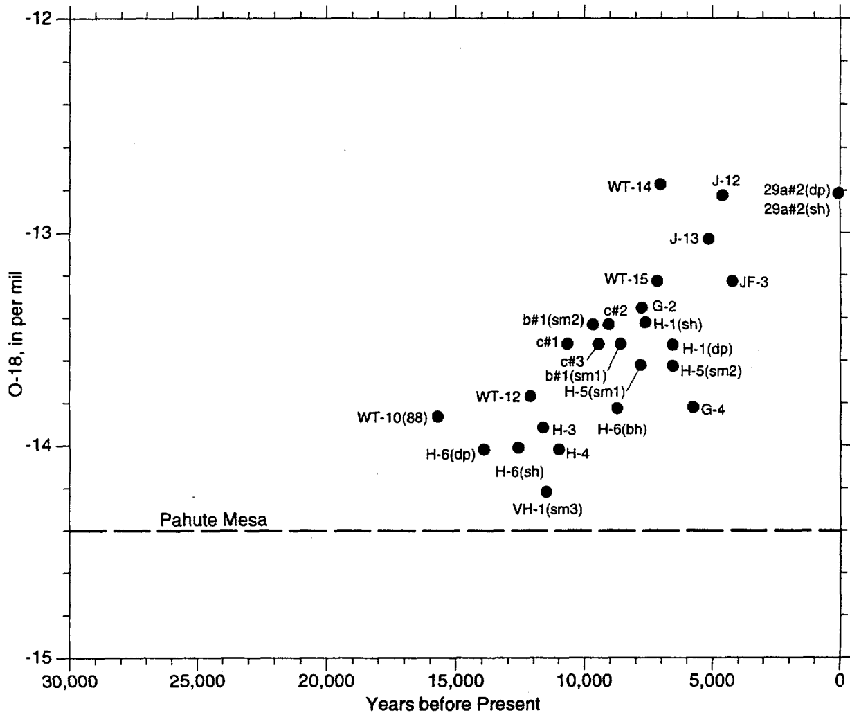
Figure DL-1 \delta^{18}\text{O} values in groundwaters with the Tertiary volcanics under Yucca Mountain and the alluvium of Fortymile Wash, plotted against their corrected \delta^{14}\text{C} ages (Kwicklis, 1997). Also shown is the average \delta^{18}\text{O} value of three well waters on Pahute Mesa, the possible recharge source for Yucca Mountain groundwater (Benson and Kieforth, 1989).
