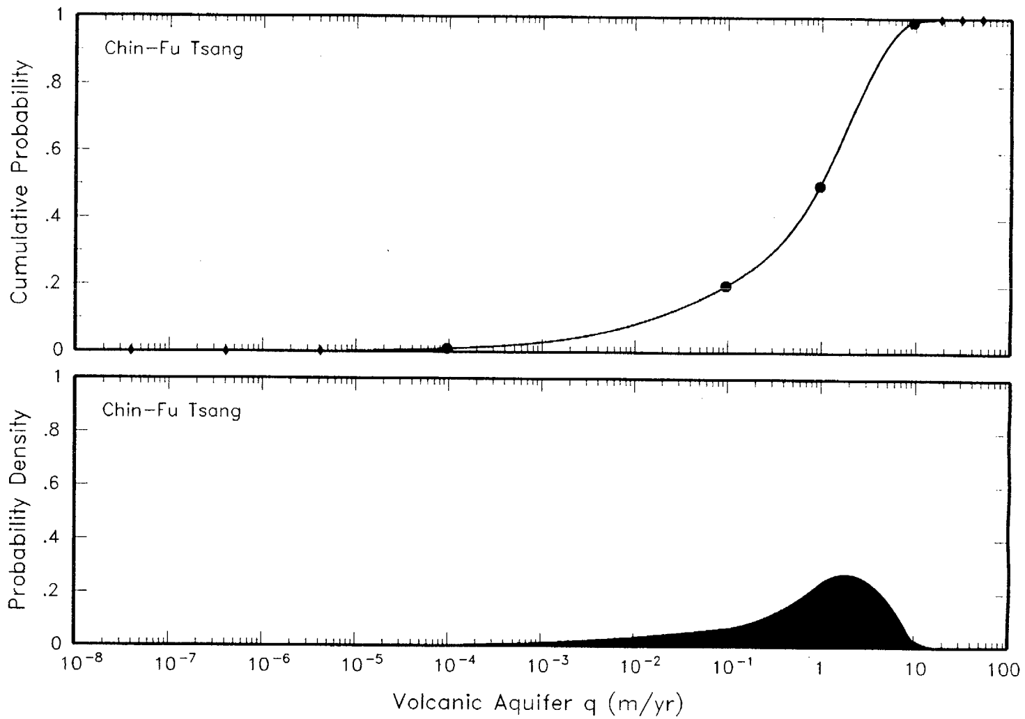
Figure 3-2a Distribution for volcanic aquifer specific discharge assessed by Chin-Fu Tsang
