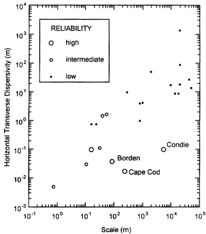
Figure LG-2a, b Horizontal and vertical transverse dispersivities (from Gelhar et al., 1992, figures 4 and 5).
