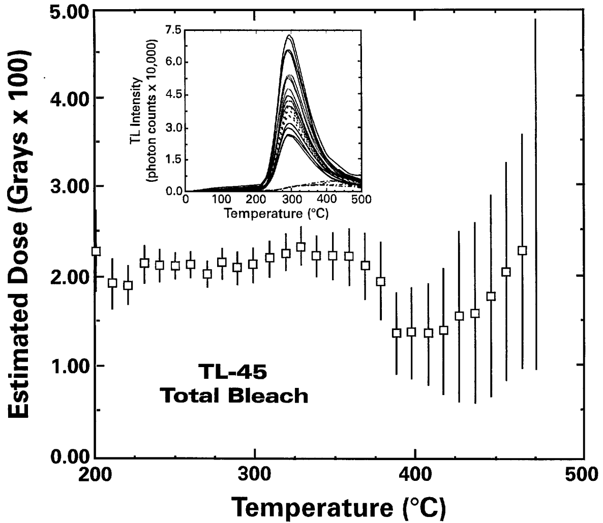
Figure 15: Estimated dose ( D_e ) versus temperature plot for sample TL-45 from SLD. See Figure 7 for details.
