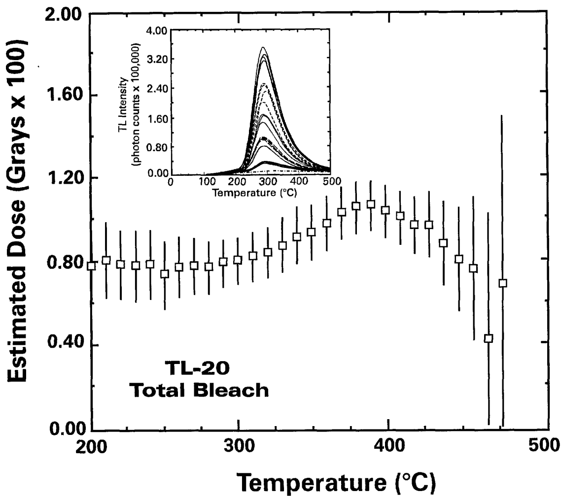
Figure 11: Estimated dose ( D_e ) versus temperature plot for sample TL-20 from CFD. See Figure 7 for details.
