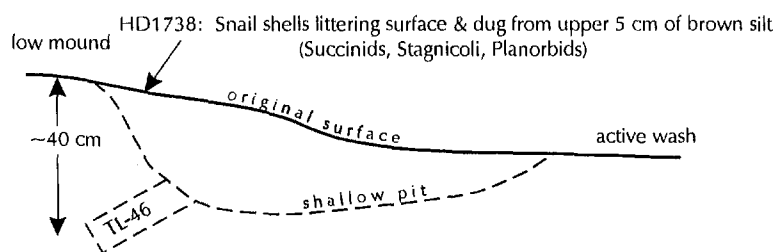
Figure 13: Schematic diagrams illustrating geological relations and geochronological data for two sites at SLD. Age determinations are from Tables 8, 9 and 10. All uncertainties are given at the 95% confidence level. Values following U-series ages are calculated initial ^{234}\text{U}/^{238}\text{U} ratios. TL ages are given for dose rates calculated at saturation-moisture contents followed parenthetically by the total range of ages calculated using different moisture contents and analytical uncertainties. A) Schematic cross-section of high-terrace spring deposits near Franklin Well. B) Schematic cross-section of brown silty deposits near the Amargosa River northwest of Franklin Well.
