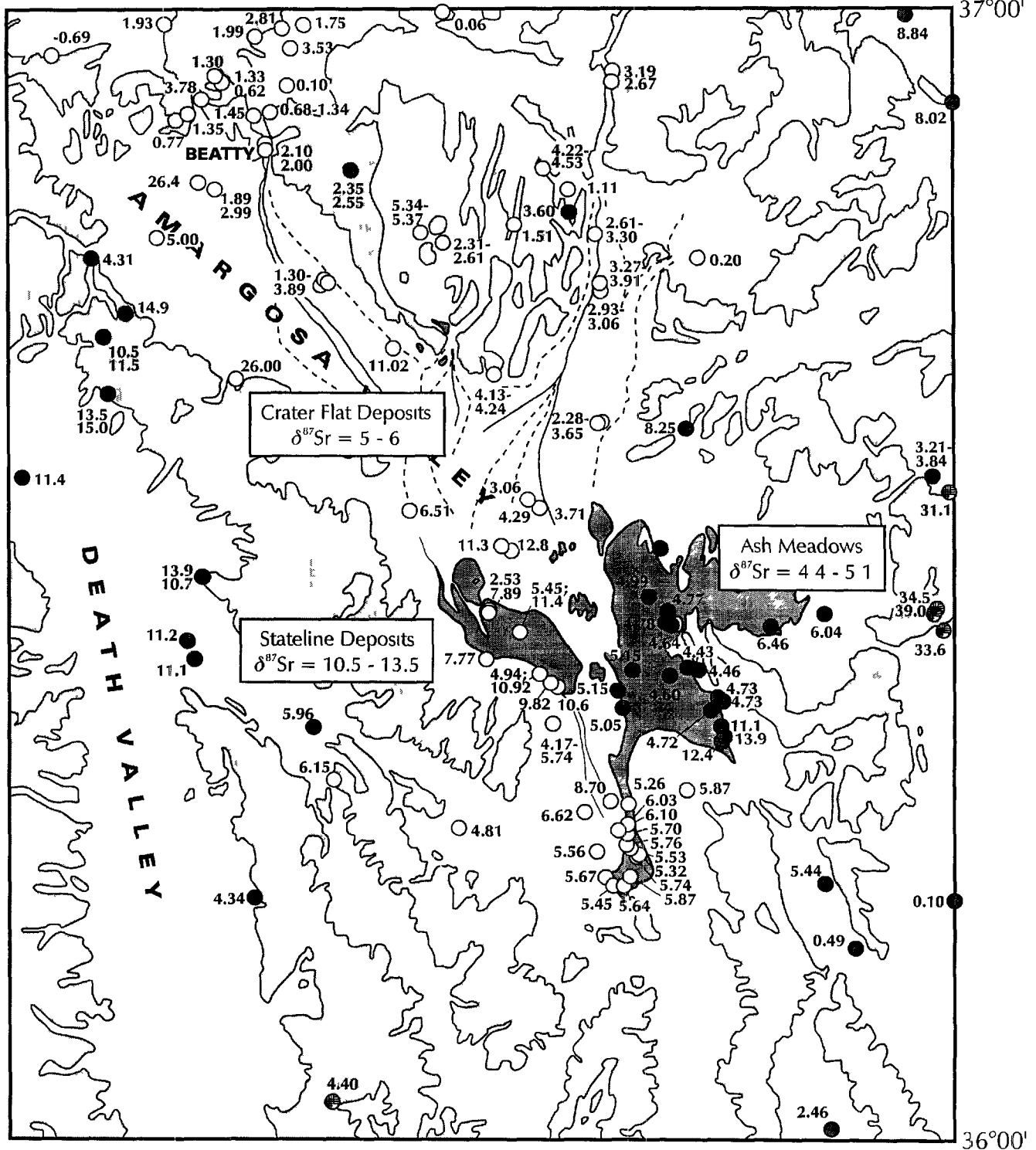
Figure 24 Location of wells and springs analyzed for \delta^{87}\text{Sr} (values in ‰ relative to sea-water = 0.70920) from waters. Bedrock ranges are shown in shaded patterns, and alluvial-filled valleys are shown unpatterned. Solid and dashed lines within alluvial valleys represent active channels and alluvial fan boundaries, boundaries. Dark circles represent sample sites classified as Paleozoic aquifer, open circles represent sample sites from volcanic or alluvium aquifers, and circles with hatch marks represent sites classified as Precambrian aquifer.
