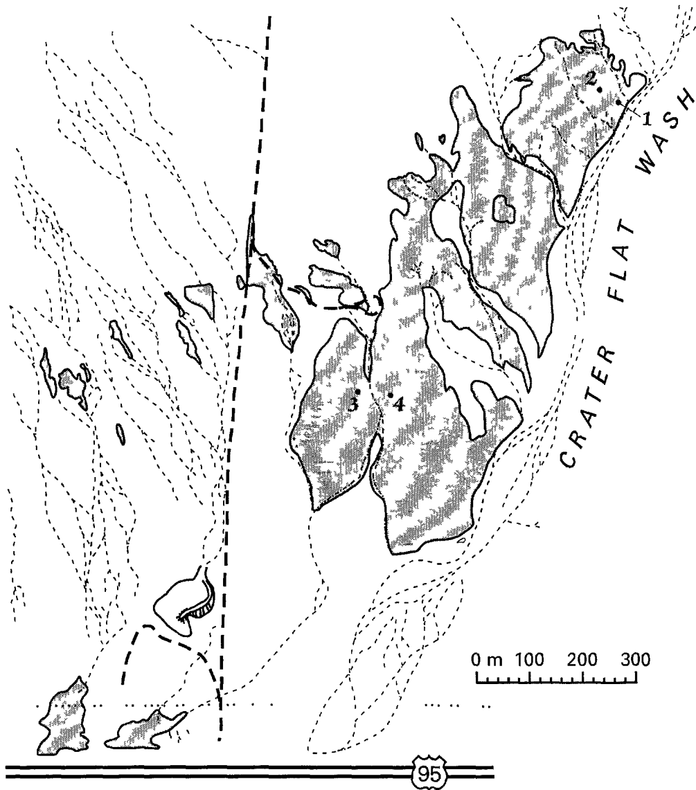
Figure 12. Sketch of air photos showing major morphologic features of the Crater Flat Wash deposit (CFW). Light-colored, fine-grained deposits are shown as light-shaded areas. Numbered sample stations are shown with small black circles. Dash-dot lines represent drainage channels.
