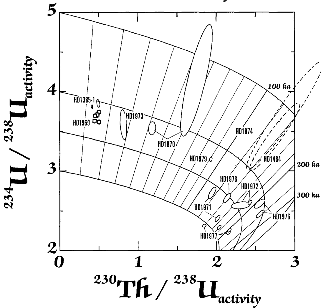
Figure 6 U-series evolution diagram showing U and Th isotopic results for LWD data having the least amount of analytical uncertainty due to detrital-Th corrections (i.e., lowest ^{232}\text{Th} contents). Diagram is described in Figure 5
