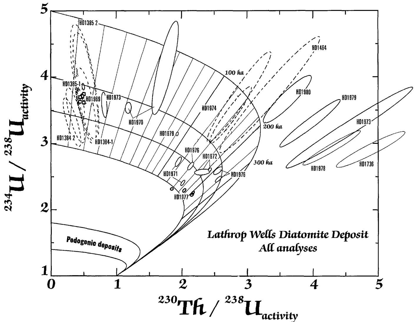
Figure 5 U-series evolution diagram showing U and Th isotopic data for all analyses from LWD. Curved lines leading from different ^{234}\text{U}/^{238}\text{U} values on the Y-axis to secular equilibrium values of ^{230}\text{Th}/^{238}\text{U} on the X-axis represent the foci of isotopic compositions during closed-system, temporal evolution of different materials with different initial uranium isotopic ratios (evolution lines). Straight, sub-parallel lines represent isochrons drawn at 10 ka intervals between 0 and 100 ka, 20 ka intervals between 100 and 200 ka, and 50 ka intervals between 200 and 300 ka. 95% confidence Error ellipses represent measured isotopic ratios corrected for detrital-Th components (see text and Appendix 2 for explanation). Samples represented by square boxes have error ellipses smaller than box dimensions.
