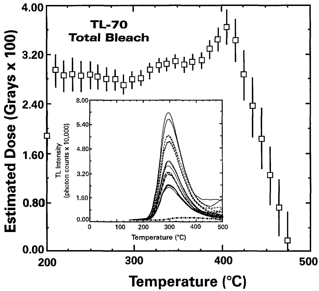
Figure 19: Estimated dose ( D_e ) versus temperature plot for sample TL-70 from IPD. See Figure 7 for details.
