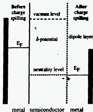
Figure 1: Schematic energy diagrams of a metal-semiconductor interface before charge spilling (the left two panels), showing the relatively high Fermi level of the electrons in the metal film; and after charge spilling (the right two panels), showing the alignment of the Fermi levels and the establishment of a dipole layer.
