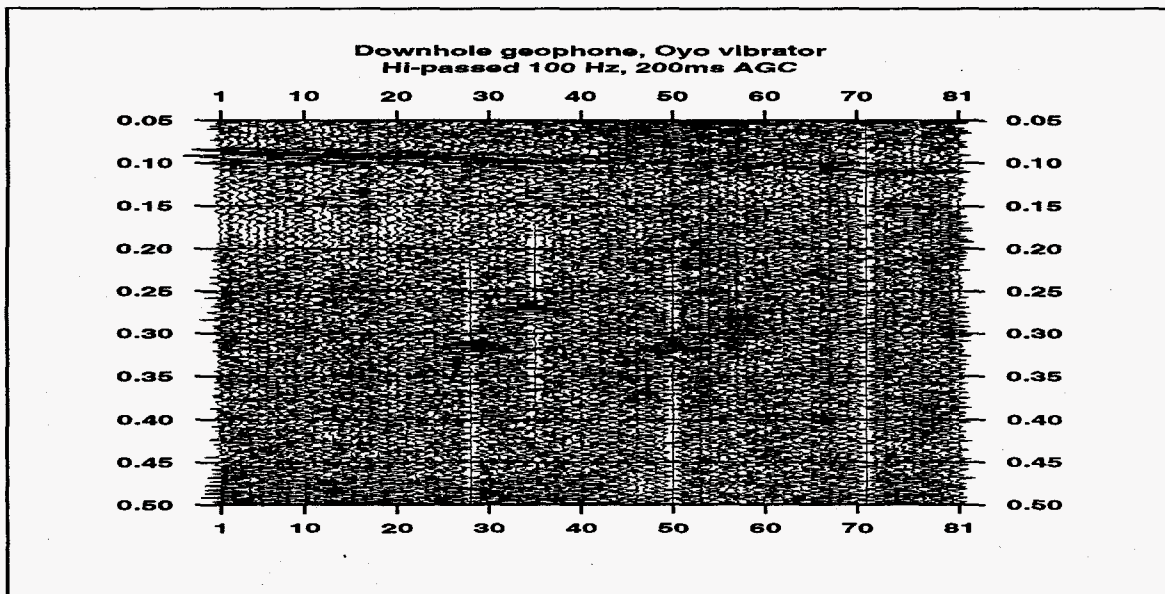
Figure 9d. Oyo portable vibrator shots from all shot stations, recorded by the downhole vertical geophone in well 1943 at the west end of the geophone spread.
