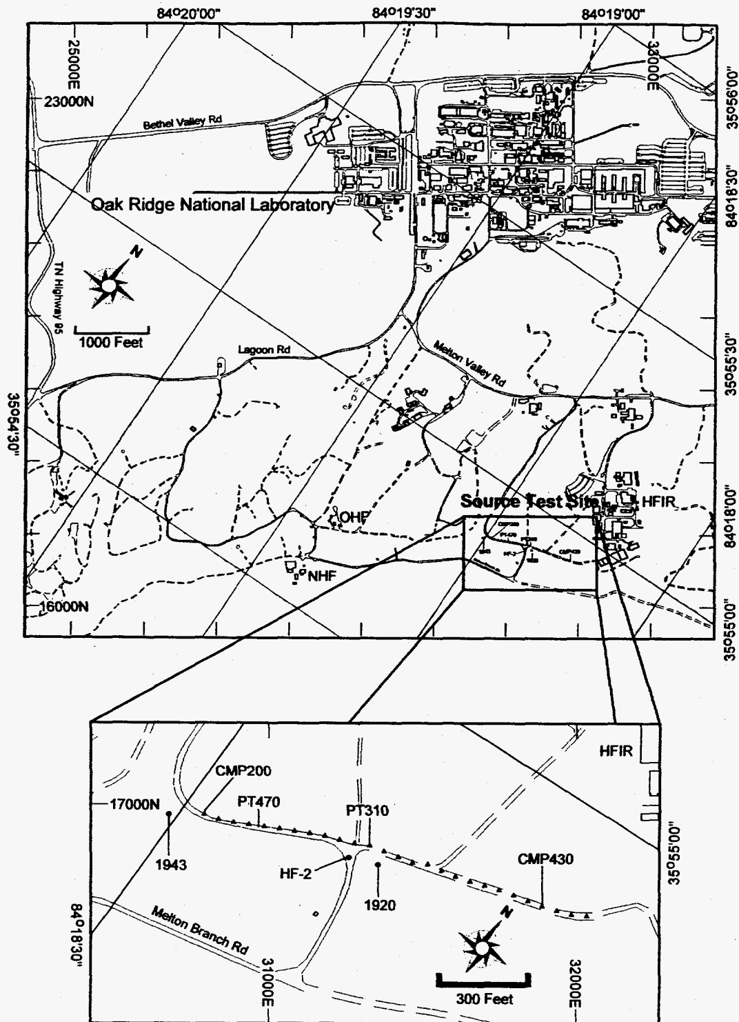
Figure 1. Map view showing the location of the source test site in relation to Oak Ridge National Laboratory. The inset view of the source test site shows locations of geophones and sources (triangles) and wells (circles). The end points of the common midpoint (CMP) and pre-test (PT) profiles are labeled for comparison with subsequent figures.
