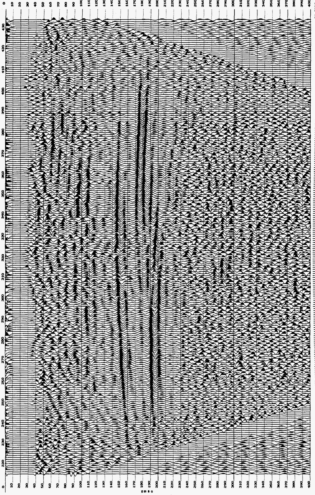
Figure 14a. CMP stacked section for data acquired with the Bison Elastic Wave Generator.
