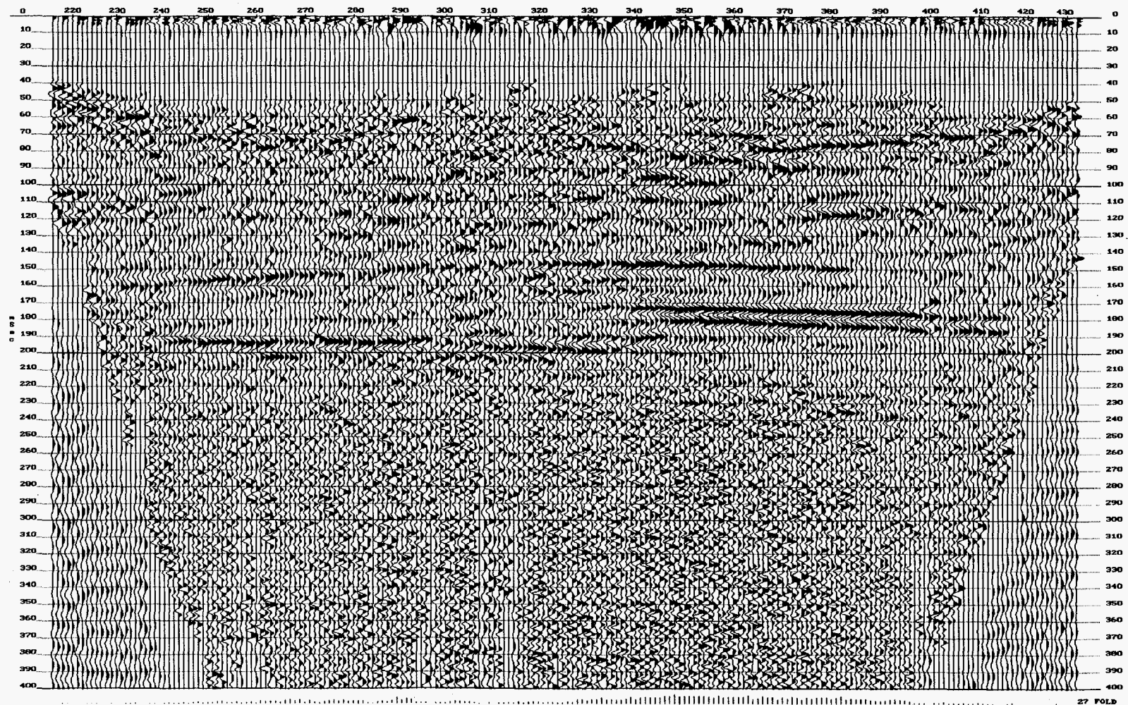
Figure 14b. CMP stacked section for data acquired with the Bison Elastic Wave Generator. Stretch AGC and spiking deconvolution have been applied to the data before stacking.
