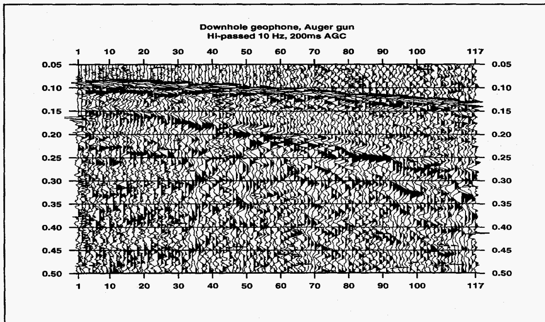
Figure 13d. Auger gun shots from all shot stations, recorded by the downhole vertical geophone in well 1943 at the west end of the geophone spread.
