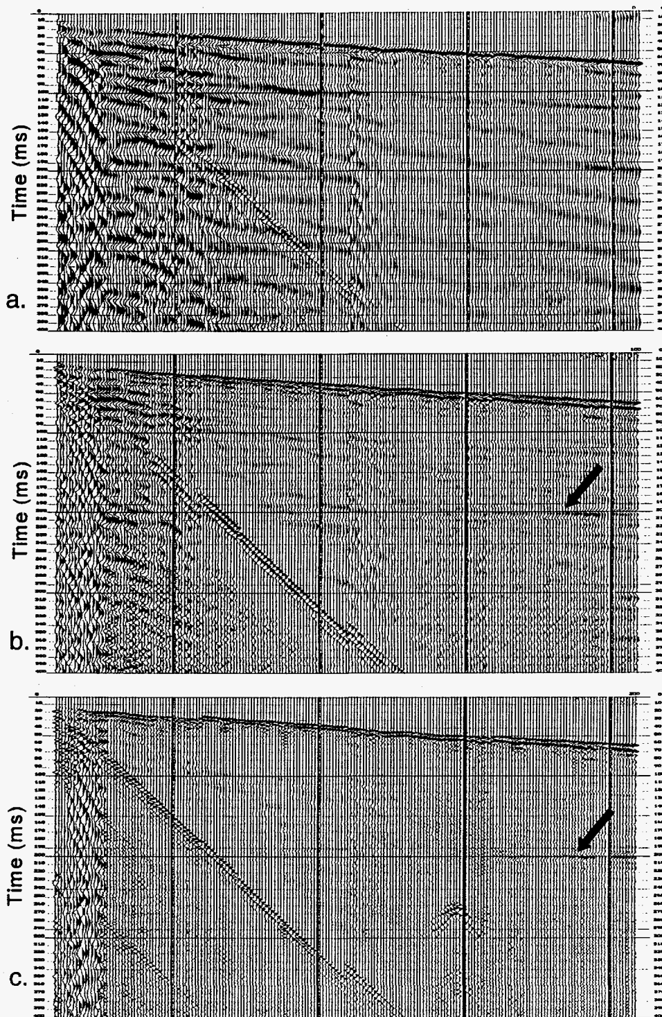
Figure 3. Three shot gathers from the October 1993 pre-test. a) raw data, b) data for the same shot as in a, but high pass filtered at 100 Hz, and c) the same data high pass filtered at 200 Hz. The 200 ms reflection is clearly seen in the filtered data, but not in the raw data. This demonstrates the need to use a source that can generate abundant energy at frequencies greater than 100 Hz.
