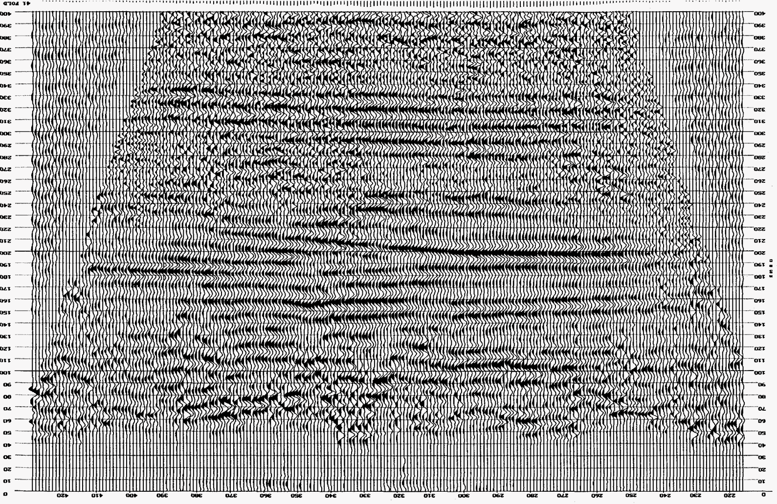
Figure 17a. CMP stacked section for data acquired with the Falling vibrator.
