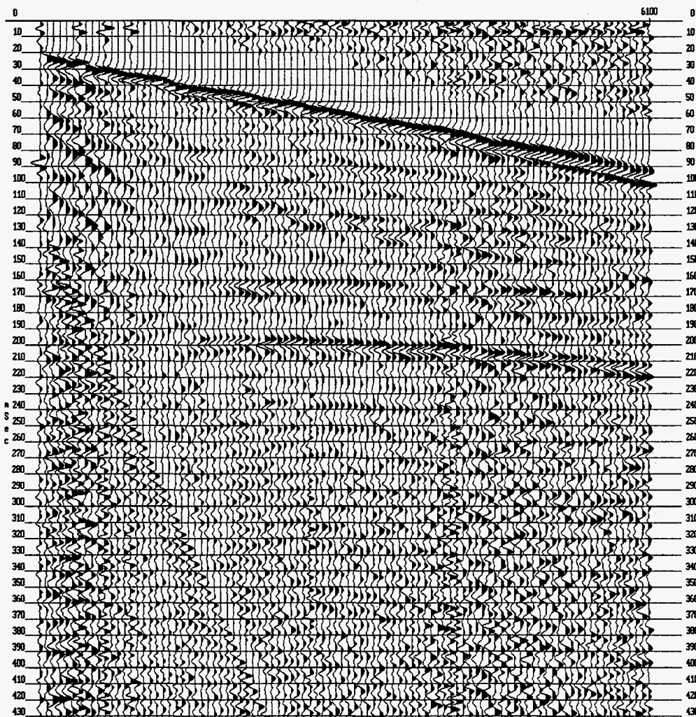
Figure 16b. Shot gather for one shot for the Bolt airgun.
