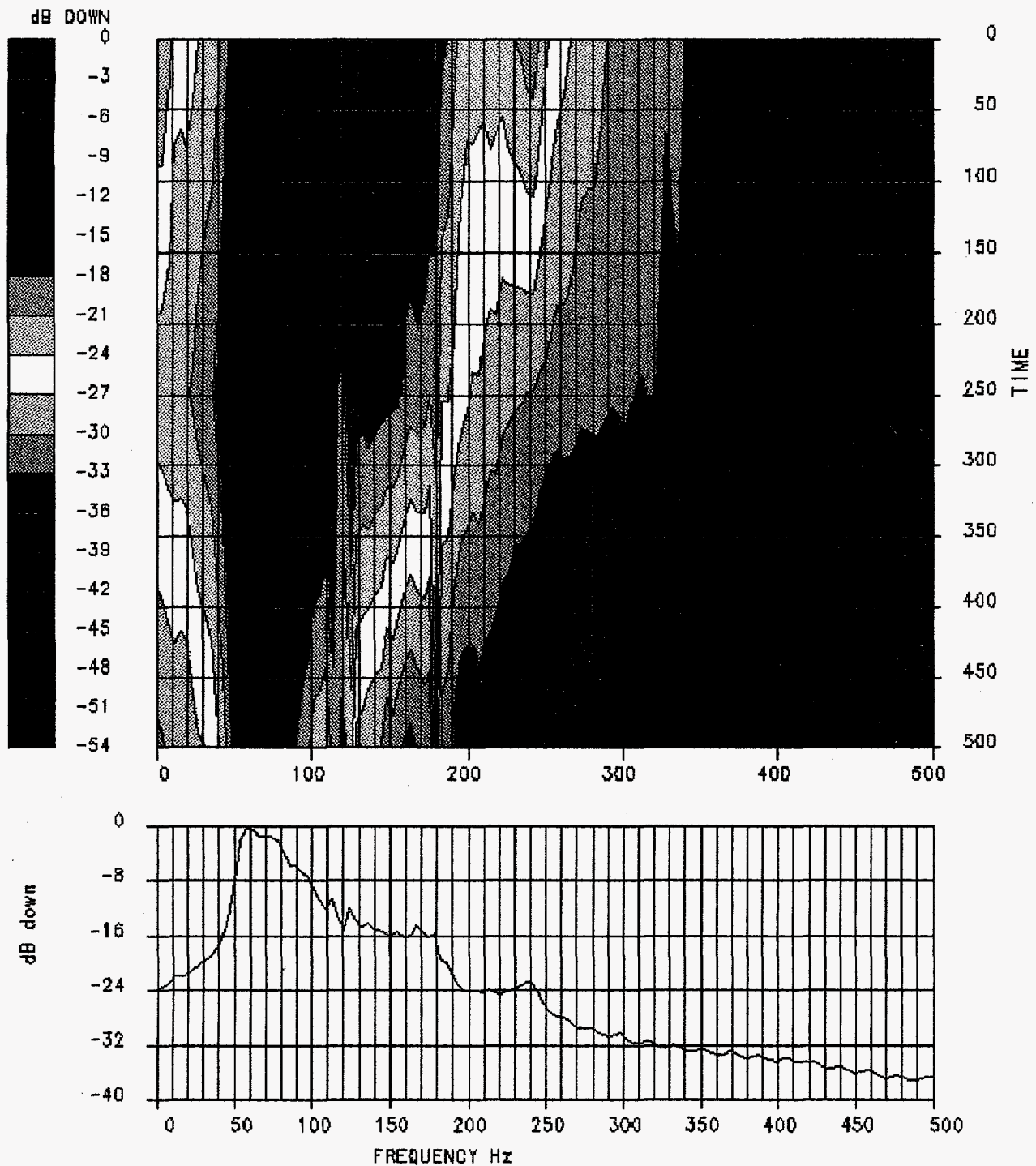
Figure 17g. Spectrum of unfiltered shots recorded by the downhole geophone with the Failing vibrator source. The color display shows how the frequency content varies with time, and an average spectrum for the entire record is shown at the bottom.
