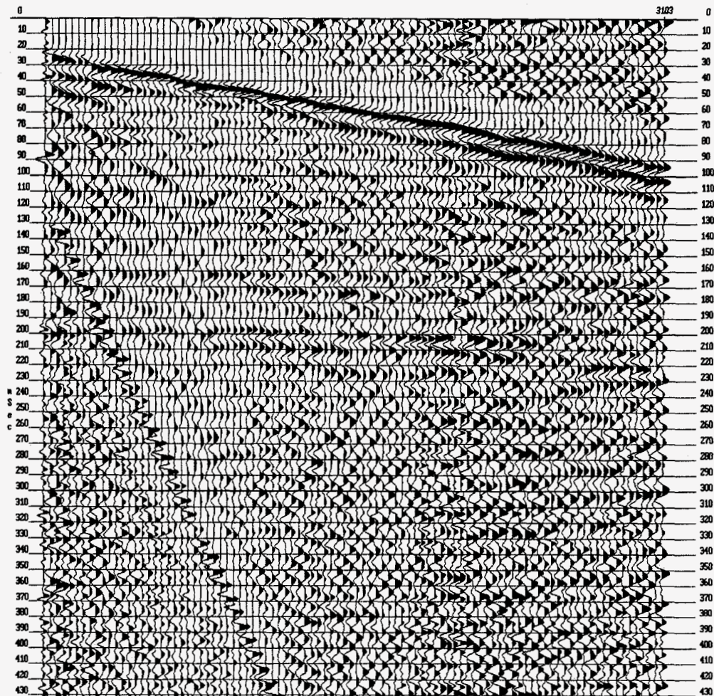
Figure 13b. Shot gather for one shot of the auger gun.
