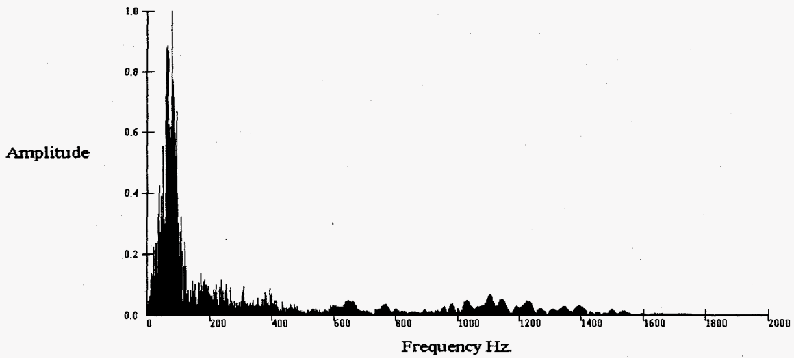
Figure 10c. Spectrum of trace 63, shot 1101 (Fig.10b) for the sledge hammer
