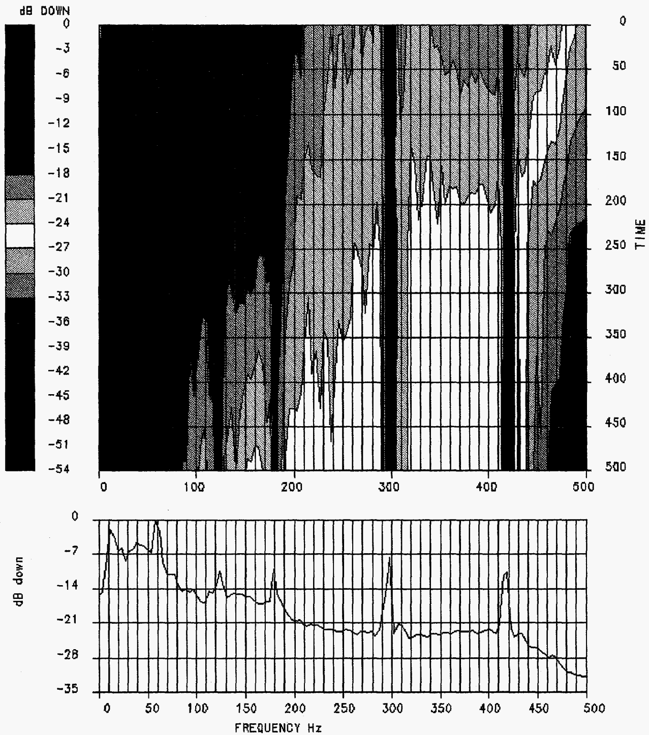
Figure 10e. Spectrum of unfiltered shots recorded by the downhole geophone with the sledge hammer source. The color display shows how the frequency content varies with time, and an average spectrum for the entire record is shown at the bottom.
