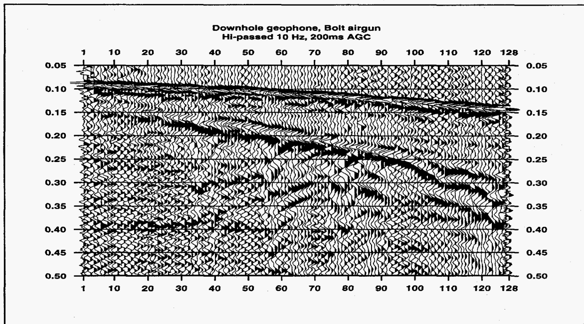
Figure 16d. Airgun shots from all shot stations, recorded by the downhole vertical geophone in well 1943 at the west end of the geophone spread.
