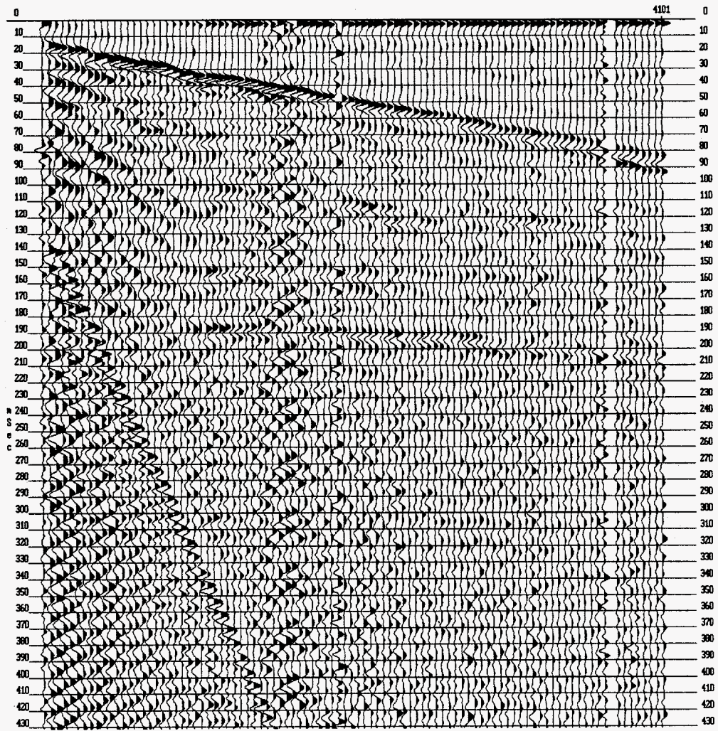
Figure 15d. Shot gather for one shot for the IVI Minivib.
