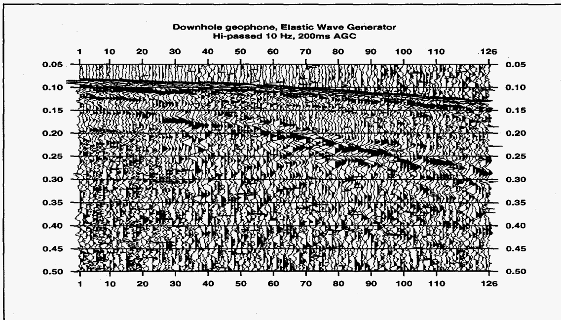
Figure 14e. EWG shots from all shot stations, recorded by the downhole vertical geophone in well 1943 at the west end of the geophone spread.
