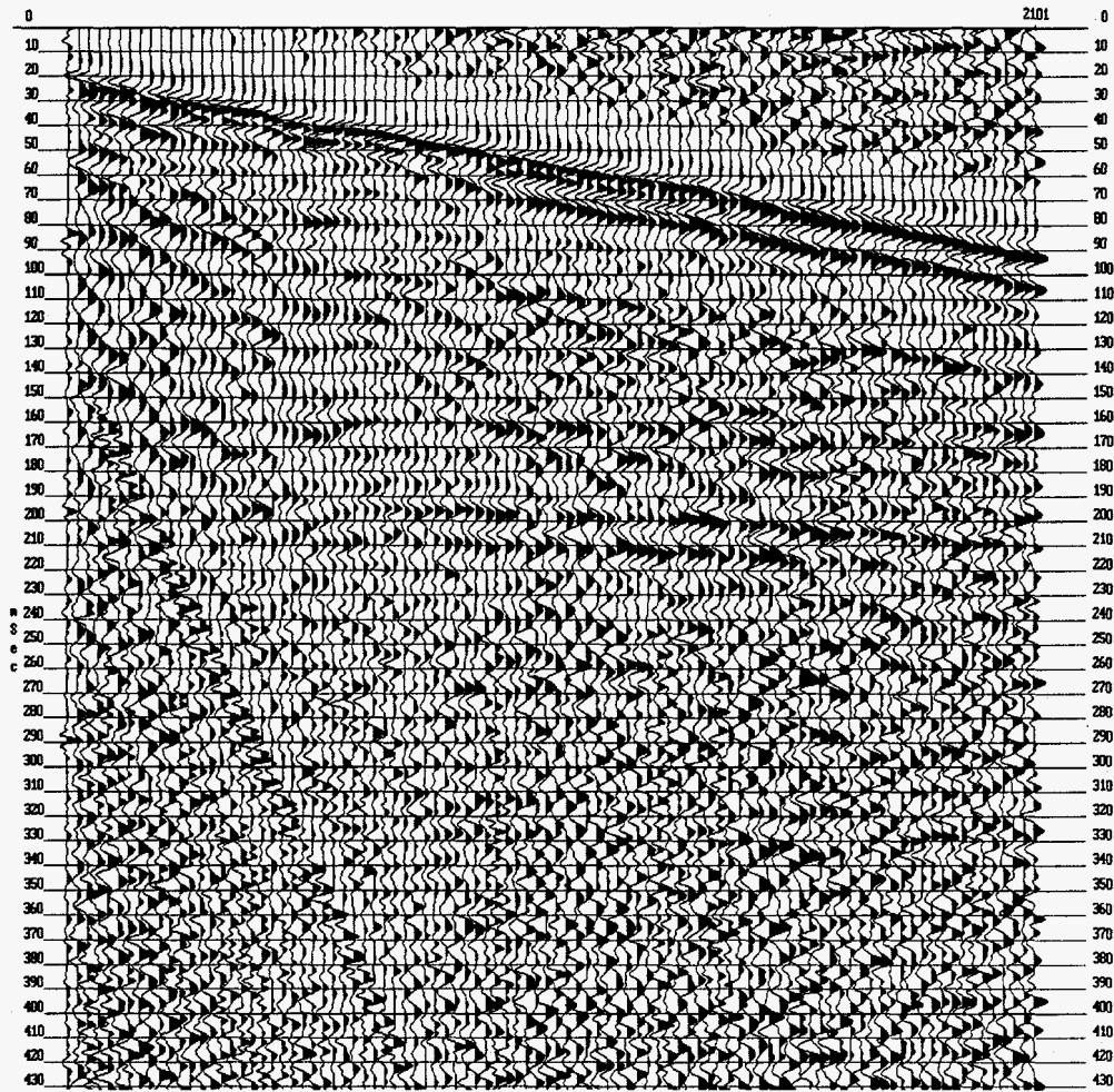
Figure 14c. Shot gather for one shot of the Bison Elastic Wave Generator.
