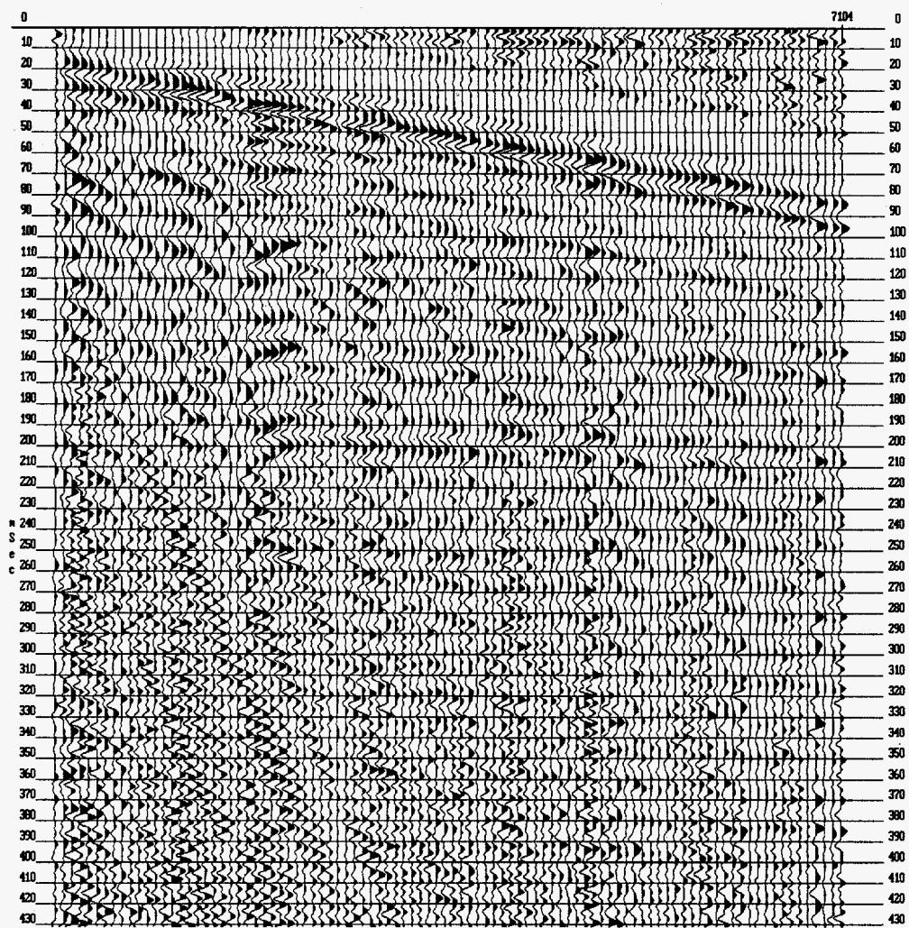
Figure 17d. Shot gather for one shot for the Failing vibrator.
