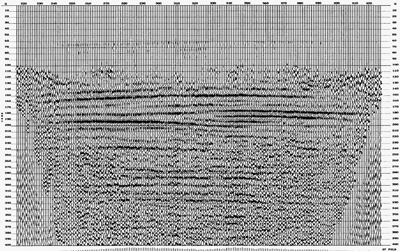
Figure 17b. CMP stacked section for data acquired with the Failing vibrator. Vibroseis whitening has been applied to the data before stacking.
