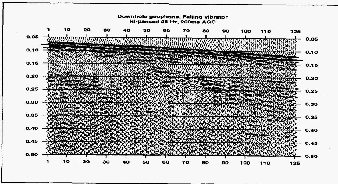
Figure 17f. Failing vibrator shots from all shot stations, recorded by the downhole vertical geophone in well 1943 at the west end of the geophone spread.
