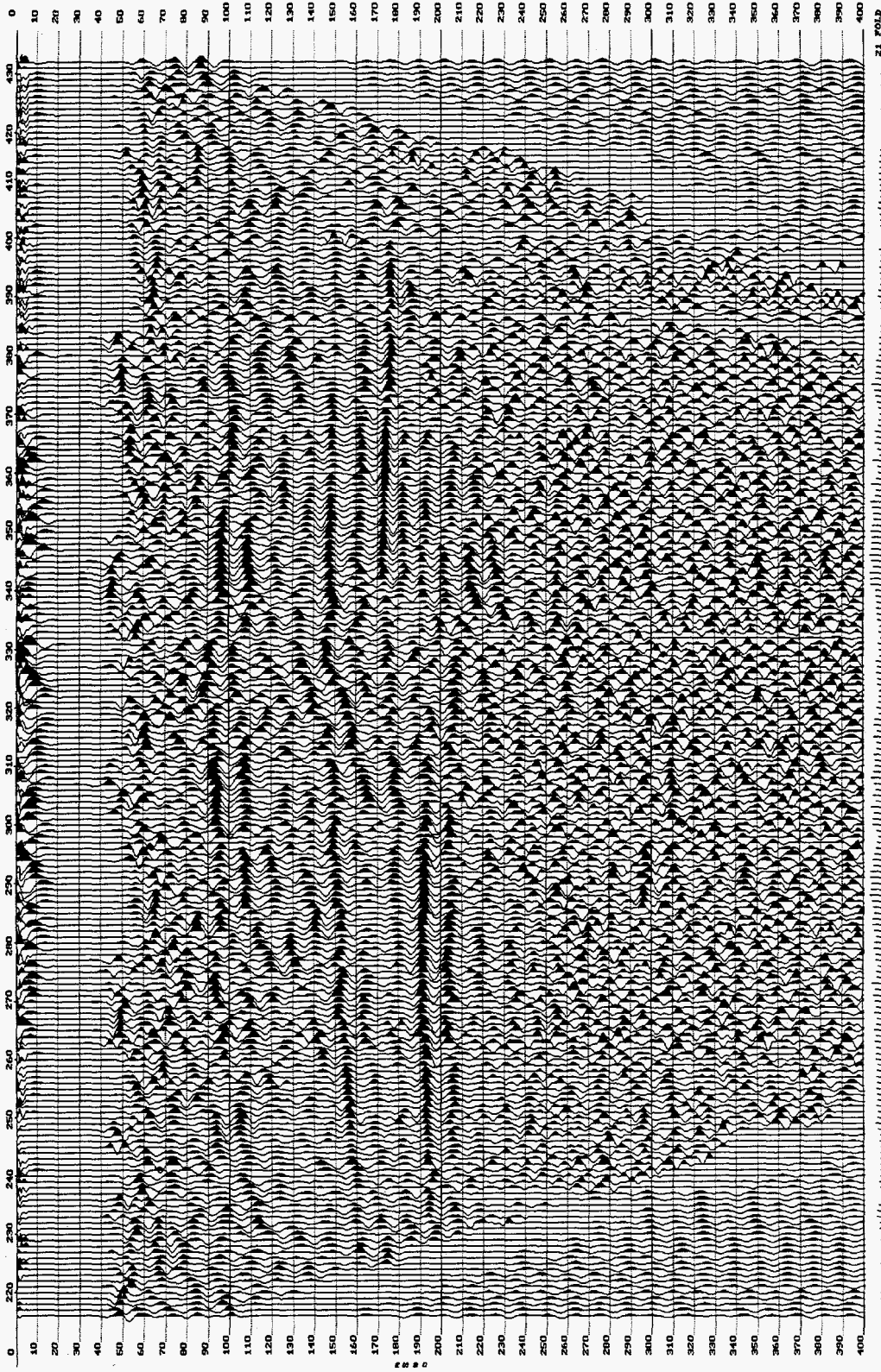
Figure 10a. CMP stacked section for data acquired with the 16 lb. sledge hammer.
