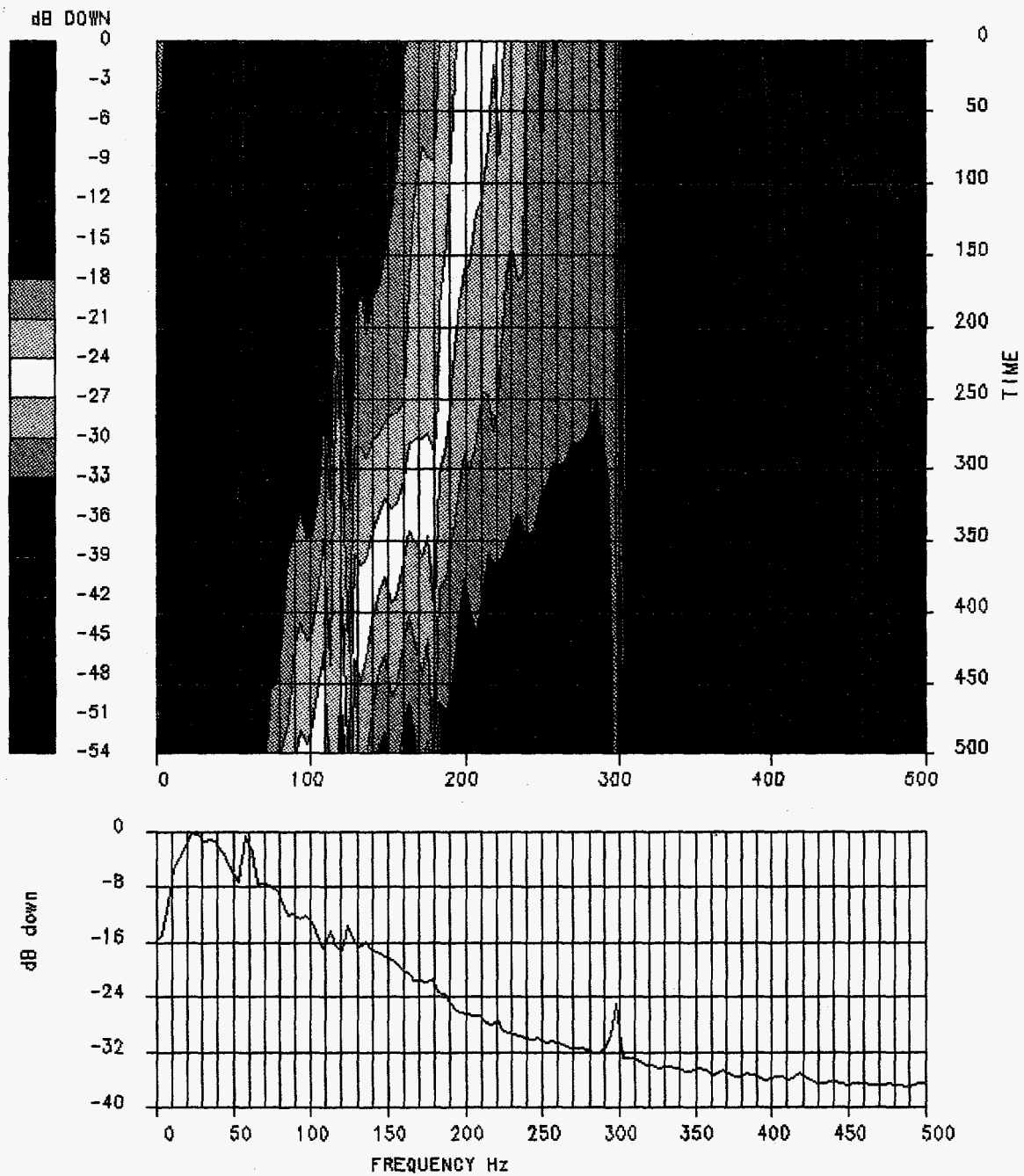
Figure 13e. Spectrum of unfiltered shots recorded by the downhole geophone with the auger gun source. The color display shows how the frequency content varies with time, and an average spectrum for the entire record is shown at the bottom.
