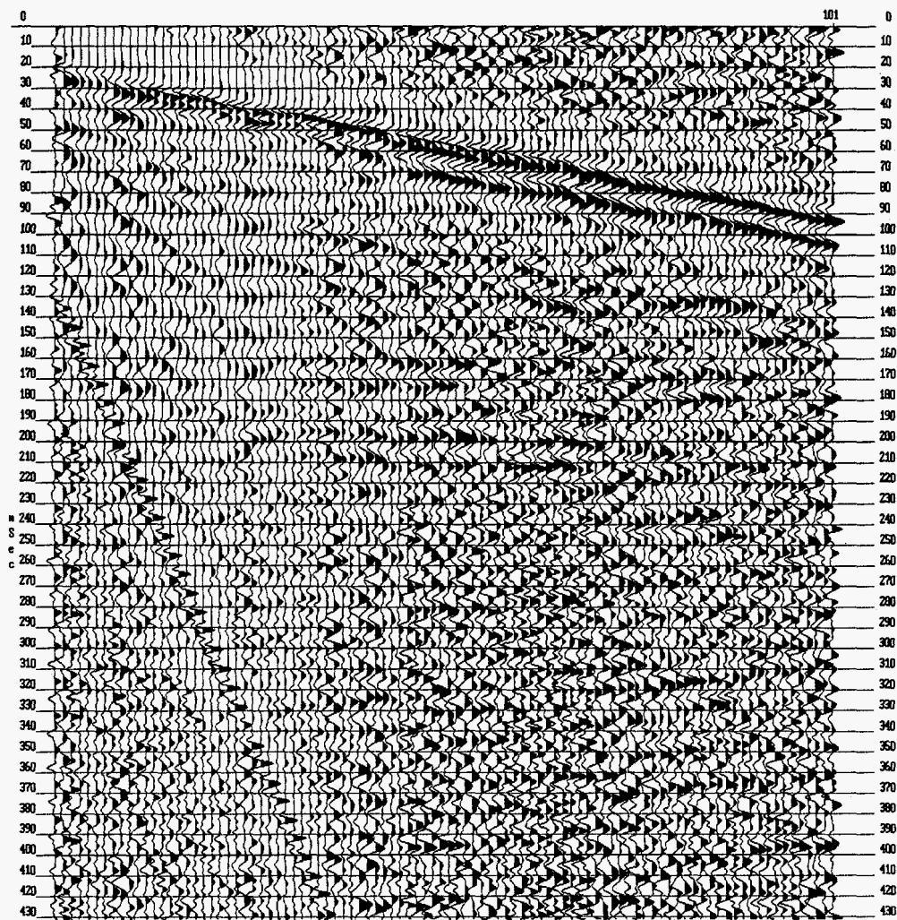
Figure 10b. Shot gather for one shot for the sledge hammer.
