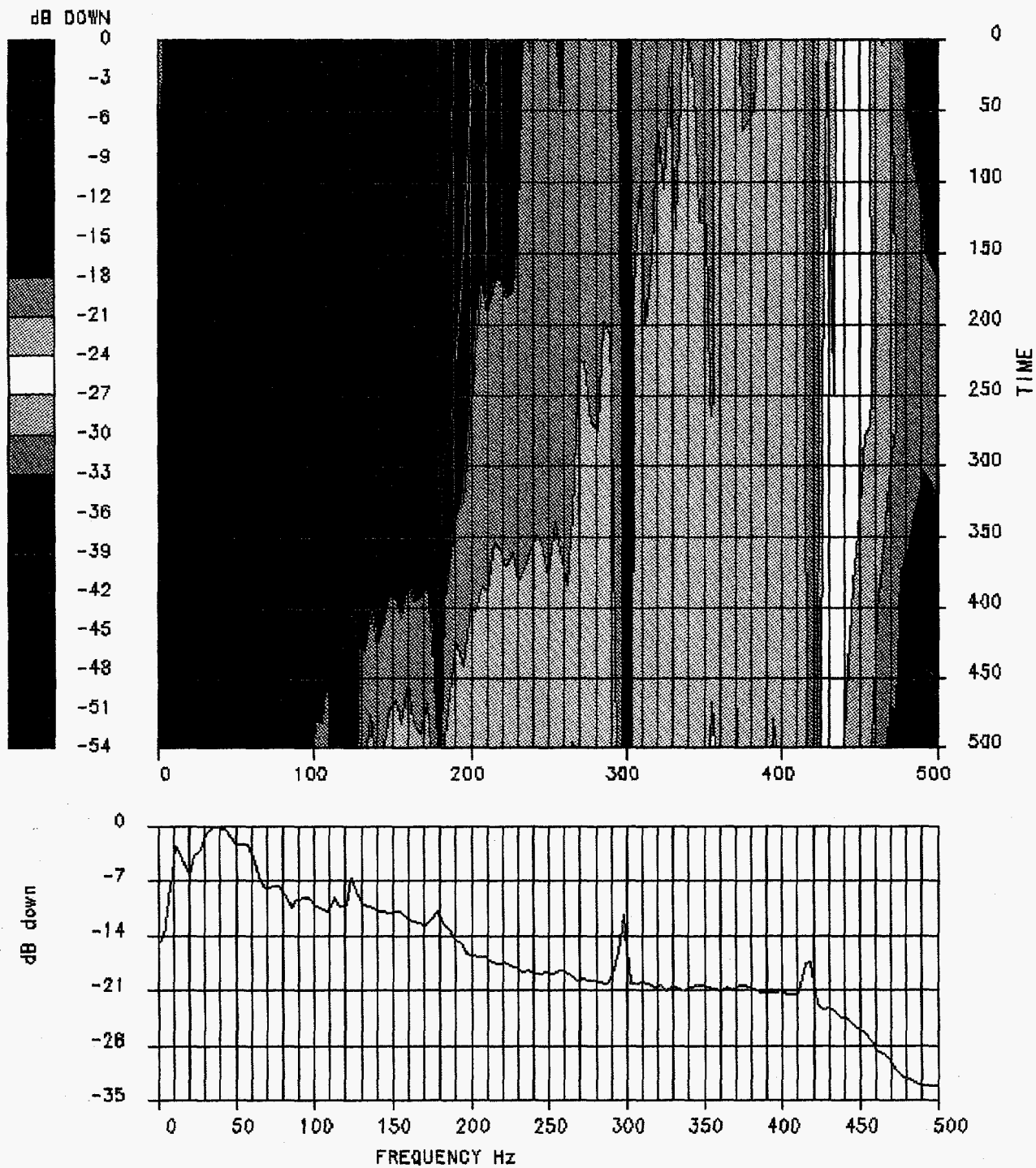
Figure 14f. Spectrum of unfiltered shots recorded by the downhole geophone with the EWG source. The color display shows how the frequency content varies with time, and an average spectrum for the entire record is shown at the bottom.
