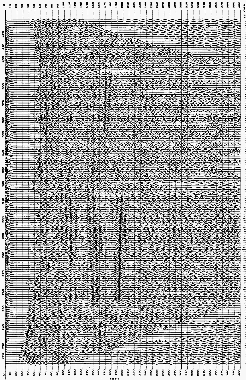
Figure 9a. CMP stacked section for data acquired with the Oyo portable vibrator.
