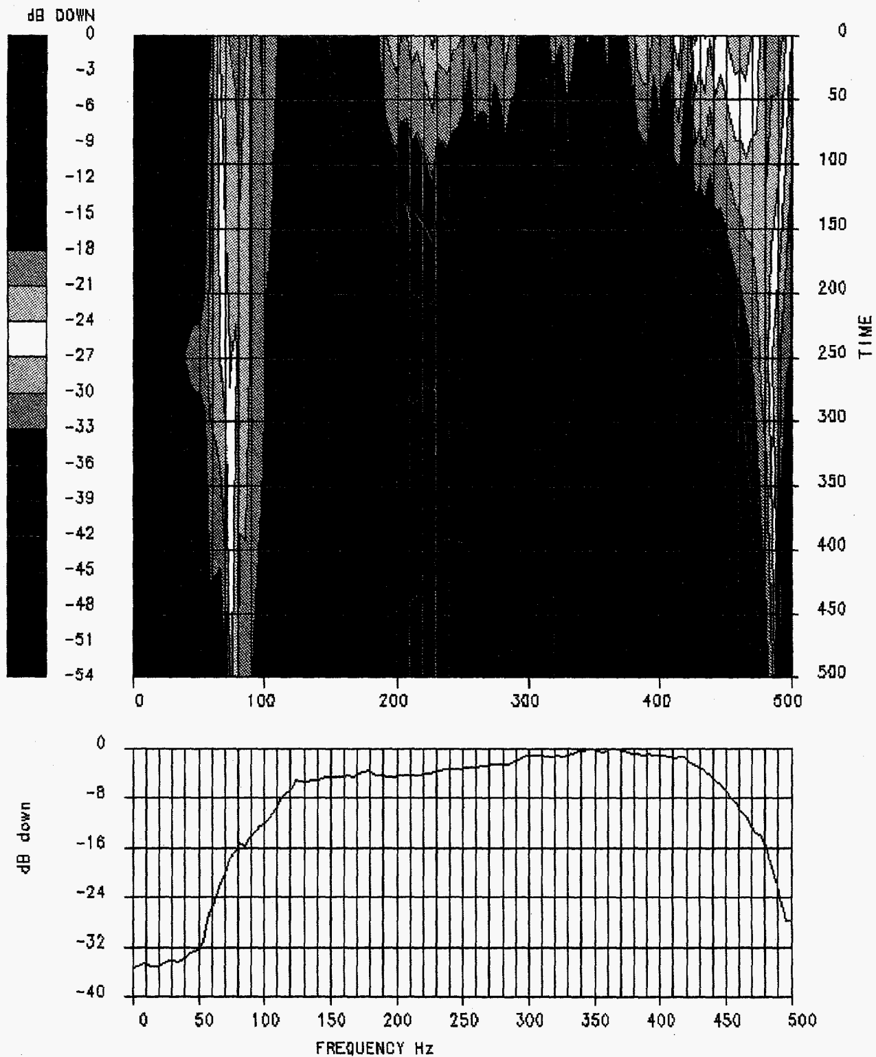
Figure 9e. Spectrum of Oyo downhole geophone data after applying a 50/100 high pass filter to the data.
