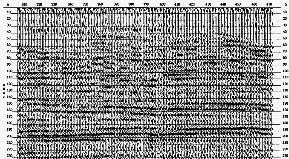
Figure 2. Brute common midpoint stack of seismic reflection data acquired during the October 1993 pre-test with an auger gun source between stations PT310 and PT470 (Figure 1).
