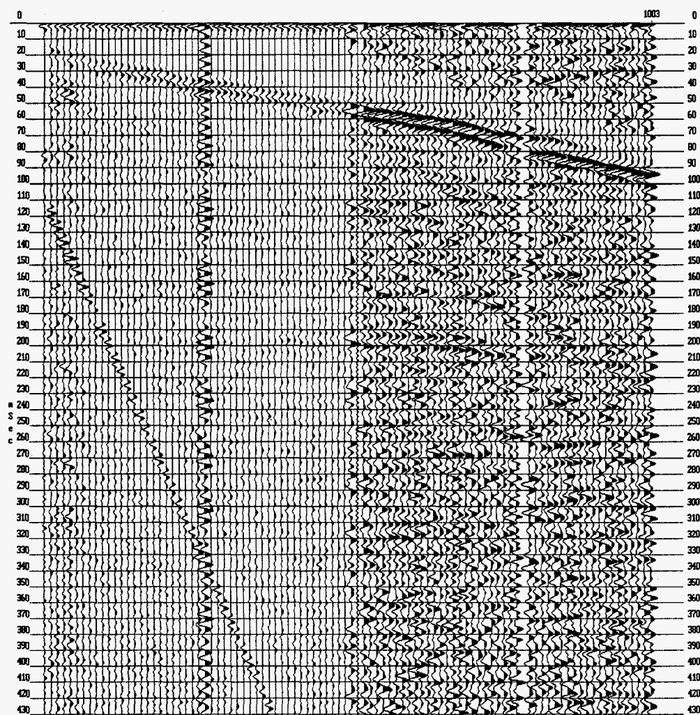
Figure 9b. Shot gather for one shot for the Oyo portable vibrator. The first 48 channels were recorded at lower gain by the Oyo representative to avoid clipping.
