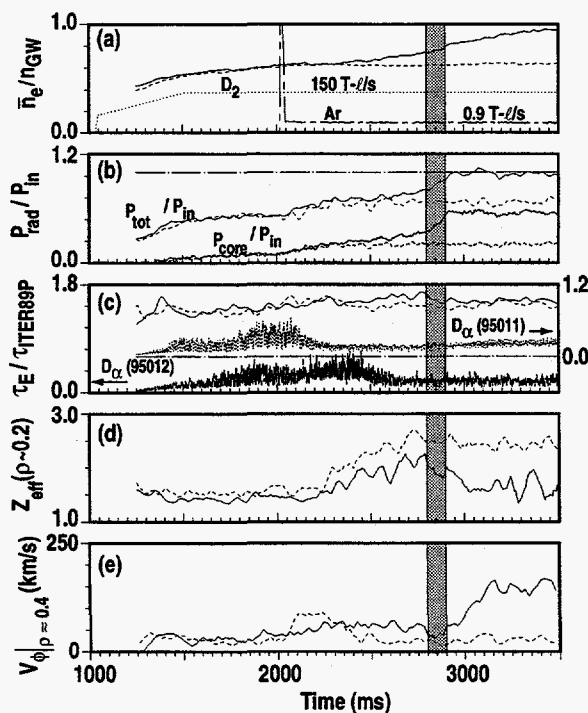
Fig. 4. Comparison of two similar discharges, one which transitions into a radiating mantle (#95011, solid) and one which has primarily divertor radiation (#95012, dash). The transition region is shown by the shaded area. The calculation of core Z_{\text{eff}} is discussed in Section 2. Deuterium and argon gas puffing rates are the same for both discharges. Discharge conditions are: 1.3 MA, 2.1 T, lower single-null divertor with pumping.
