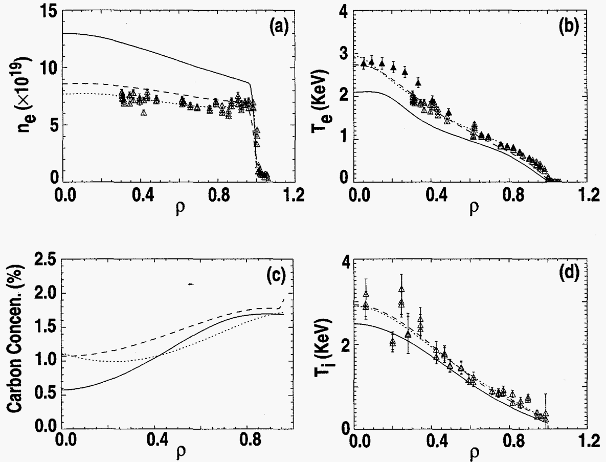
Fig. 6. Profiles during the evolution of the radiating mantle discharge (#95011) at 3 times: 2240 ms (dots), 2700 ms, just before the transition (dashed), and 3400 ms (solid). For clarity, data points are only shown for the fit at 2240 ms. (a) Electron density is measured by Thomson scattering, (b) T_e is determined from fits to Thomson scattering and 3rd harmonic ECE measurements. The carbon impurity fraction (c) and T_i (d) are measured by CER.
