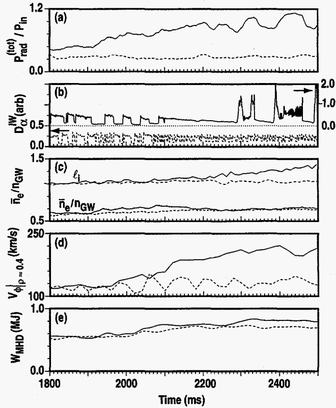
Fig. 2. Comparison of a discharge with impurity injection (#95758, solid) to a similar discharge with no impurity puff (#95756, dashed). Stored energy, W_{MHD} , and \ell_i are calculated from EFIT equilibria including motional Stark effect measurements and toroidal rotation is measured by charge exchange recombination of a visible CVI line.
