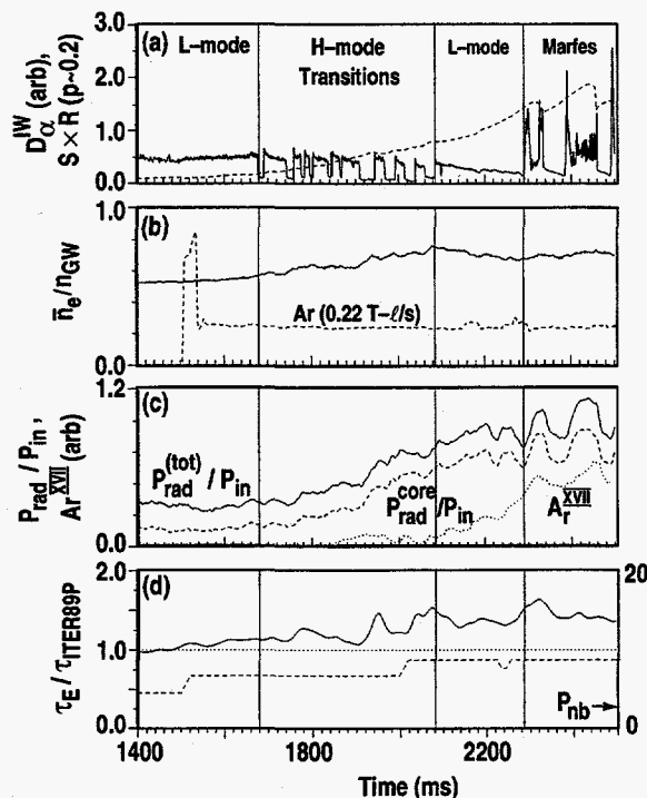
Fig. 1. Time evolution leading to the radiating mantle phase of a inner wall limited discharge in DIII-D: (a) Inner wall D_{\alpha} intensity and central soft X-ray emission, (b) normalized density, n_e/n_{GW} and argon impurity flow (there was no deuterium puffing during the time shown), (c) radiation fractions and Ar XVII line intensity which was the dominant charge state, and (d) H factor and neutral beam power. Discharge conditions (#95758): 1.3 MA, 1.8 T, K \approx 1.5 .
