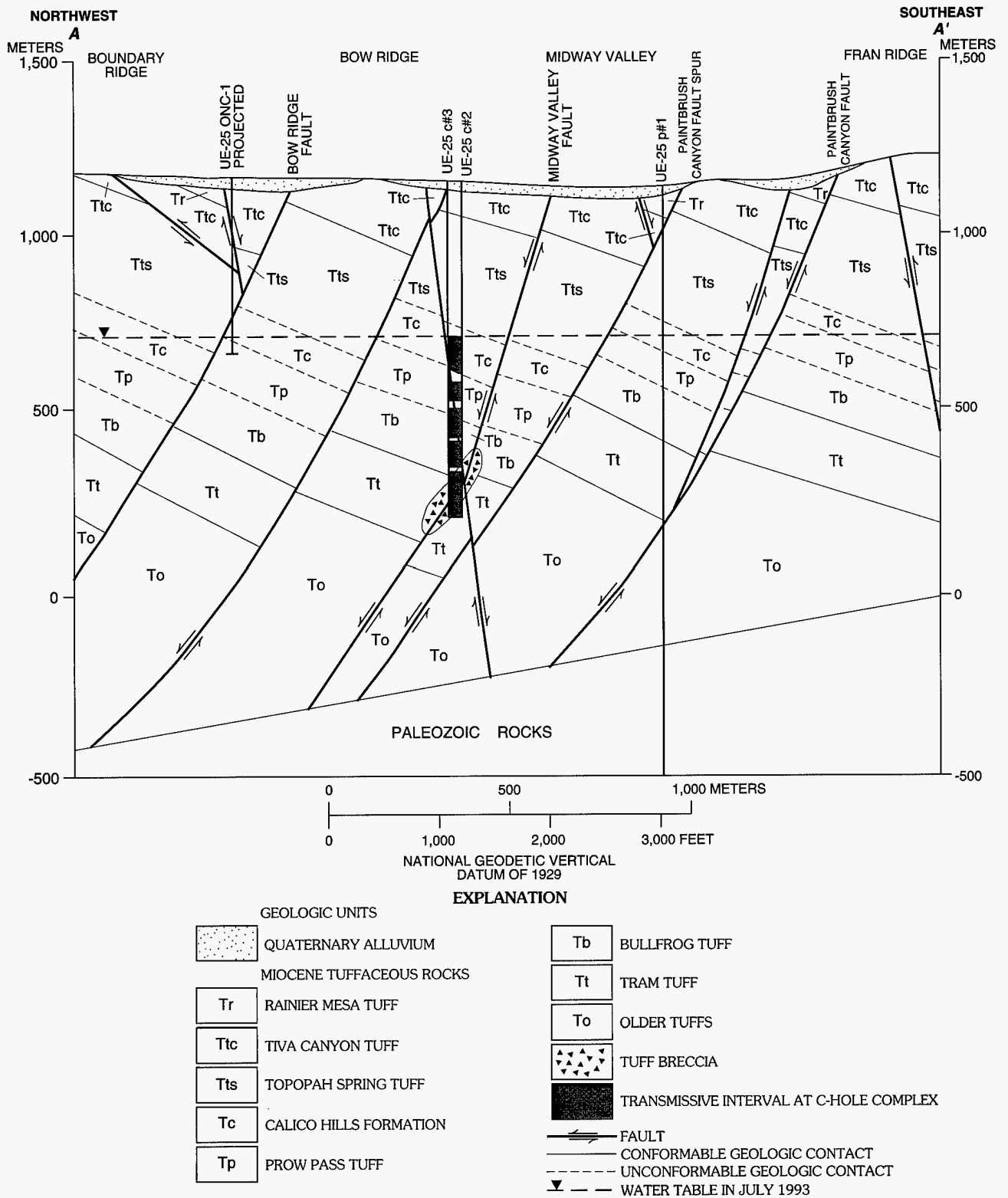
Figure 3. Hydrogeologic section from Boundary Ridge to Fran Ridge (location of section shown in figure 2).
