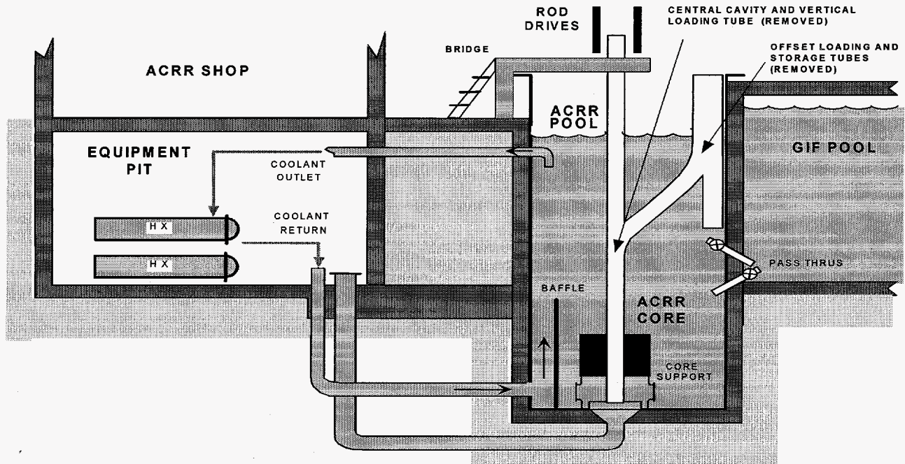
Figure 2. Cutaway View of the ACRR.
