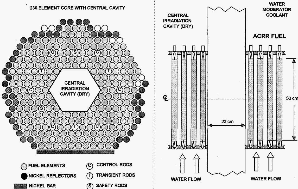
Figure 3A: Core Configuration for DOE DP Programs.
