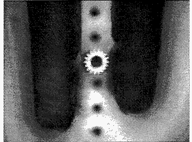
Figure 2. LIGA tweezers placing a LIGA gear on a 44 micron OD shaft.
