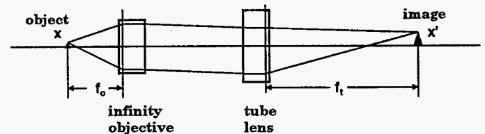
Figure 3. Infinity corrected microscope optics.
