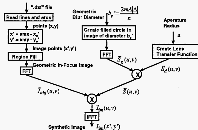
Figure 5. Block Diagram of synthetic image generation.
