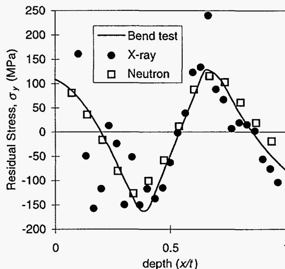
Figure 1. Measured and known residual stress profiles.
