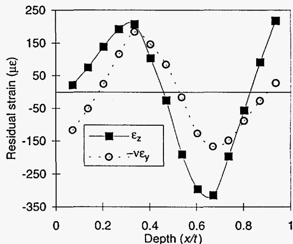
Figure 3. Measured transverse strains compared to plane stress assumption.
