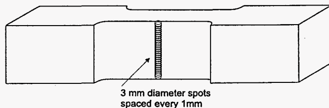
Figure 4. Measuring residual stress profile using overlapping x-ray measurements.
