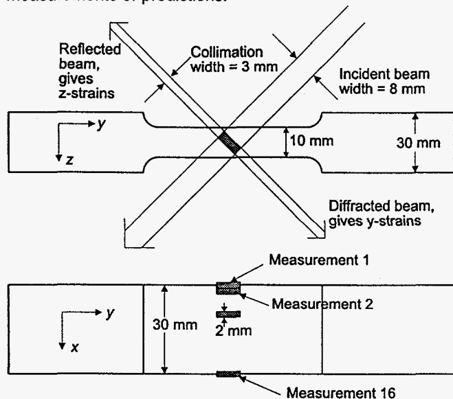
Figure 2. Measuring residual stress profile \sigma_y(x) using neutron powder diffraction.
