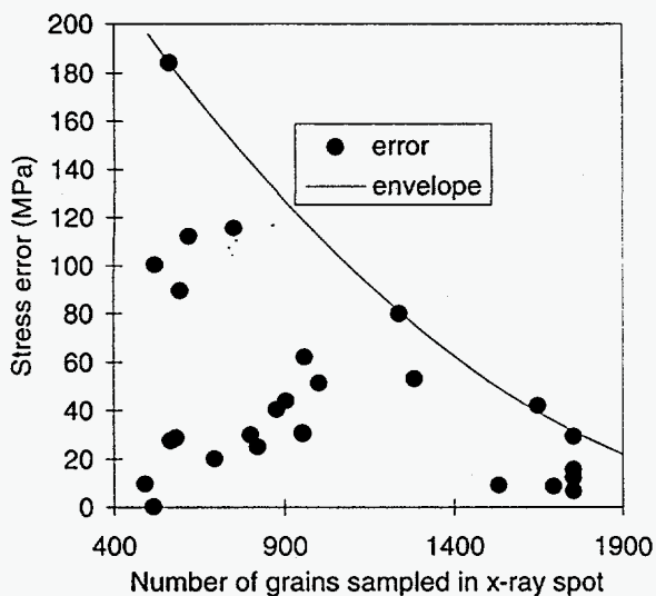
Figure 5. Error in x-ray stress measurements correlated to grain size variations.
