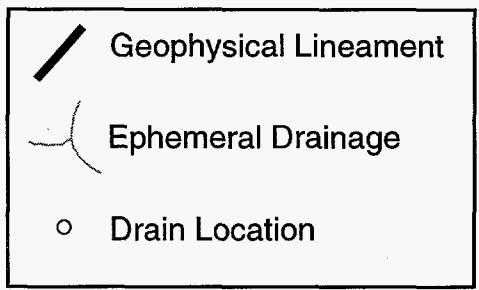
FIGURE 2 Drain Distributions in the Vicinity of the Lautertal and Groundwater Flow Vector Results of the Calibrated Model
