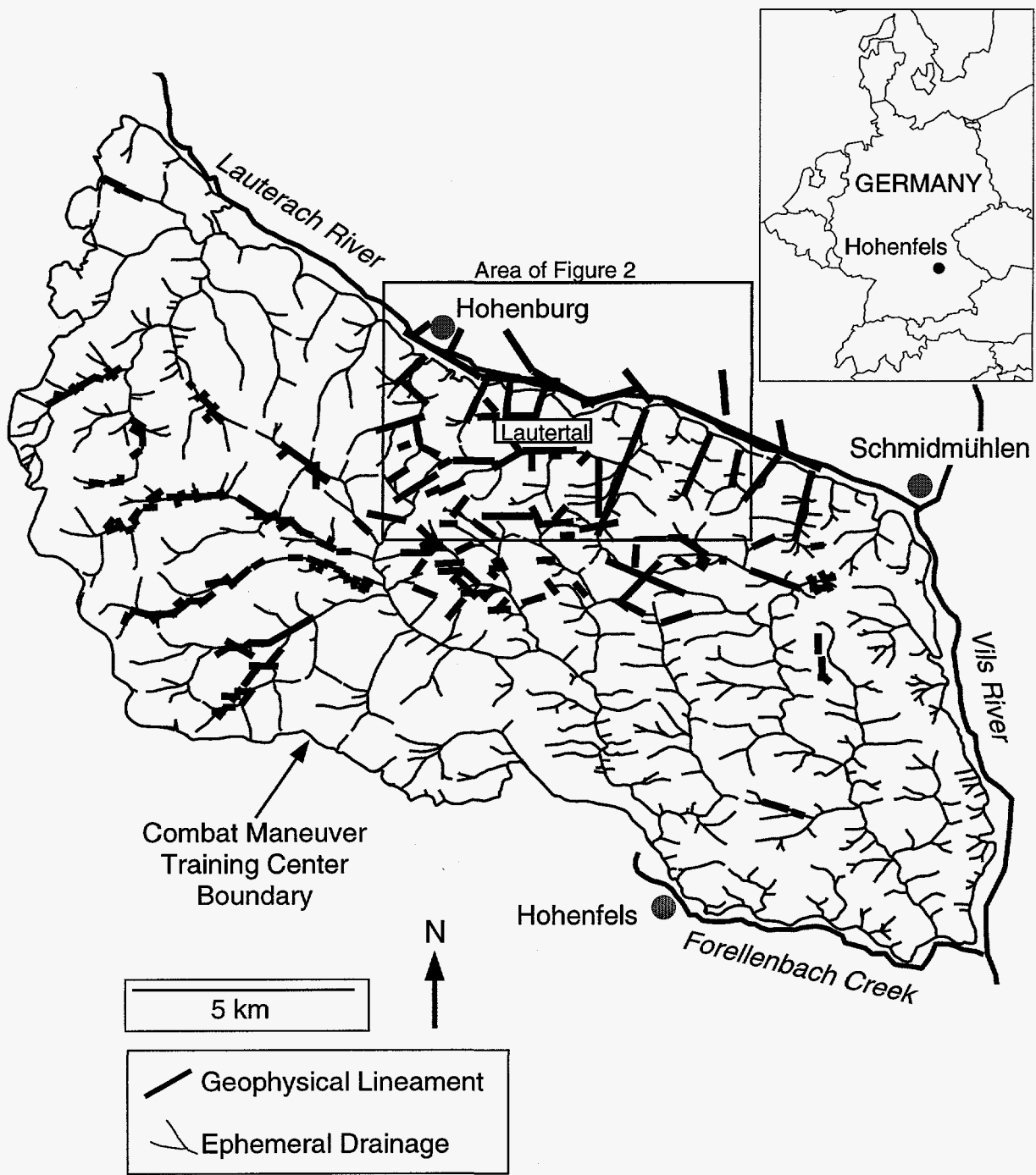
FIGURE 1 Location of the Lautertal Study Area, Geophysical Lineament Results, and On-Base Ephemeral Drainages
