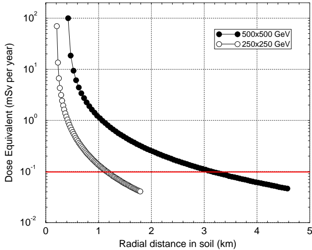
Figure 7: Maximum dose equivalent in TEP embedded in soil in low-energy muon collider orbit plane with 2 \times 10^{20} decays per year vs distance from ring center.
