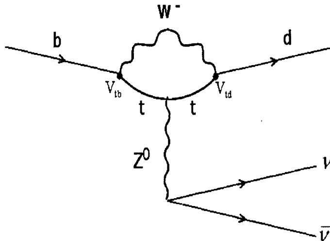
FIGURE 6. The Feynman diagram for the rare B decay B \rightarrow X_d \nu \bar{\nu} , which is analogous to the neutrino process of figure 5.
