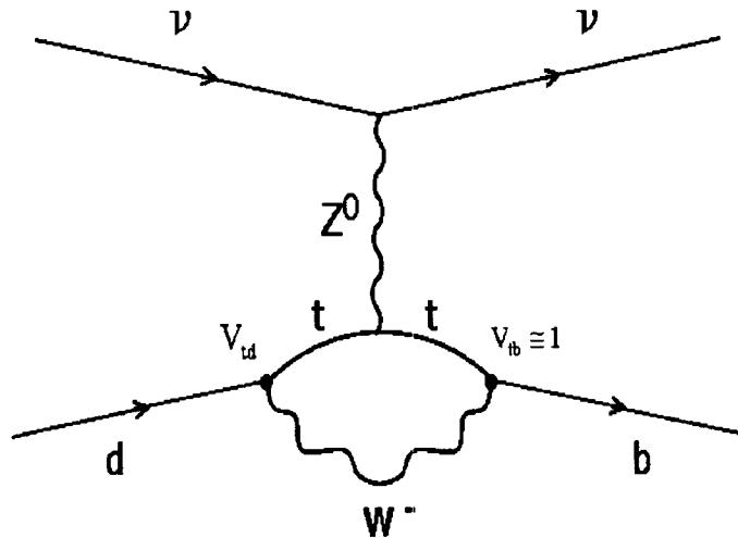
FIGURE 5. The Feynman diagram for B production through a flavor changing neutral current interaction involving a top quark loop.
