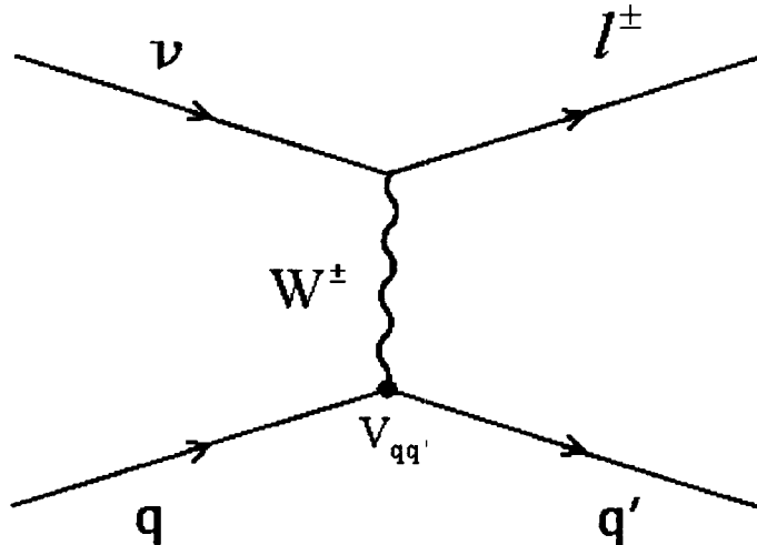
FIGURE 4. The Feynman diagram for charged current neutrino-quark scattering, showing that the CKM matrix element V_{qq'} participates as an amplitude in the W -quark vertex.
