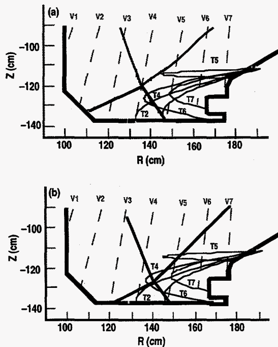
Fig. 1. Vertical views (V1-V7) and tangential views (T2, T4-T7) for obtaining the BII data employed in the present analysis. (a) separatrix configuration at 3.0 s. (b) separatrix configuration at 4.4 s.
