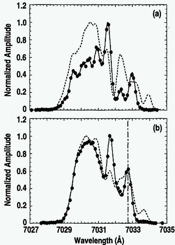
Fig. 2. Profiles of the B II ( ^3P-^3S ) transition observed along views V2 (a) and V6 (b). Solid circles are measured data; solid lines are the best fit theoretical profiles using the Zeeman/Paschen-Back effect; dotted lines are theoretical profiles if only the low-field linear approximation (Zeeman effect) is employed.
